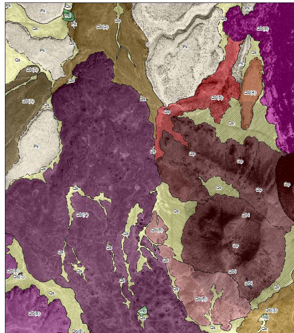
Figure 1. Geologic map of the V7504 field area, San Francisco Volcanic Field, north-central AZ. A chief question of the field mapping was the nature and evolution of the V7504 vent complex, identified here in brown.
