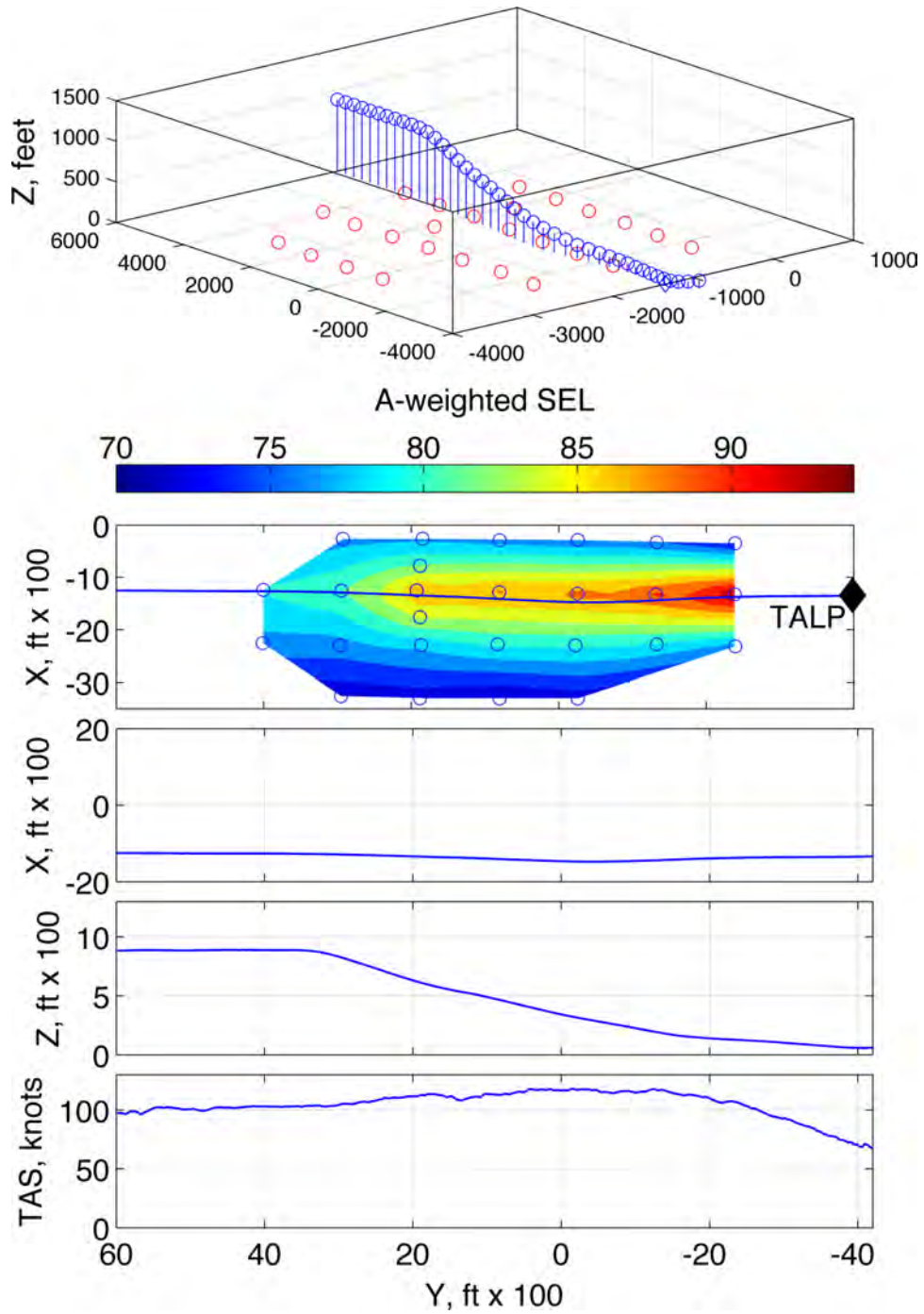
Figure 355: Terminal area condition T9A, segmented 100 - 110 KIAS, -9^\circ , 110 - 90 KIAS, -7.5^\circ , 90 - 0 KIAS, -4^\circ , run number 288631
