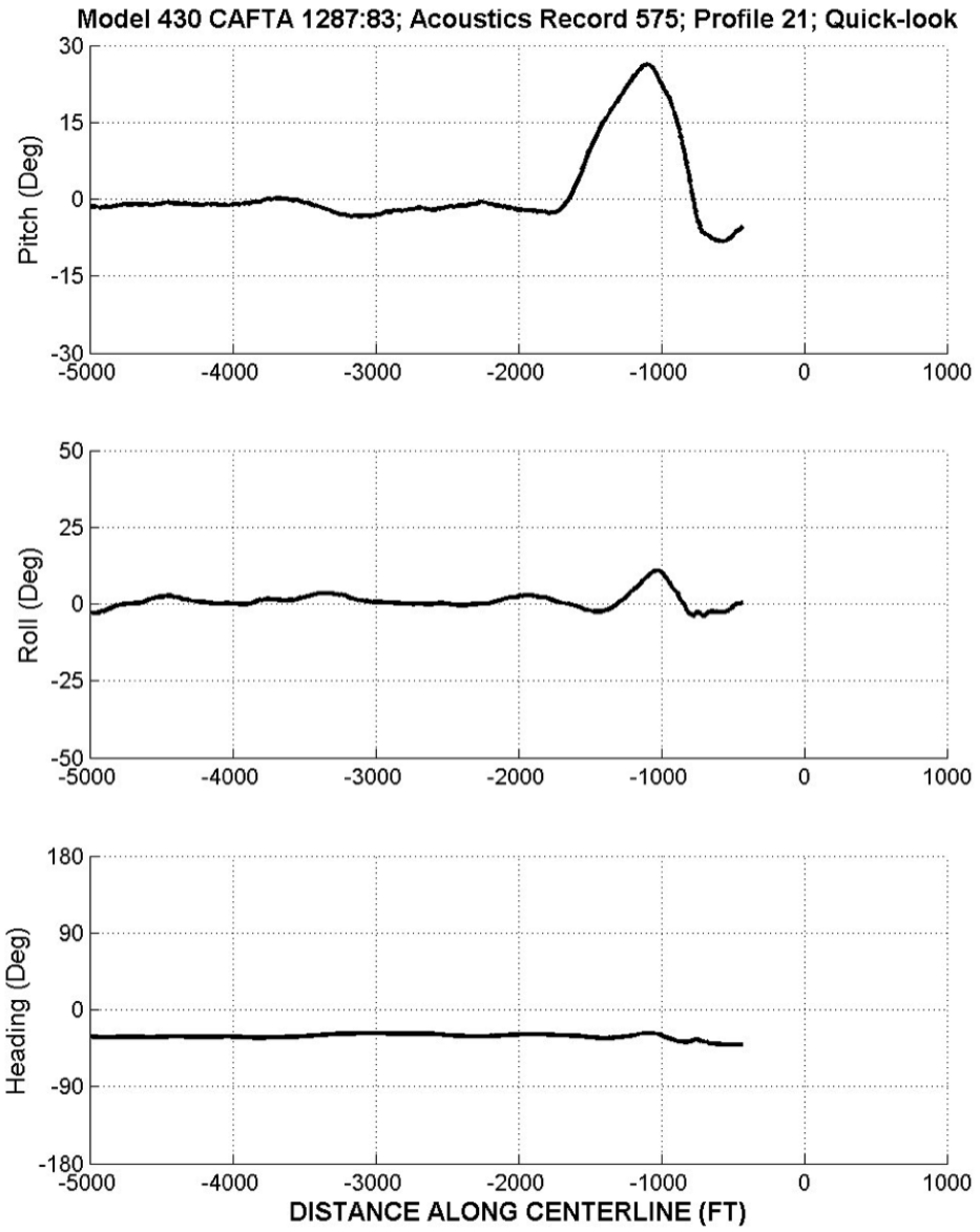
Figure 12: Quick-look aircraft control attitudes.
