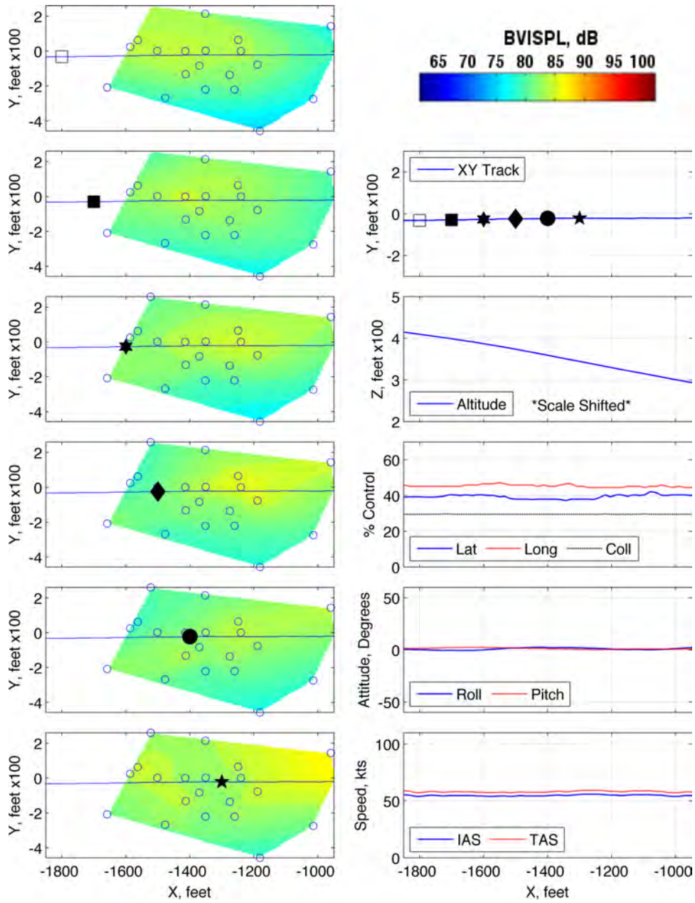
Figure 102: Maneuver condition A6, 60 KIAS, -6^\circ , run number 282446
