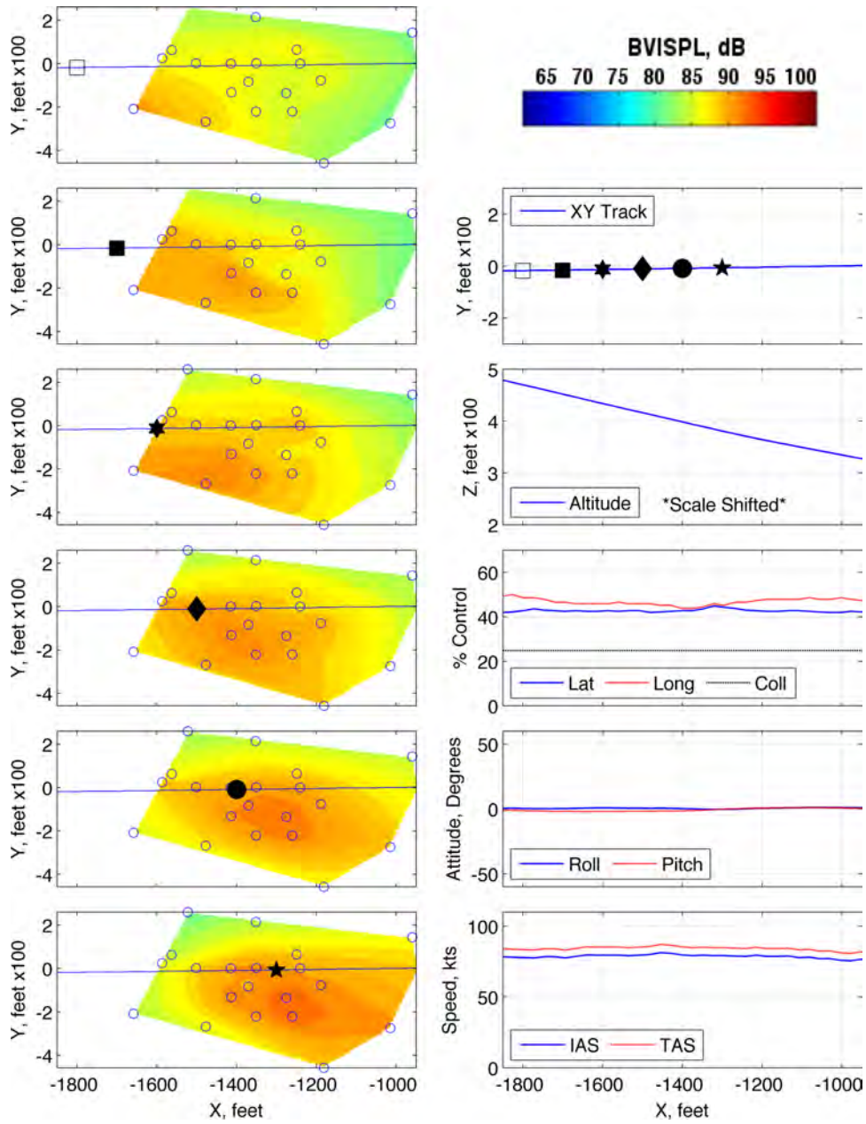
Figure 115: Maneuver condition A22, 80 KIAS, -9^\circ , run number 282445
