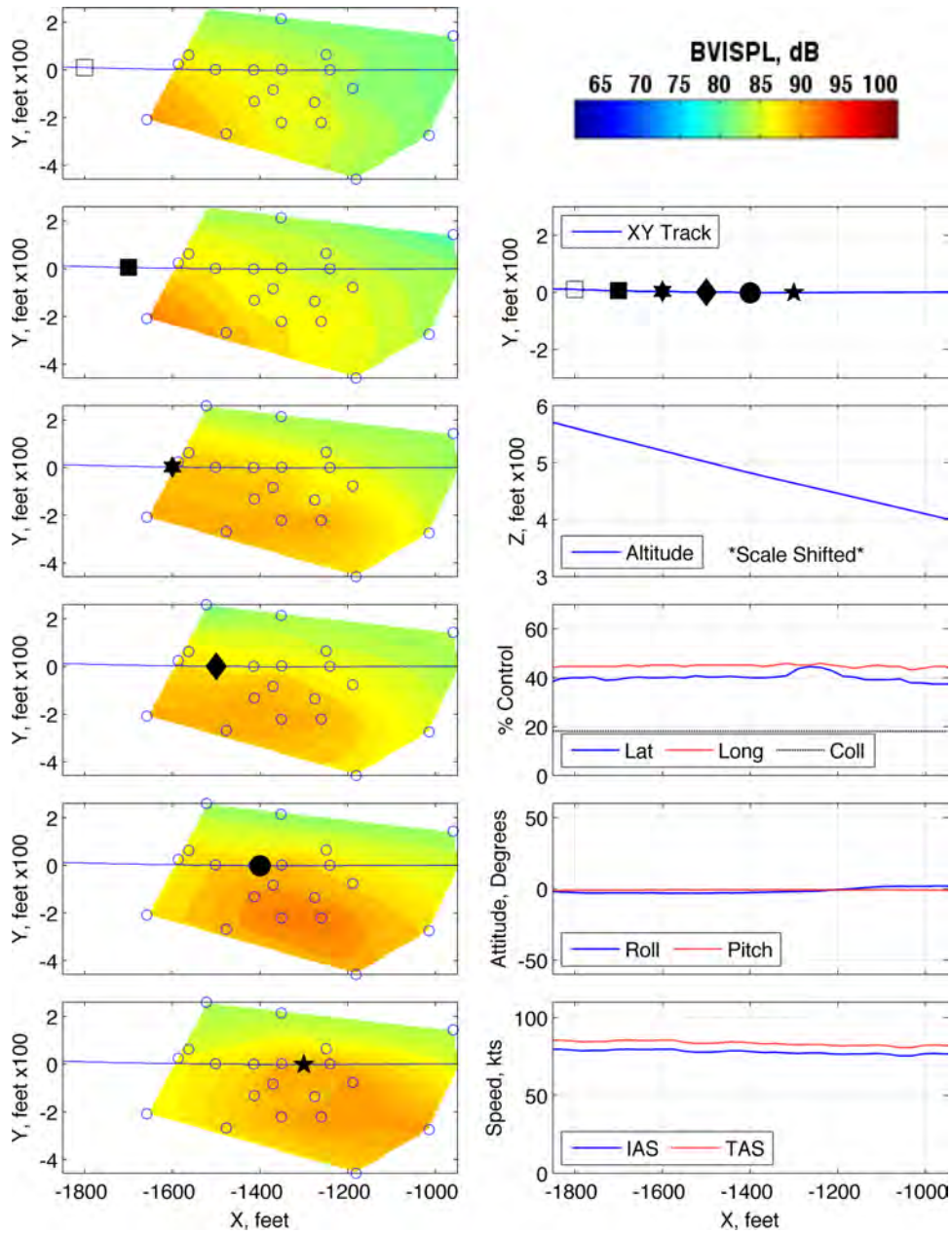
Figure 117: Maneuver condition A24, 80 KIAS, -12^\circ , run number 285496
