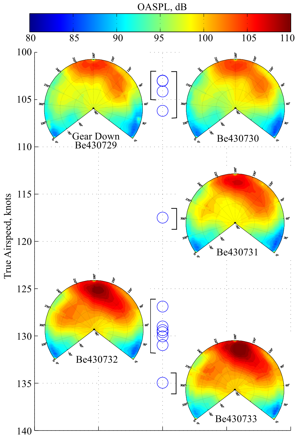
Figure 27: Semi-spheres for high speed level flight, OASPL.
