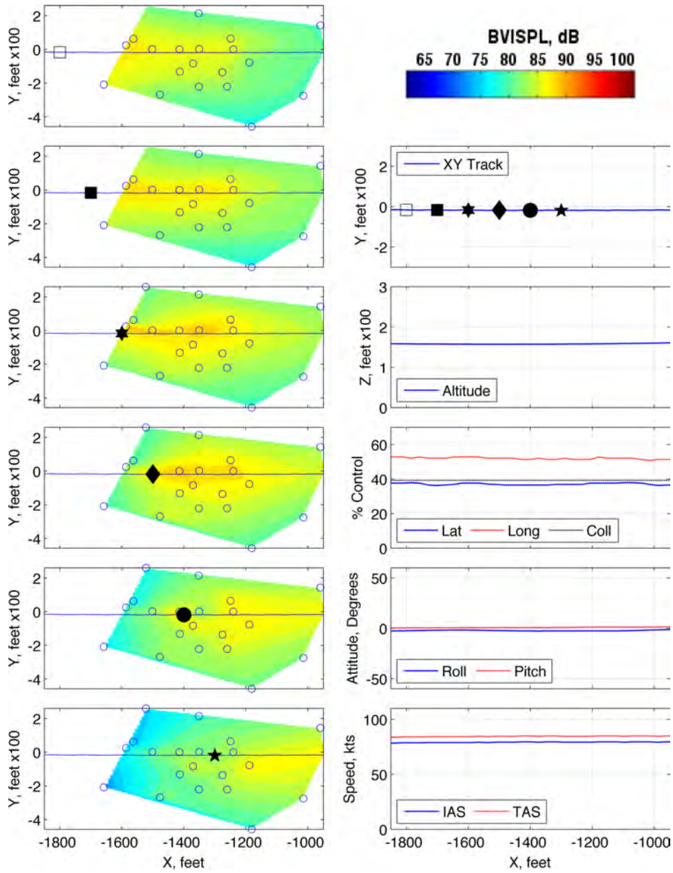
Figure 96: Maneuver condition L1, 80 KIAS, level, run number 285461
