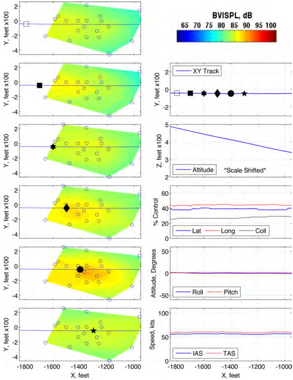
Figure 103: Maneuver condition A8, 60 KIAS, -9° , run number 282444
