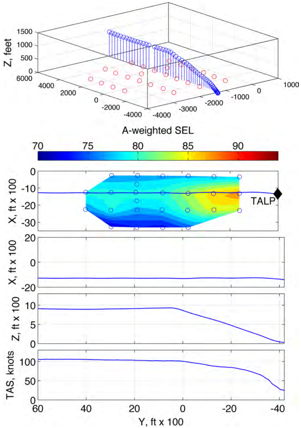
Figure 344: Terminal area condition T5, 100 KIAS decelerating, -12^\circ , run number 288614
