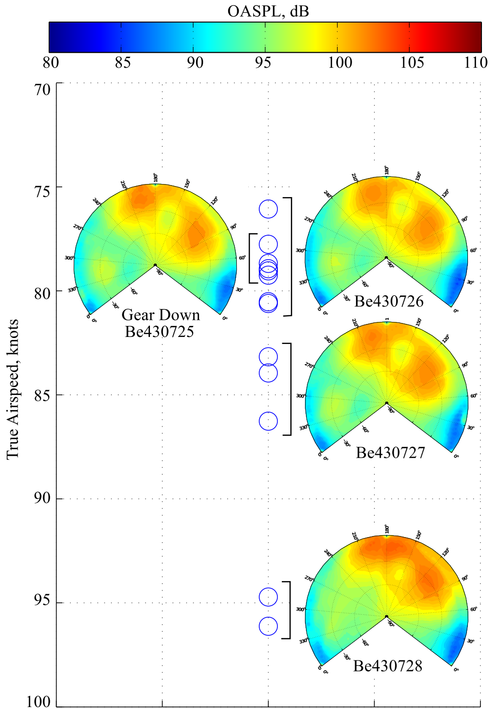
Figure 26: Semi-spheres for mid speed level flight, OASPL.
