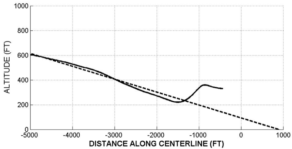
Figure 9: Quick-look aircraft position.
