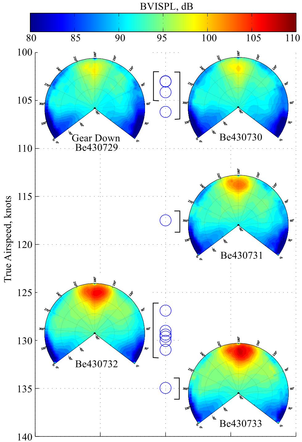
Figure 30: Semi-spheres for high speed level flight, BVISPL.
