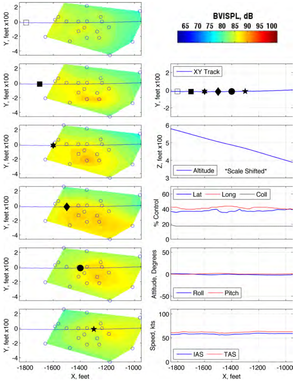
Figure 107: Maneuver condition A10, 60 KIAS, -12^\circ , run number 285495
