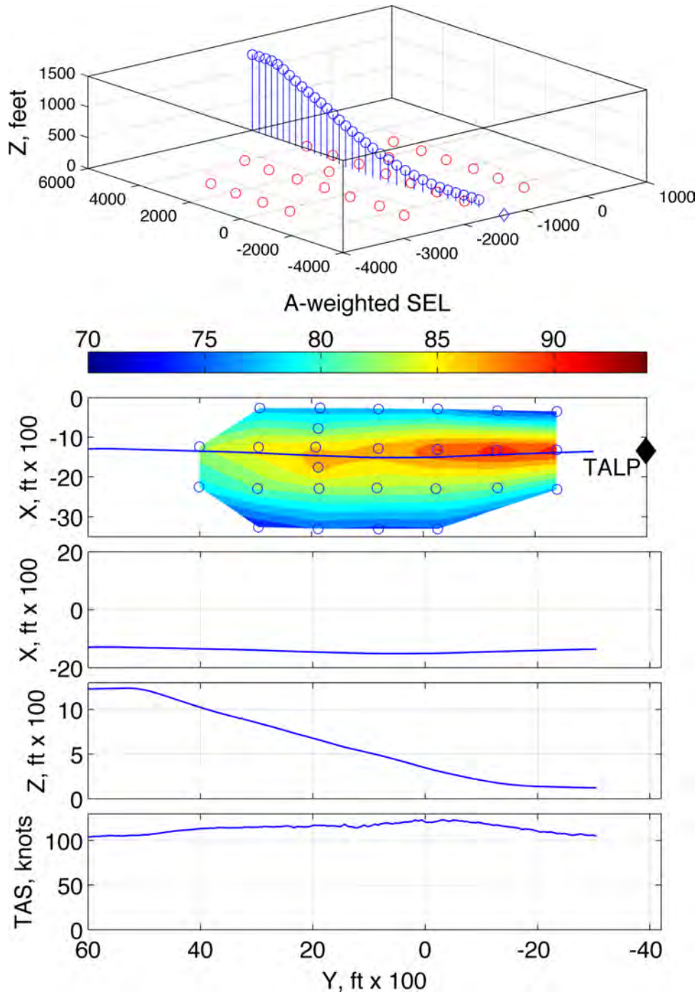
Figure 356: Terminal area condition T9A, segmented 100 - 110 KIAS, -9^\circ , 110 - 90 KIAS, -7.5^\circ , 90 - 0 KIAS, -4^\circ , run number 288632
