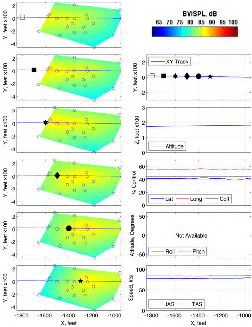
Figure 90: Maneuver condition L1, 80 KIAS, level, run number 278301
