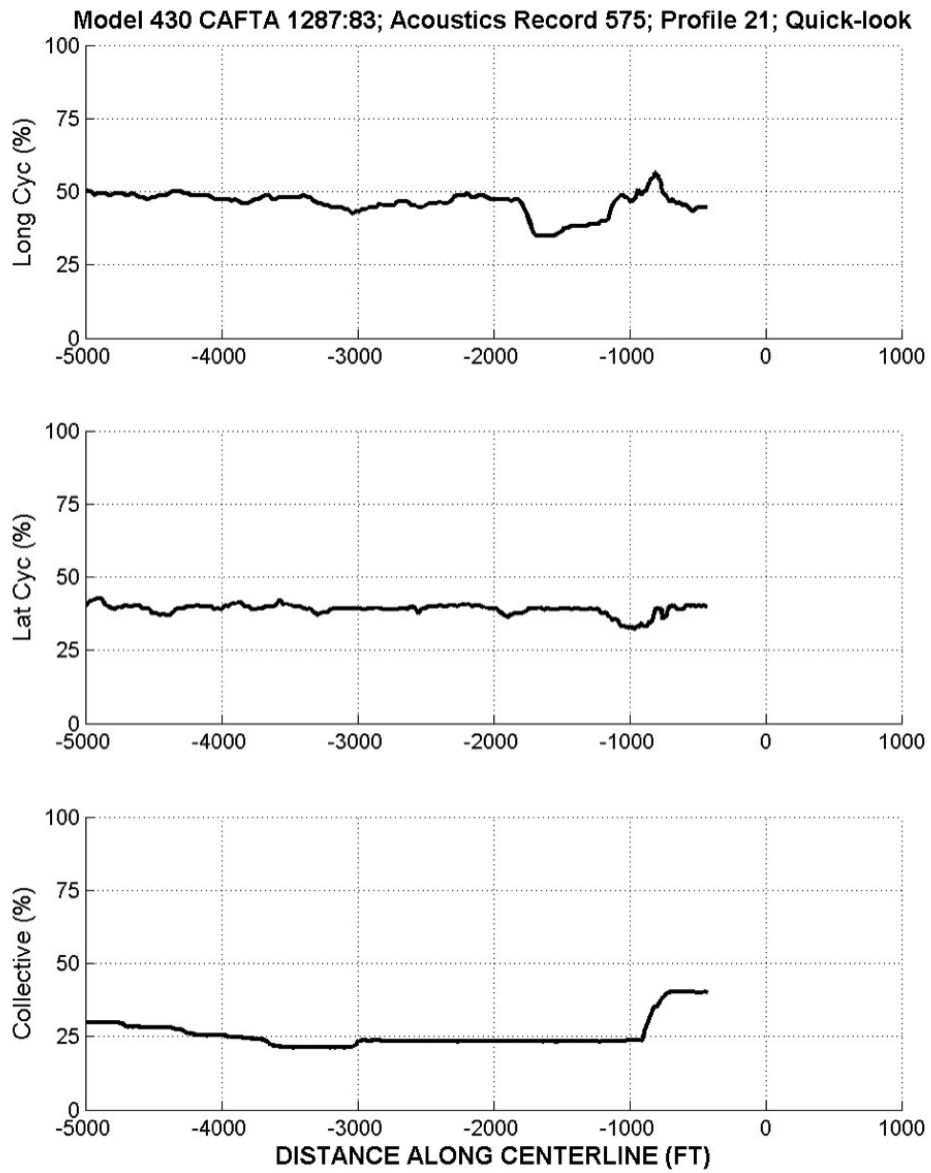
Figure 10: Quick-look aircraft control positions.
