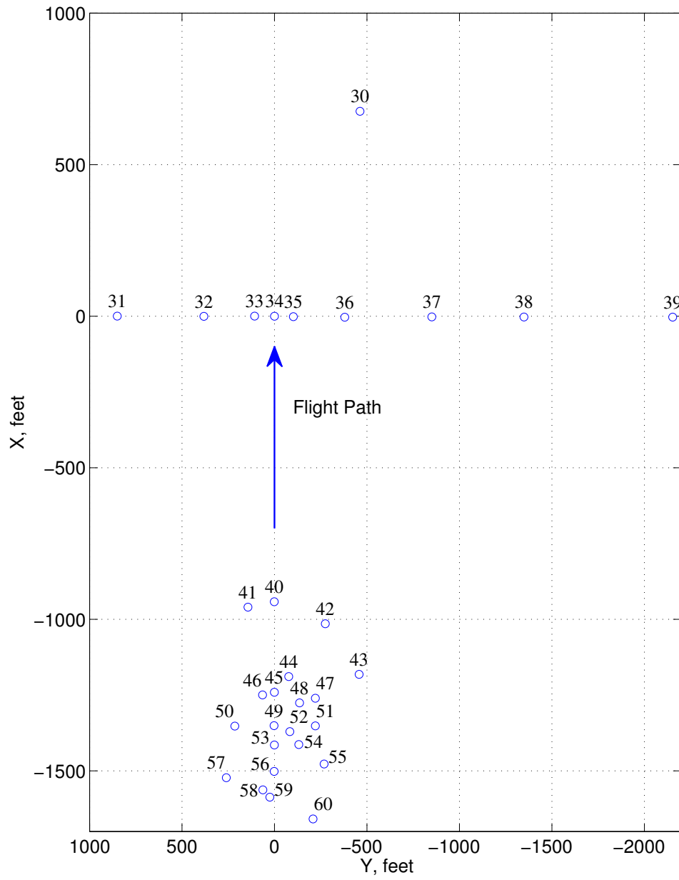
Figure 18: Maneuver microphone array.
