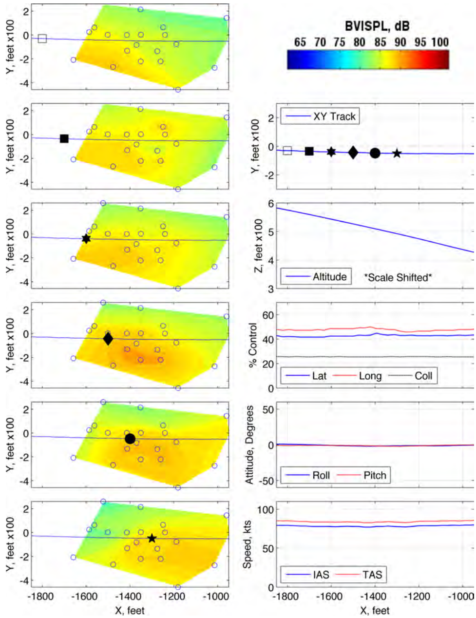
Figure 116: Maneuver condition A24, 80 KIAS, -12^\circ , run number 282443
