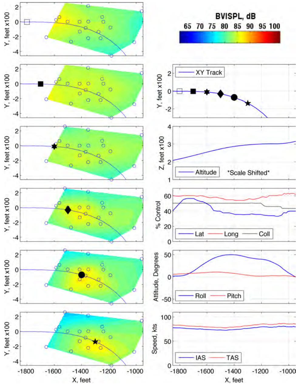
Figure 312: Maneuver condition Z18, 80 KIAS, 0^\circ to 9^\circ , roll right, run number 287554
