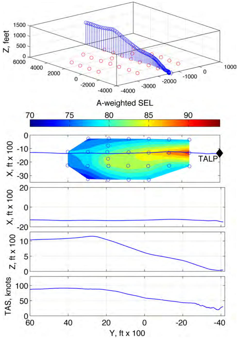
Figure 349: Terminal area condition T7, segmented 100 - 90 KIAS, 3^\circ , 90 - 0 KIAS, -9.5^\circ , run number 288619
