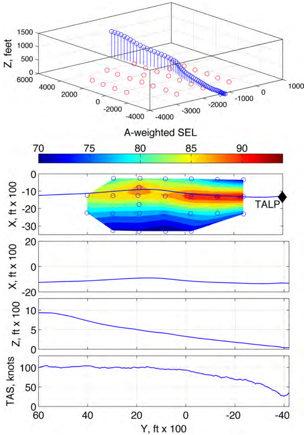
Figure 354: Terminal area condition T9, segmented 100 - 110 KIAS, -9^\circ , 110 - 90 KIAS, -7.5^\circ , 90 - 0 KIAS, -4^\circ , run number 288630
