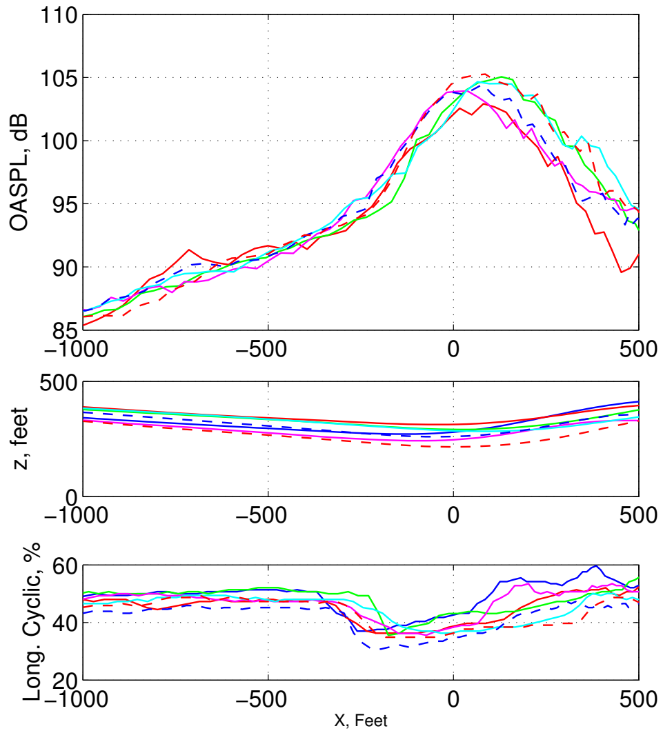
Figure 89: Cyclic pitch up from 80 knot, 6° descent housekeeping points.
