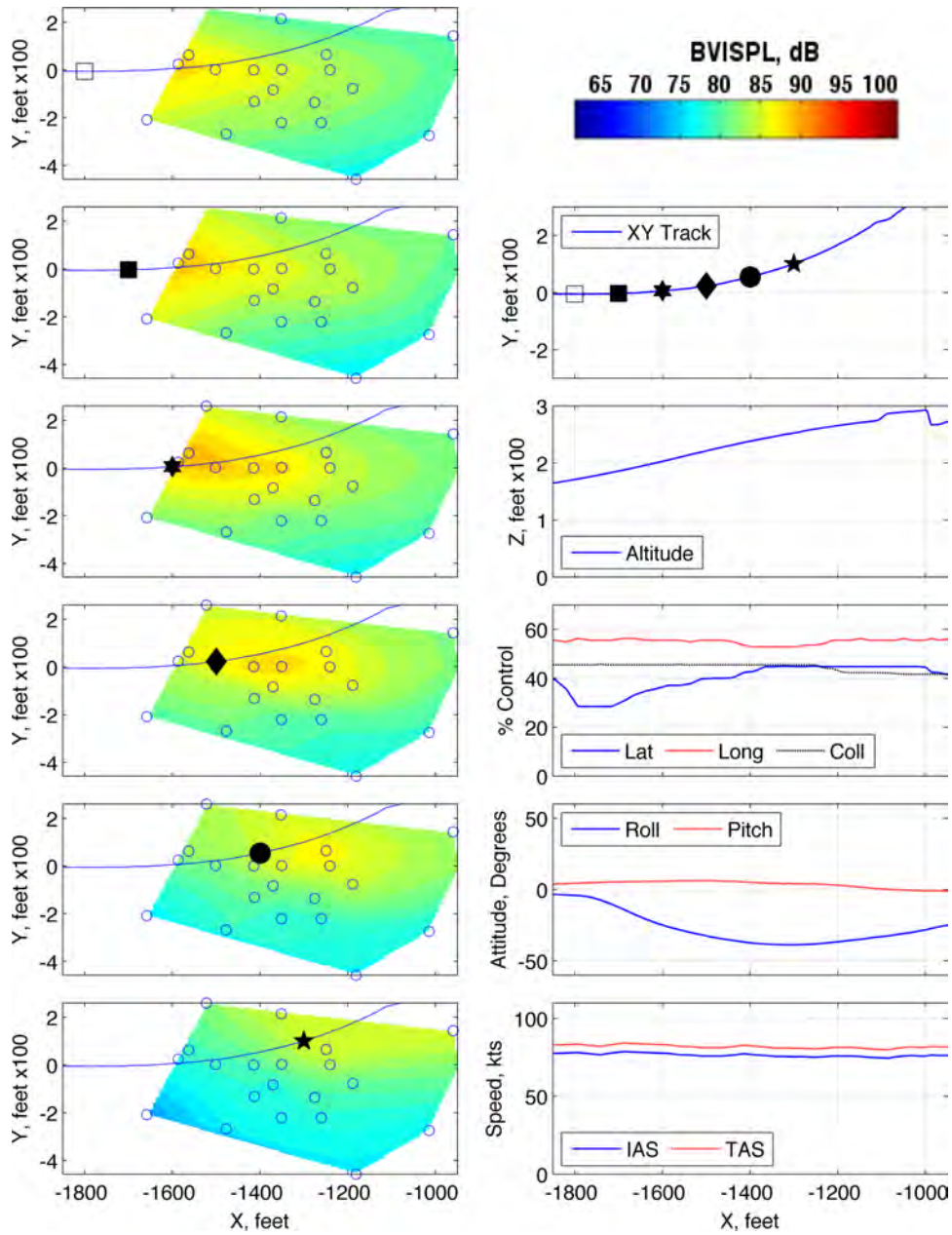
Figure 302: Maneuver condition Z6, 80 KIAS, 0° to 6° , roll left, run number 287551
