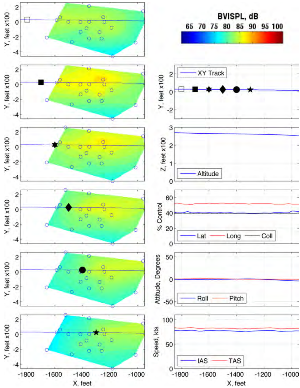
Figure 112: Maneuver condition A18, 80 KIAS, -3^\circ , run number 282449
