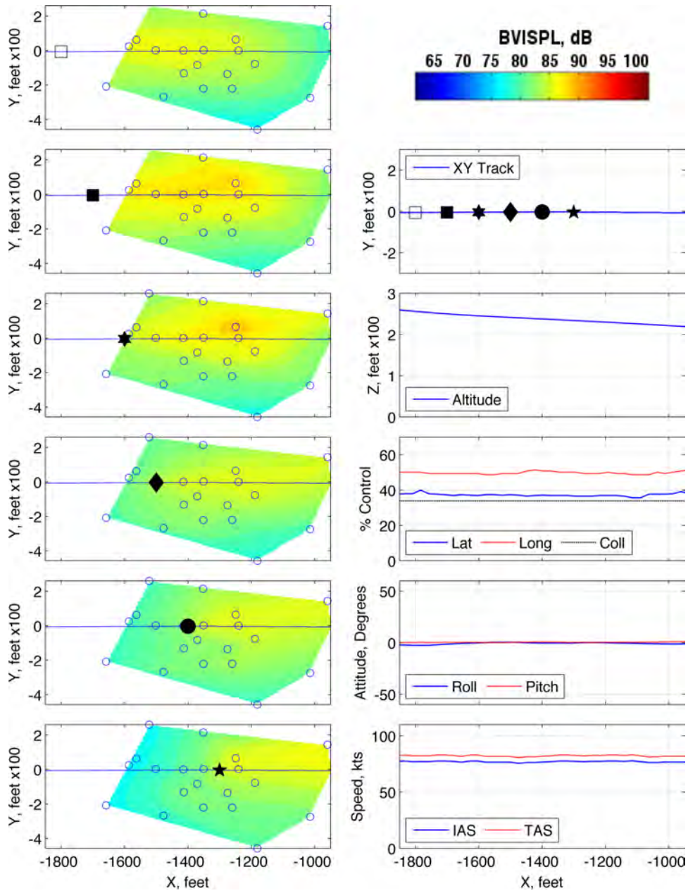
Figure 113: Maneuver condition A18, 80 KIAS, -3^\circ , run number 285498
