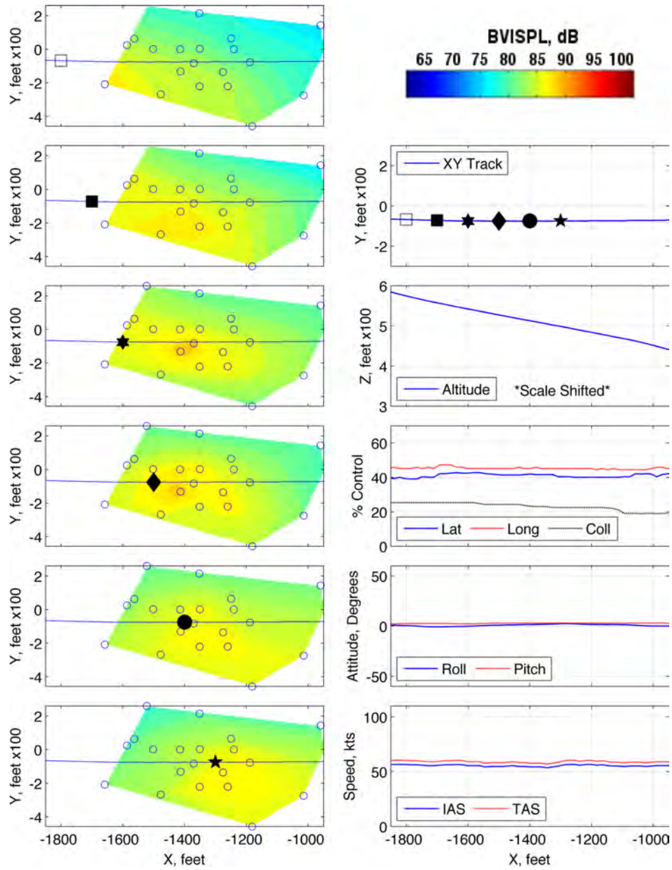
Figure 105: Maneuver condition A10, 60 KIAS, -12^\circ , run number 282442
