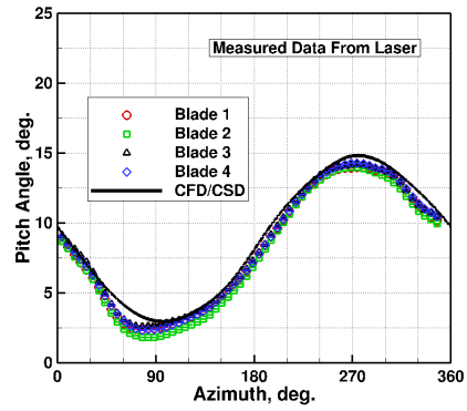
(b) Pitch: Laser Data
