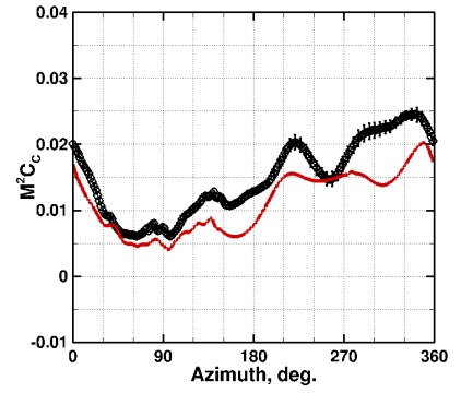
(f) M^2 C_c, r/R = 0.865
