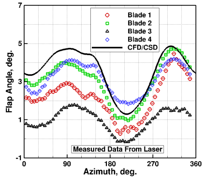
(e) Flap: Laser Data
