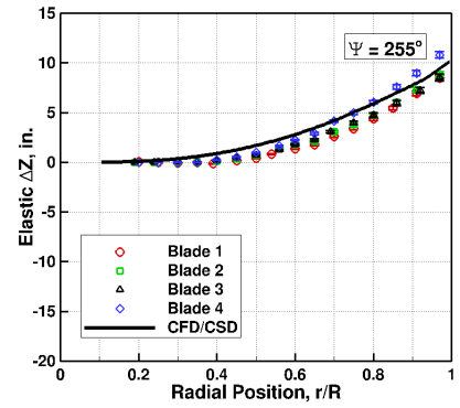
(c) Psi = 255 deg.
