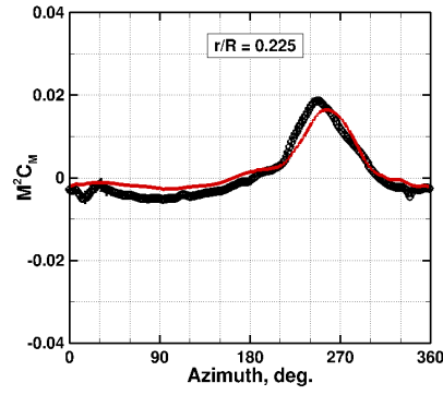
(b) M^2 C_m, r/R = 0.225
