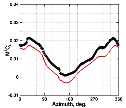
(l) M^2 C_c, r/R = 0.990
