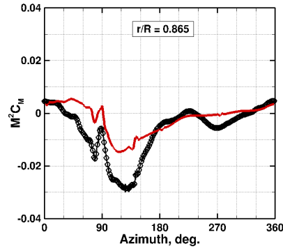
(e) M^2 C_m, r/R = 0.865
