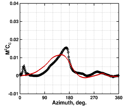
(c) M^2 C_c, r/R = 0.225
