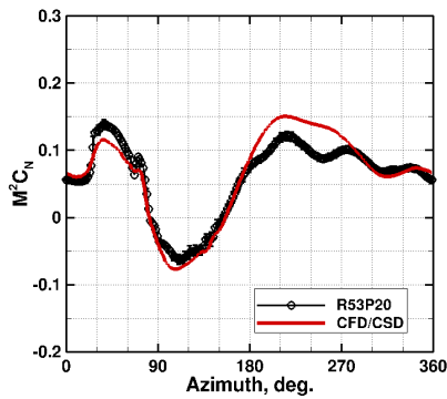
(j) M^2 C_n, r/R = 0.990
