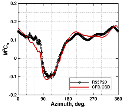
(g) M^2 C_n, r/R = 0.920
