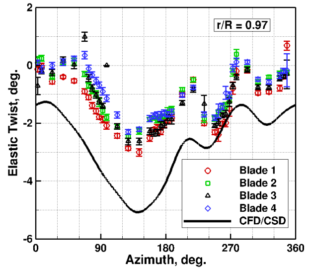
(b) Elastic Twist
