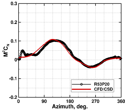
(a) M^2 C_n, r/R = 0.225
