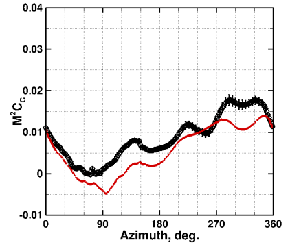
(i) M^2 C_c, r/R = 0.920
