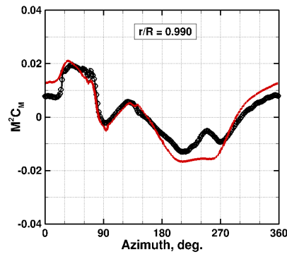
(k) M^2 C_m, r/R = 0.990
