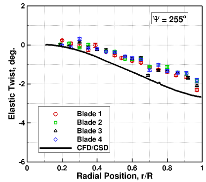
(f) Psi = 255 deg.
