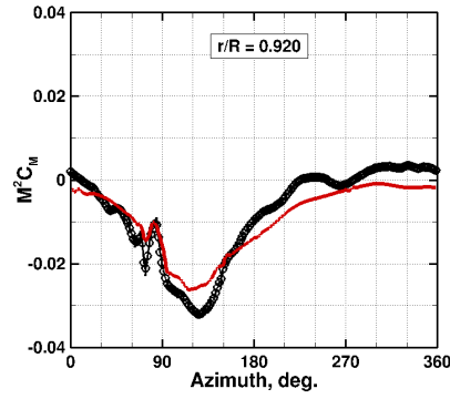
(h) M^2 C_m, r/R = 0.920
