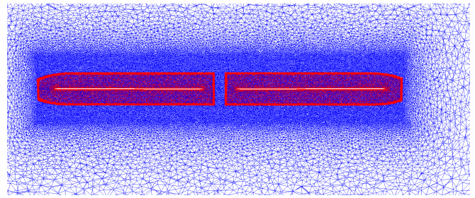
Fig. 4. Slice through the CFD grid used to model the rotor.
