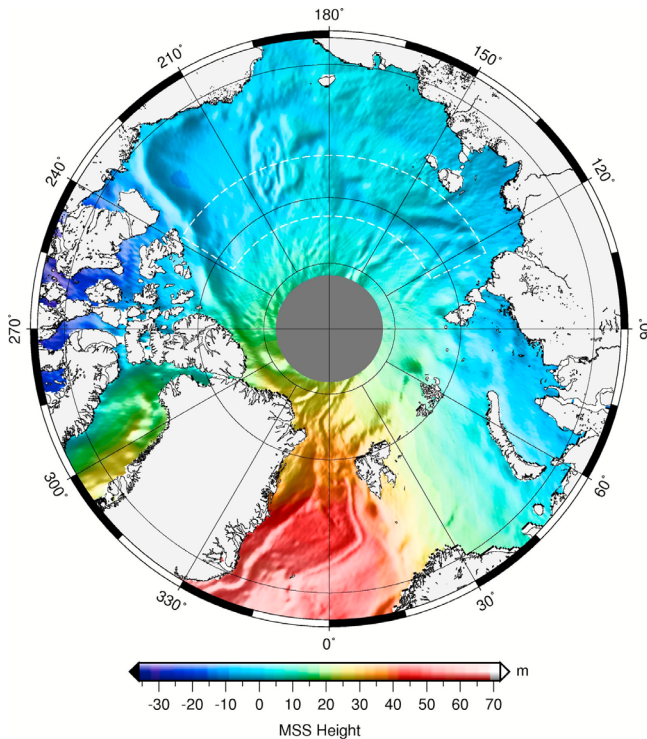
Figure 1. The ICEn Mean Sea Surface (MSS) model of the Arctic Ocean. Artificial illumination from 125 °E has been added to emphasize topographical features of the MSS. The ICEn MSS is computed with respect to the Topex/Poseidon Reference Ellipsoid. A dashed-white box outlines Region A.
