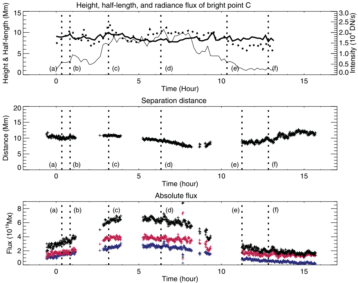
Figure 5. Temporal evolution of the physical parameters of case C. Other explanations are the same as Figure 1. (A color version of this figure is available in the online journal.)
