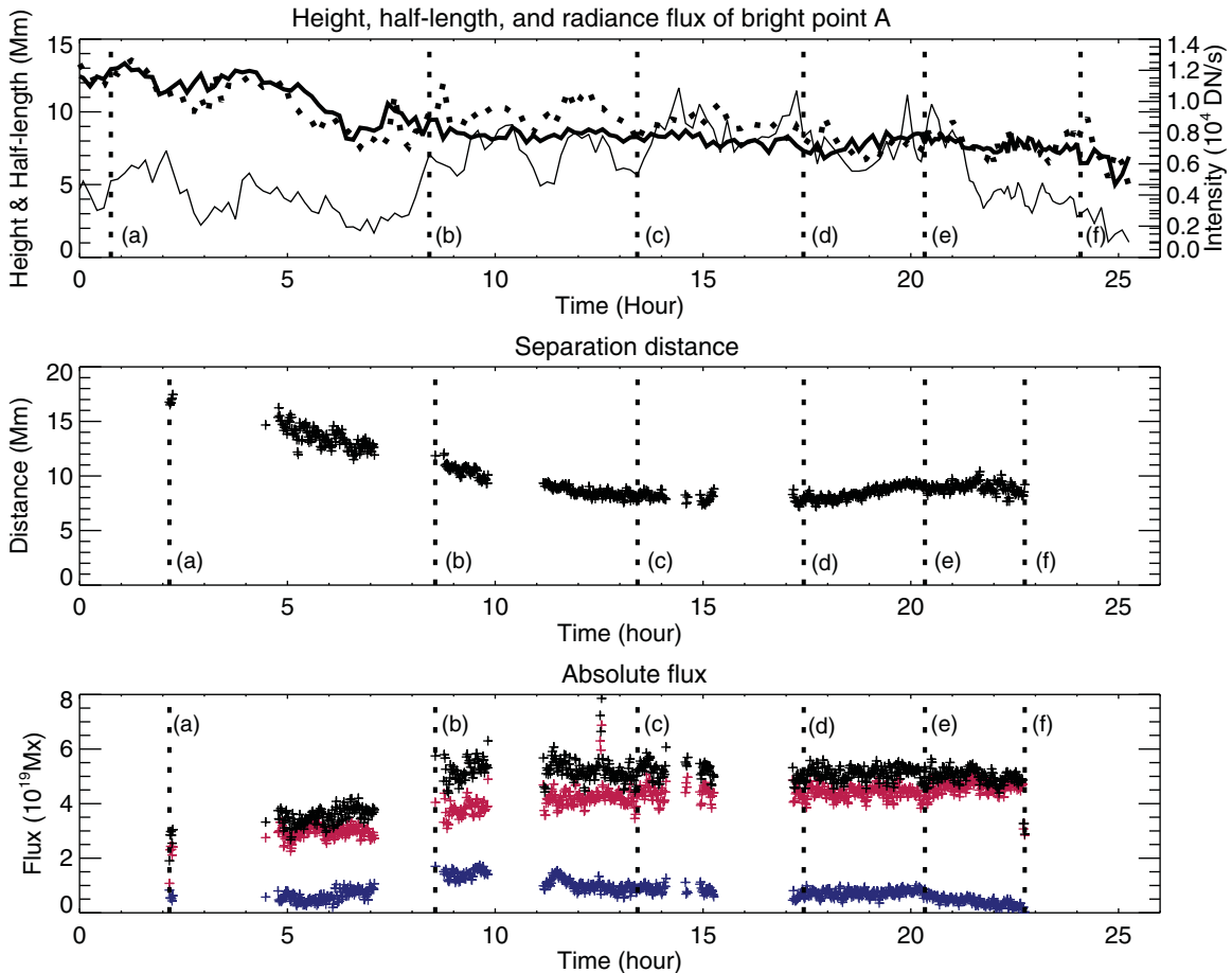
Figure 1. Temporal evolution of the physical parameters of the case A BP. The x -axis refers to the relative time from when the BP first appeared. The top panel shows the height (solid), half-length (dotted), and integrated intensity (thin solid) variations. The middle panel represents the distance between two opposite magnetic flux concentrations in units of Mm and the bottom panel shows the unsigned magnetic flux variation in units of 1 \times 10^{19} Mx. The black, blue, and red colors refer to the unsigned total, negative, and positive magnetic fluxes, respectively. The letters from (a) to (f) refer to the specific times which show some noticeable morphological changes (see the text) in Figure 2.
