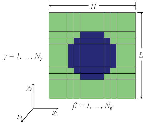
Figure 7: RUC used in square-packed analyses containing 7 \times 7 subcell architecture. Blue subcells are composed of the AS4 fiber material, and green subcells are composed of 3502 matrix material.
