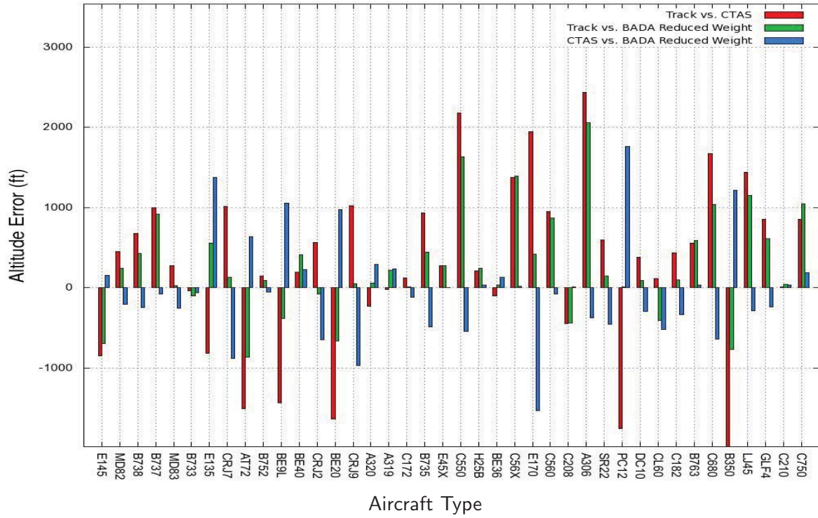
Figure 26. Mean of mean altitude errors in climb, BADA Reduced Weight
