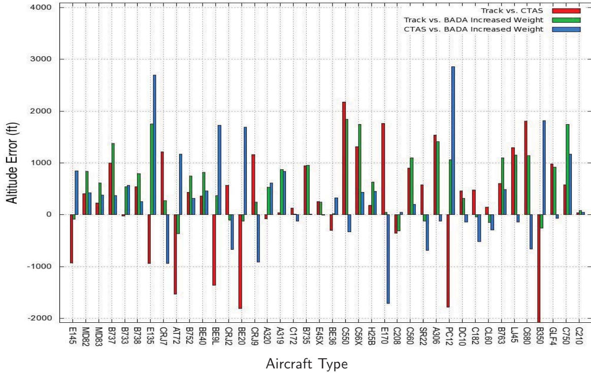
Figure 28. Mean of mean altitude errors in climb, BADA Increased Weight
