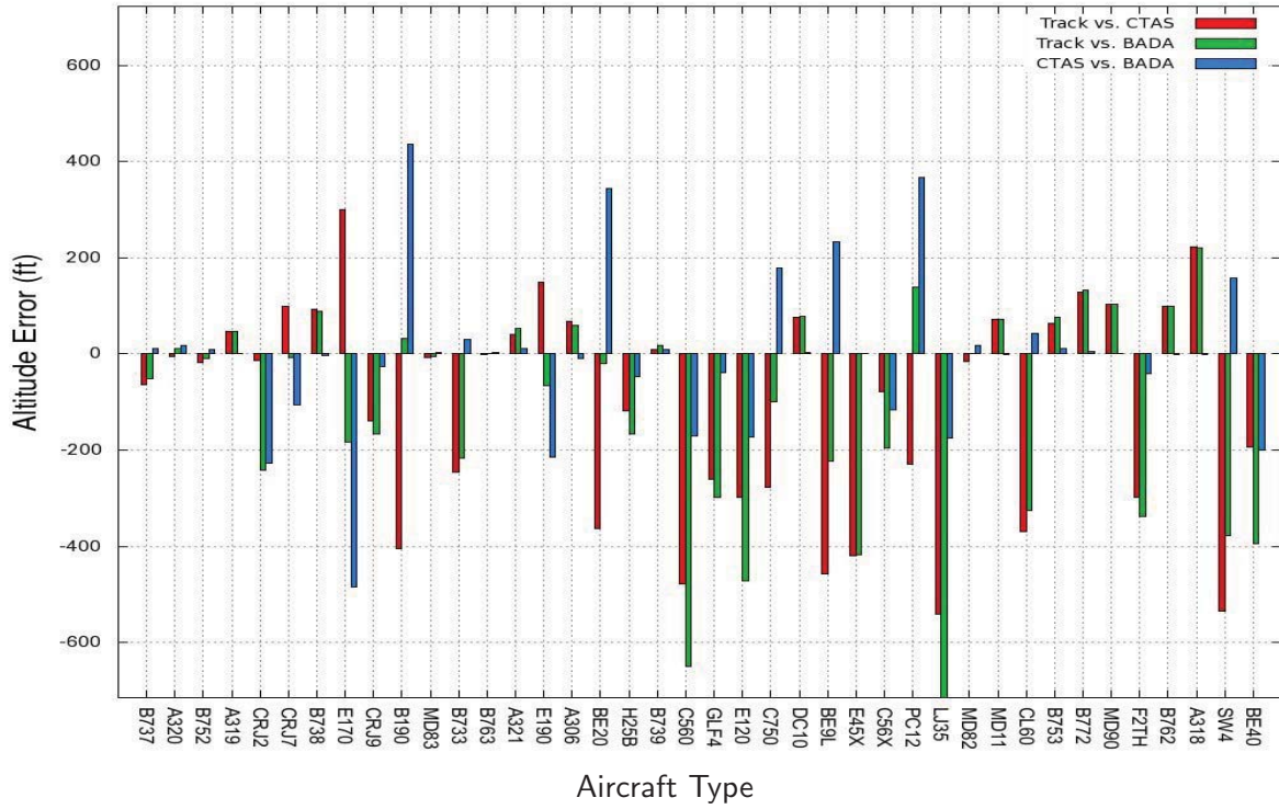
Figure 40. Mean of mean altitude errors in Denver center
