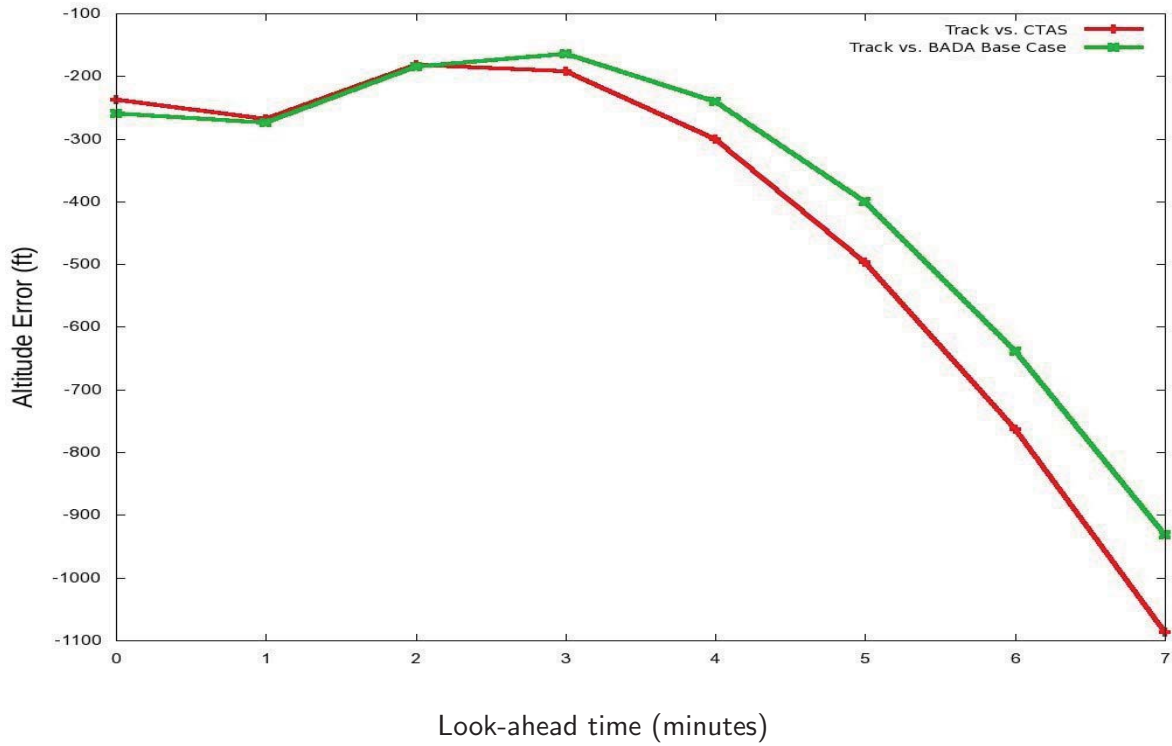
Figure 18. Interval-based sampling, mean altitude error during descent
