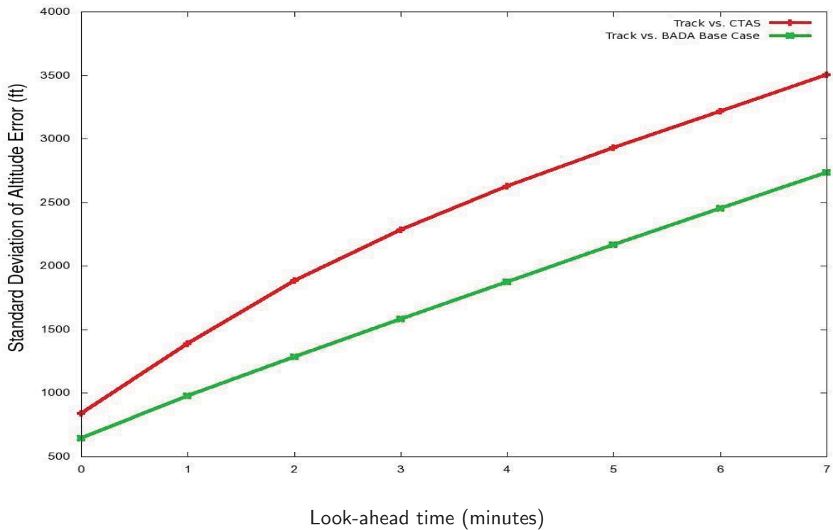
Figure 17. Interval-based sampling, standard deviation of altitude error during climb
