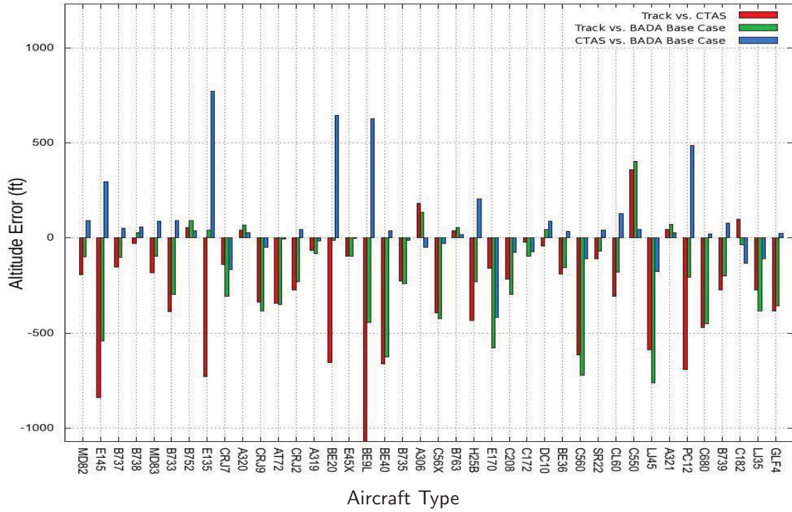
Figure 6. Mean of mean altitude errors
