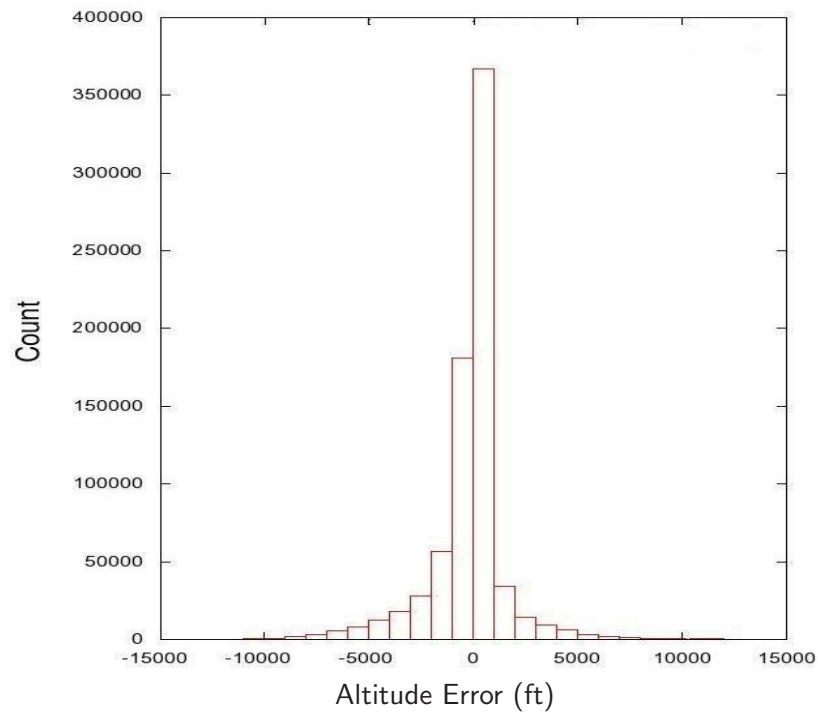
Figure 4. Overall mean altitude error, CTAS distribution
