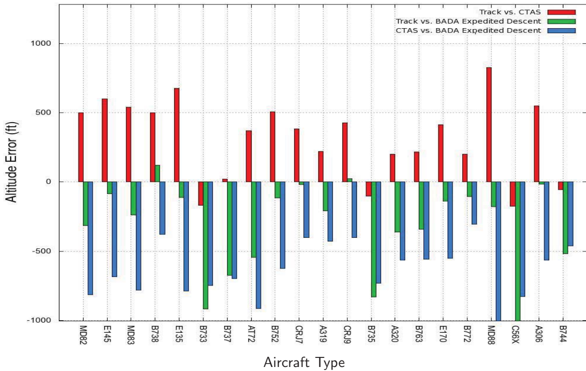
Figure 25. Mean of mean altitude errors for BADA Expedited Descent, TRACON only
