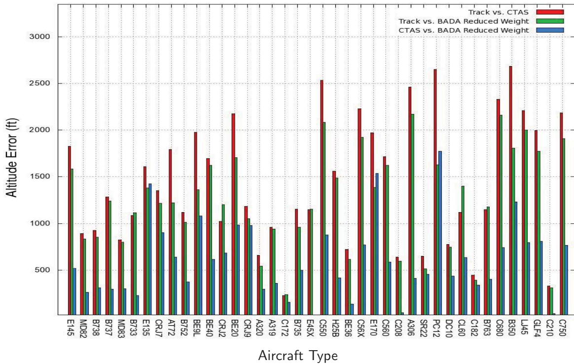
Figure 29. Mean of absolute mean altitude errors in climb, BADA Reduced Weight
