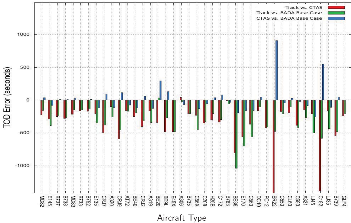
Figure 11. Events, Mean of mean TOD time errors
