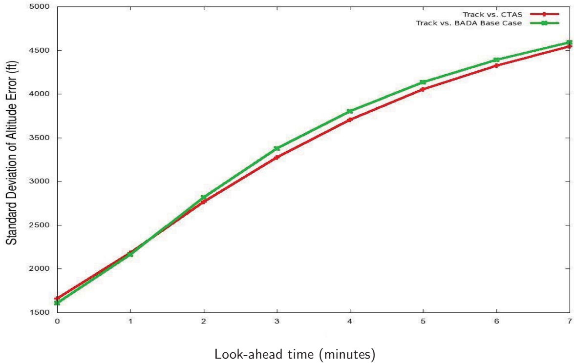
Figure 20. Interval-based sampling, standard deviation of altitude error during descent
