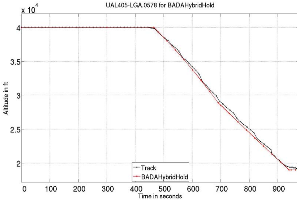
Figure 46. Boeing 757-200 BADA Hybrid Hold idle descent: altitude
