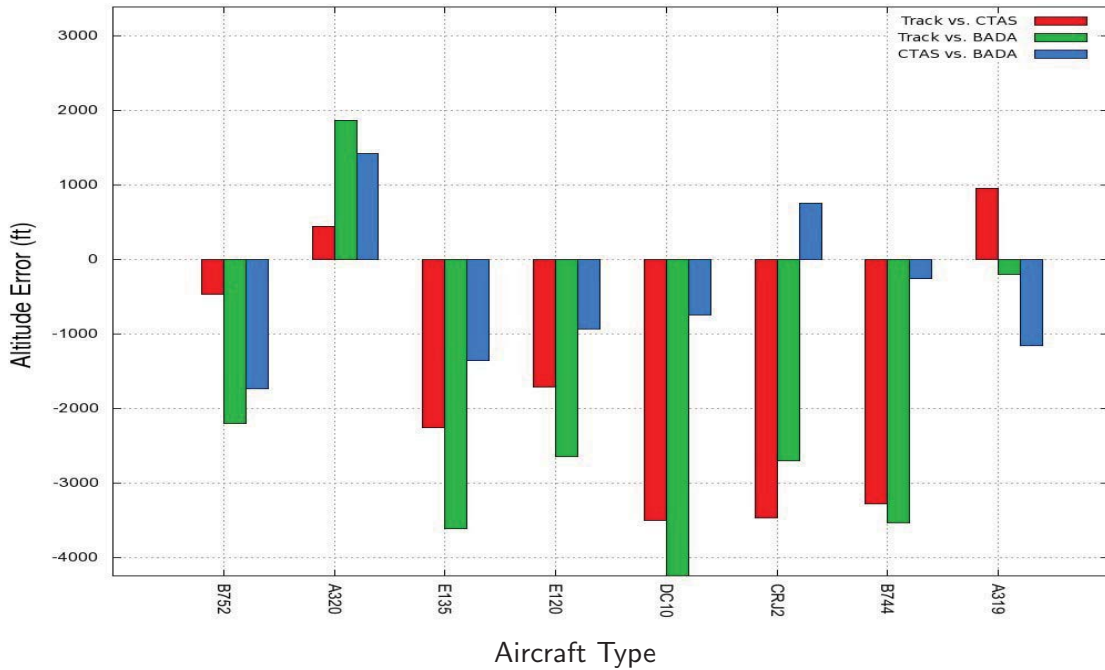
Figure 37. Mean of mean altitude errors in Los Angeles center, TRACON only
