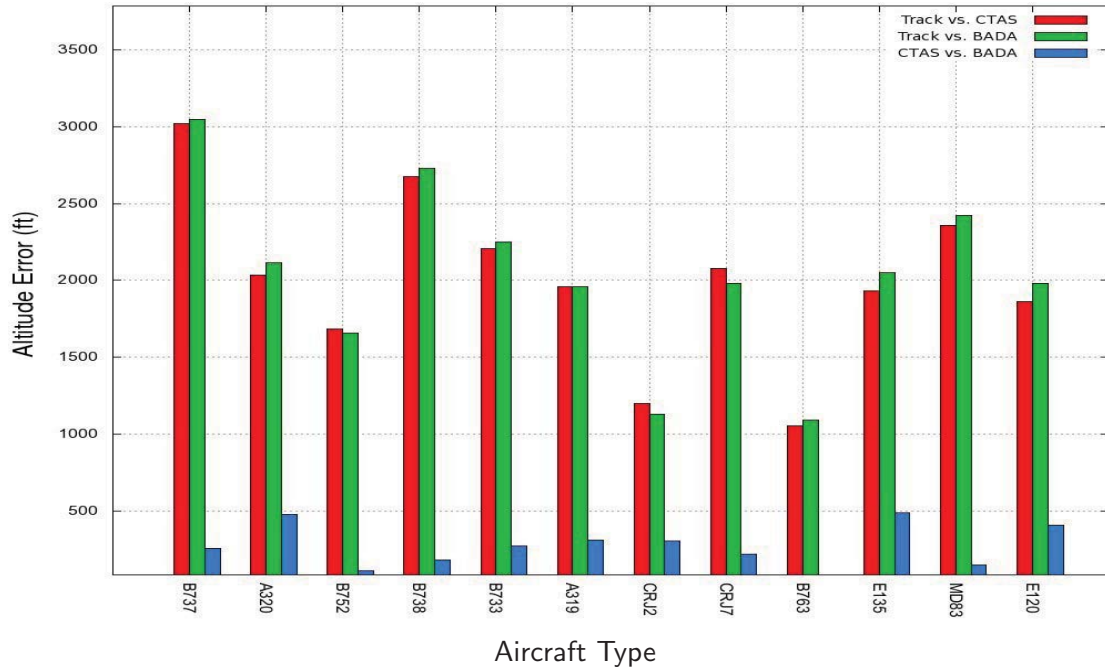
Figure 36. Mean of absolute mean altitude errors in Los Angeles center
