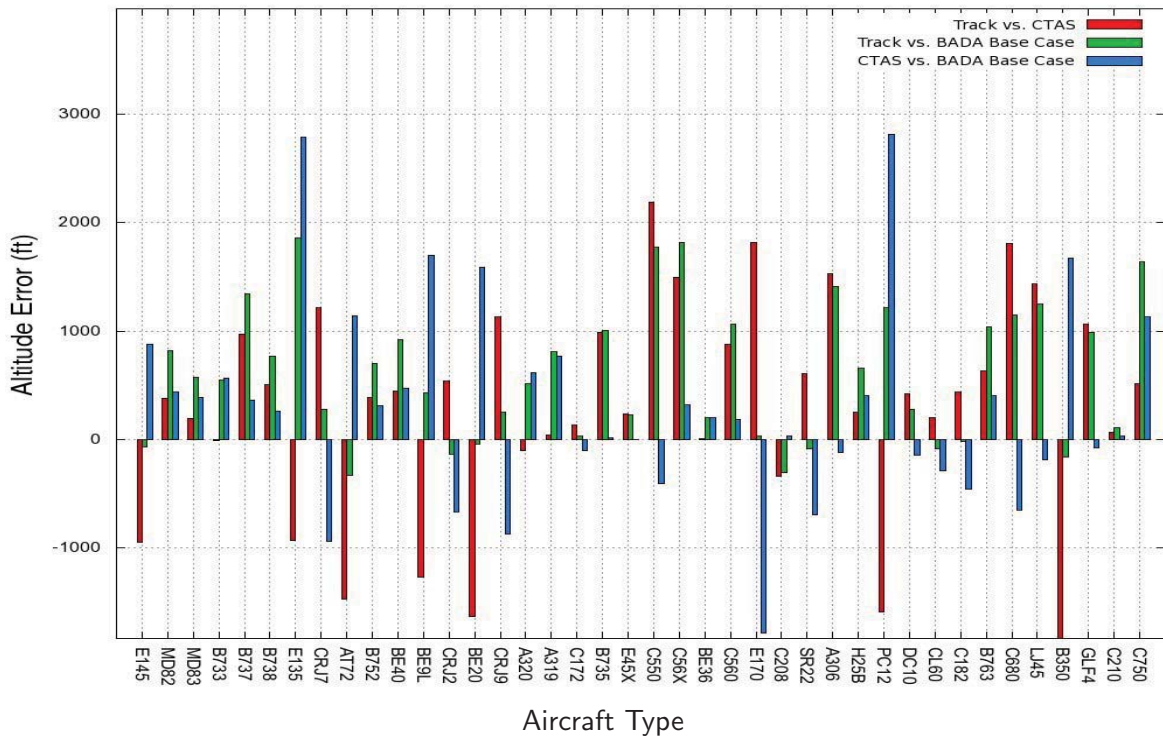
Figure 27. Mean of mean altitude errors in climb, BADA Nominal Weight
