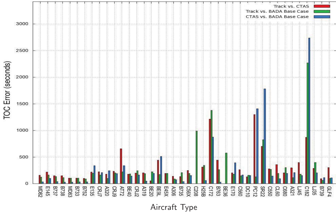
Figure 10. Events, Mean of absolute mean TOC time errors
