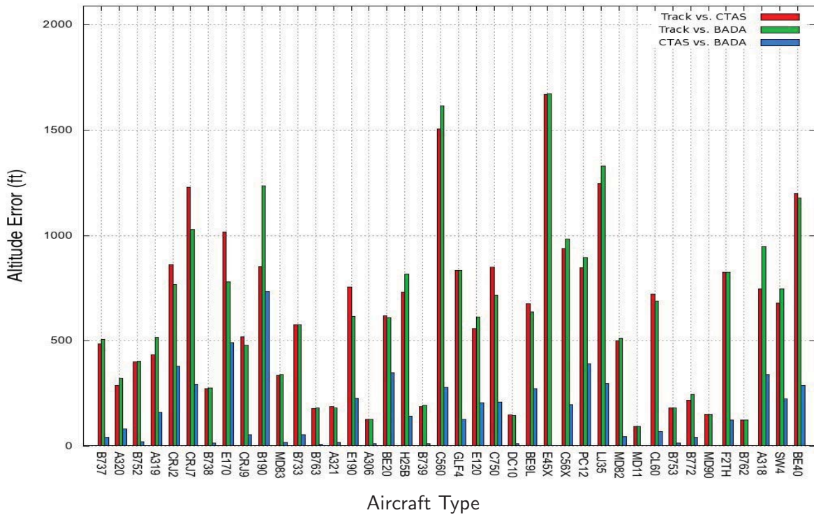
Figure 41. Mean of absolute mean altitude errors in Denver center
