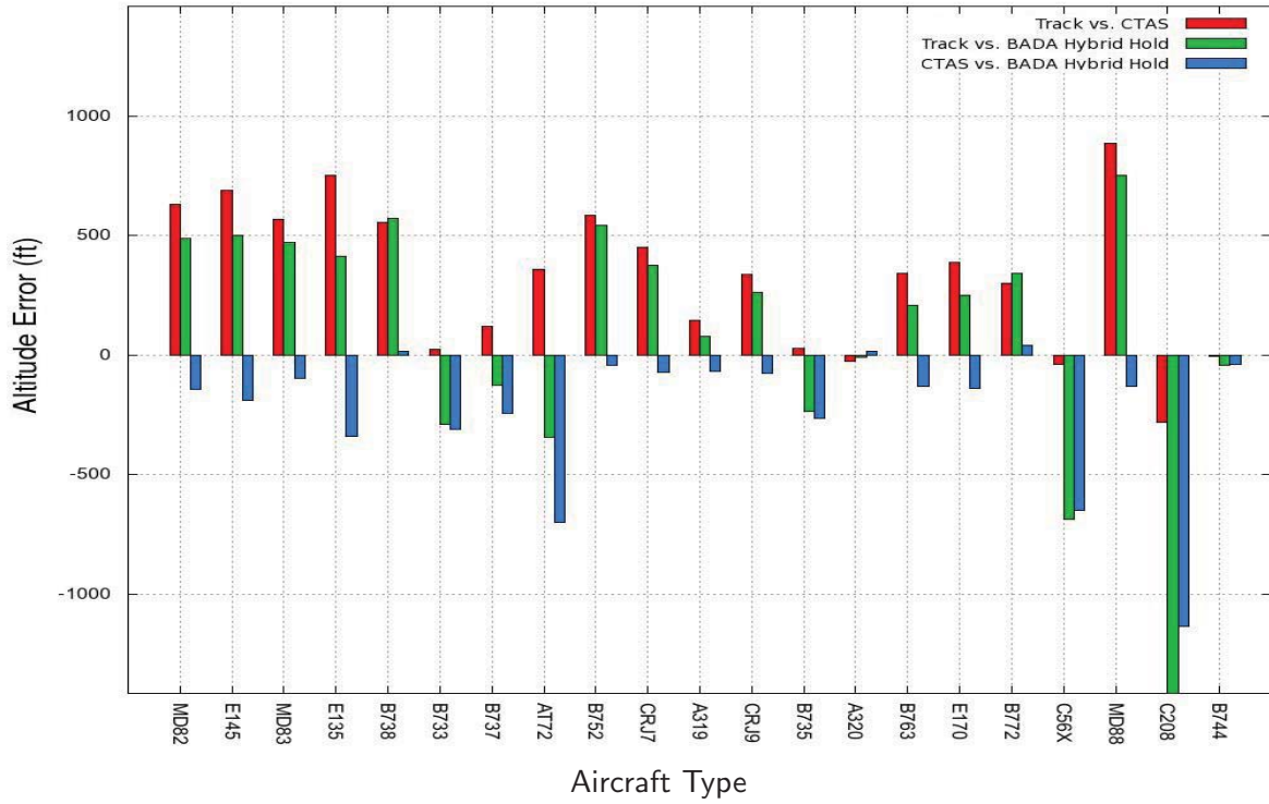
Figure 24. Mean of mean altitude errors for BADA Hybrid Hold, TRACON only
