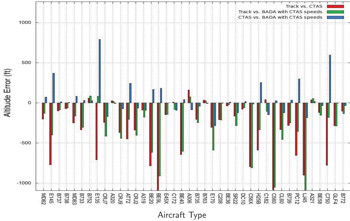
Figure 32. Mean of mean altitude errors for BADA with CTAS speeds
