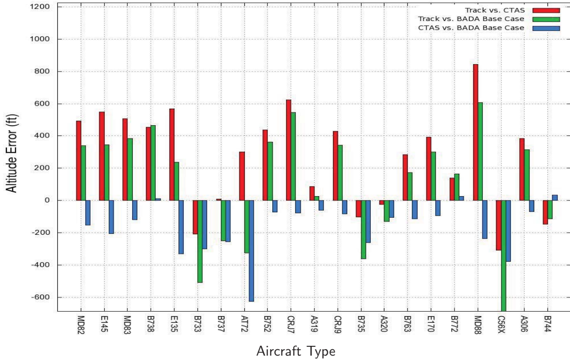
Figure 22. Mean of mean altitude errors, TRACON only
