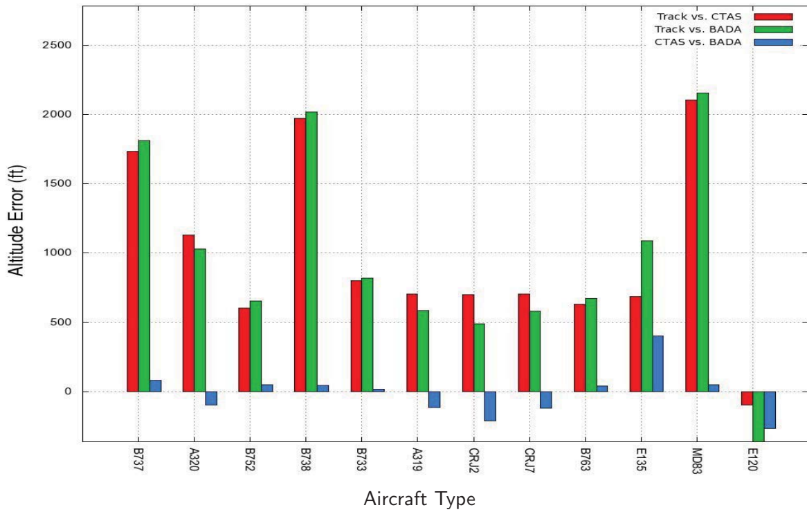
Figure 35. Mean of mean altitude errors in Los Angeles center
