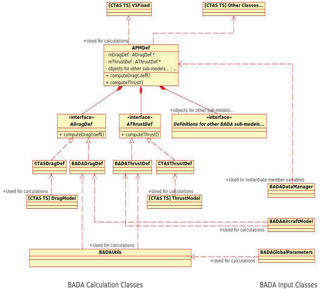
Figure 1. CTAS/BADA TS Class Diagram
