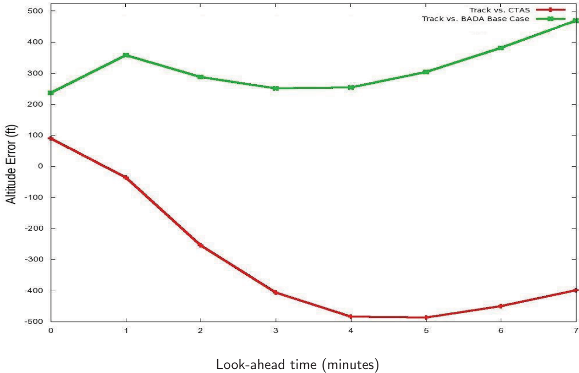
Figure 15. Interval-based sampling, mean altitude error during climb
