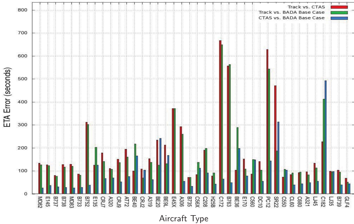
Figure 14. Events, Mean of absolute mean ETA time errors
