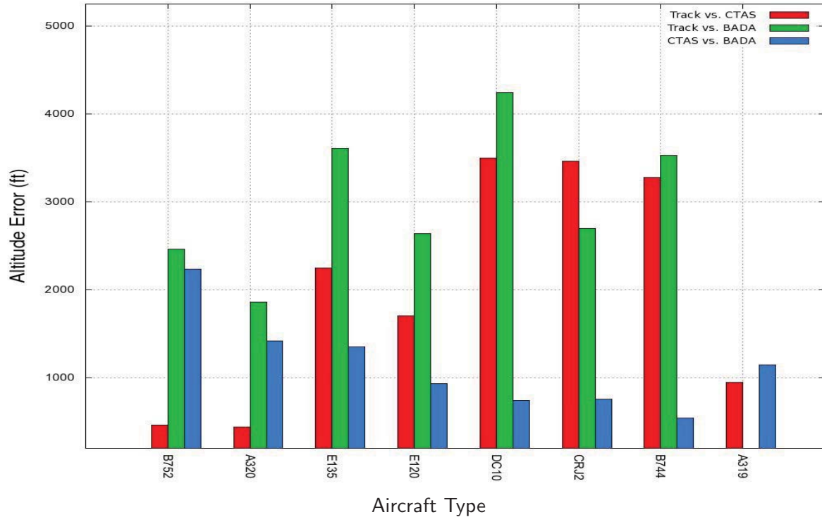
Figure 38. Mean of absolute mean altitude errors in Los Angeles center, TRACON only
