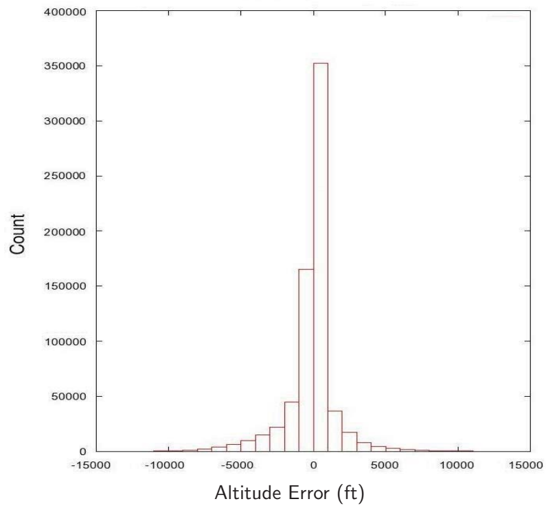
Figure 5. Overall mean altitude error, BADA distribution
