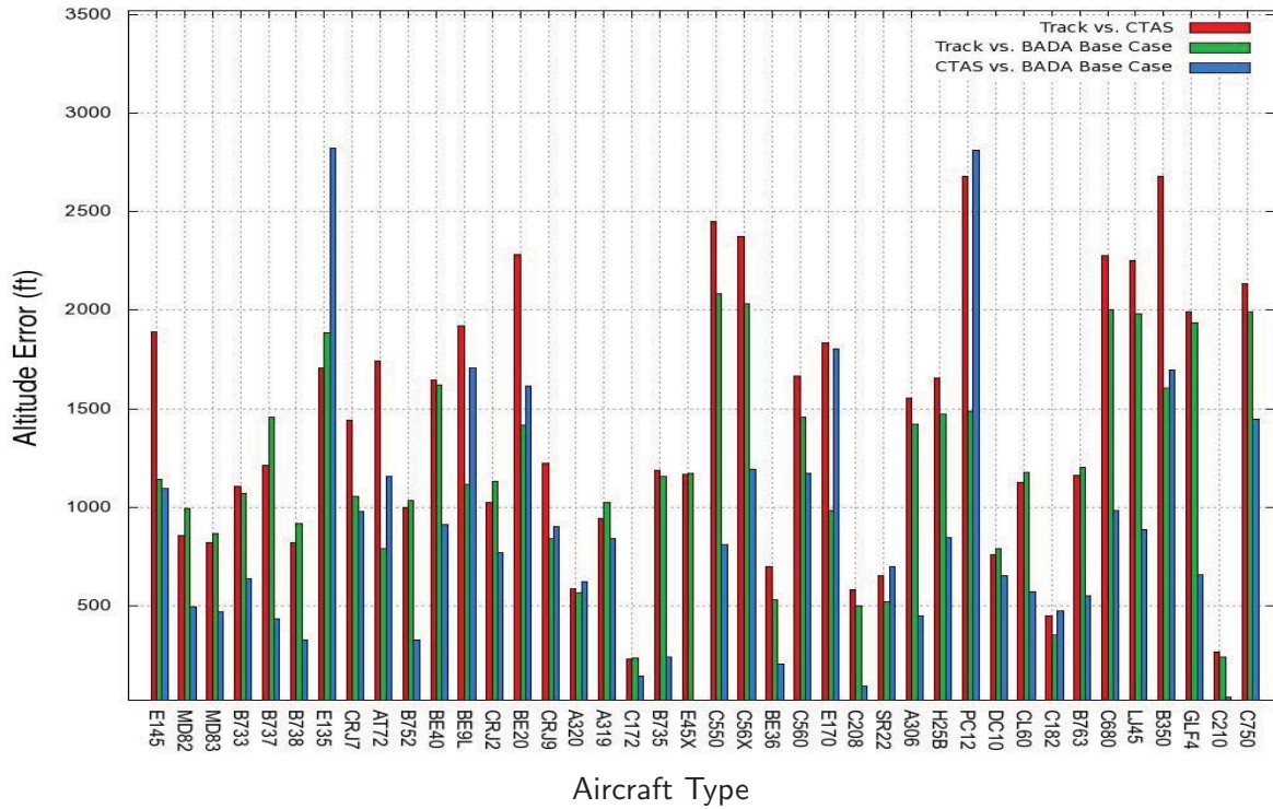
Figure 30. Mean of absolute mean altitude errors in climb, BADA Nominal Weight
