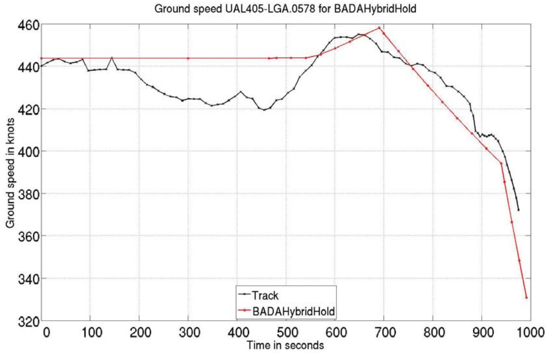
Figure 45. Boeing 757-200 BADA Hybrid Hold idle descent: ground speed
