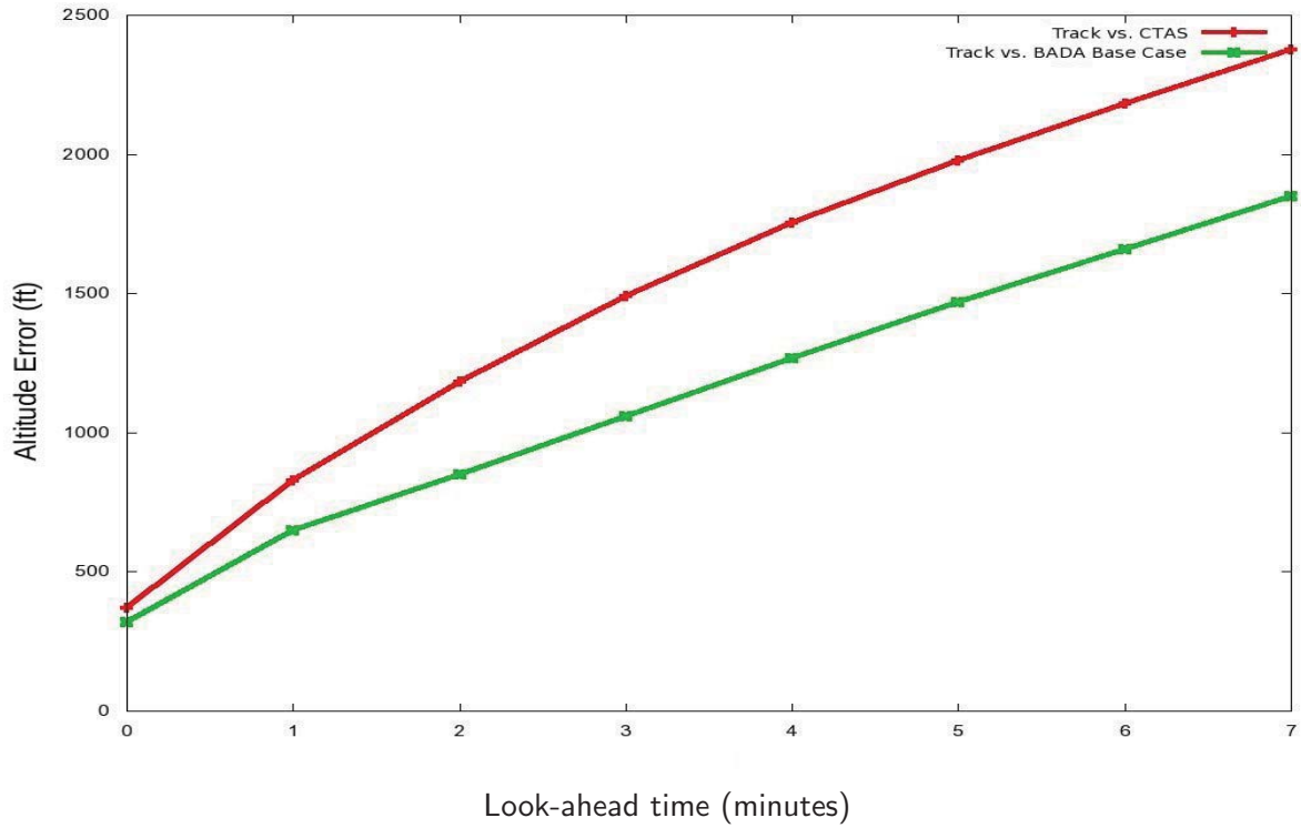
Figure 16. Interval-based sampling, mean absolute altitude error during climb
