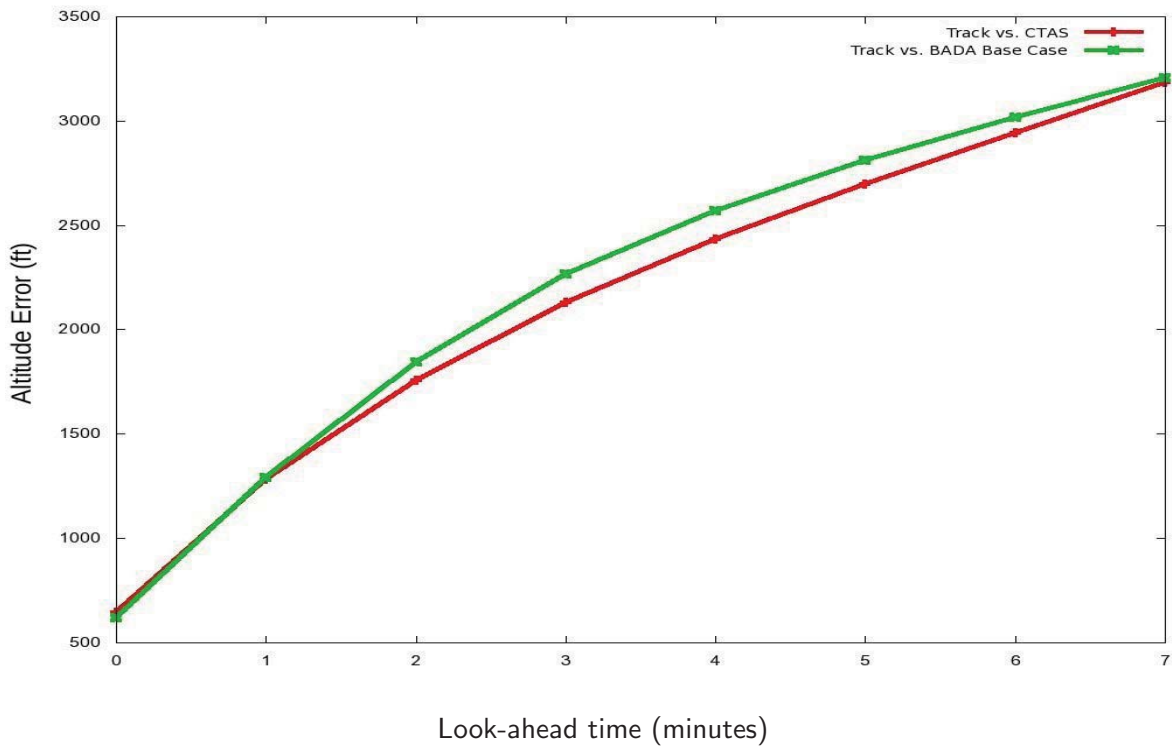
Figure 19. Interval-based sampling, mean absolute altitude error during descent
