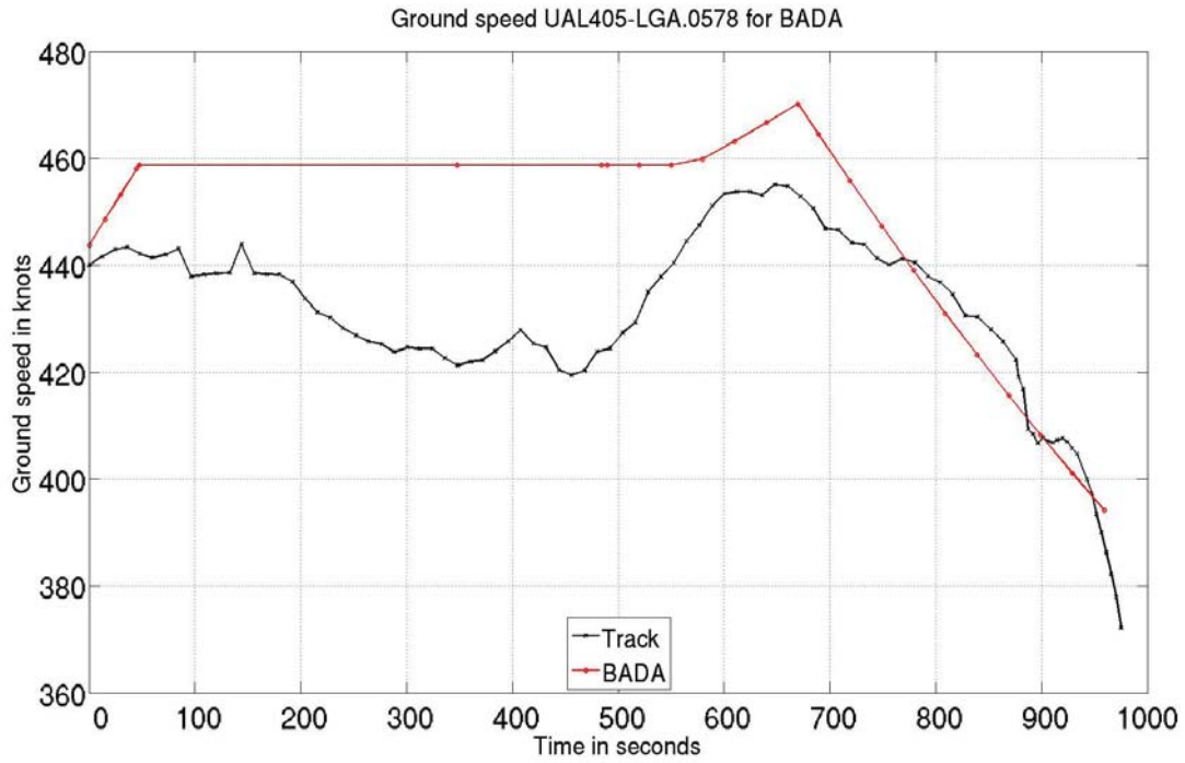
Figure 43. Boeing 757-200 BADA Base Case idle descent: ground speed
