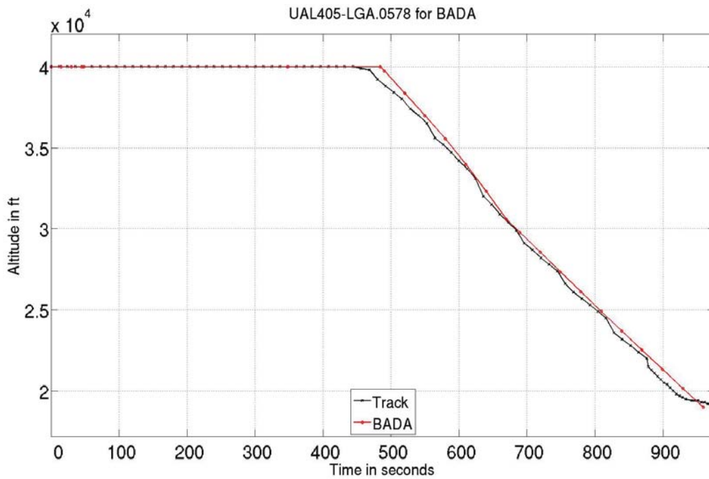
Figure 44. Boeing 757-200 BADA Base Case idle descent: altitude
