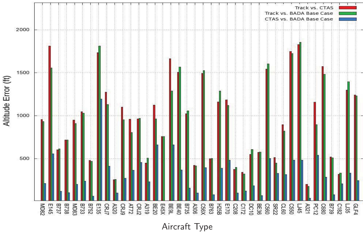
Figure 7. Mean of absolute mean altitude errors
