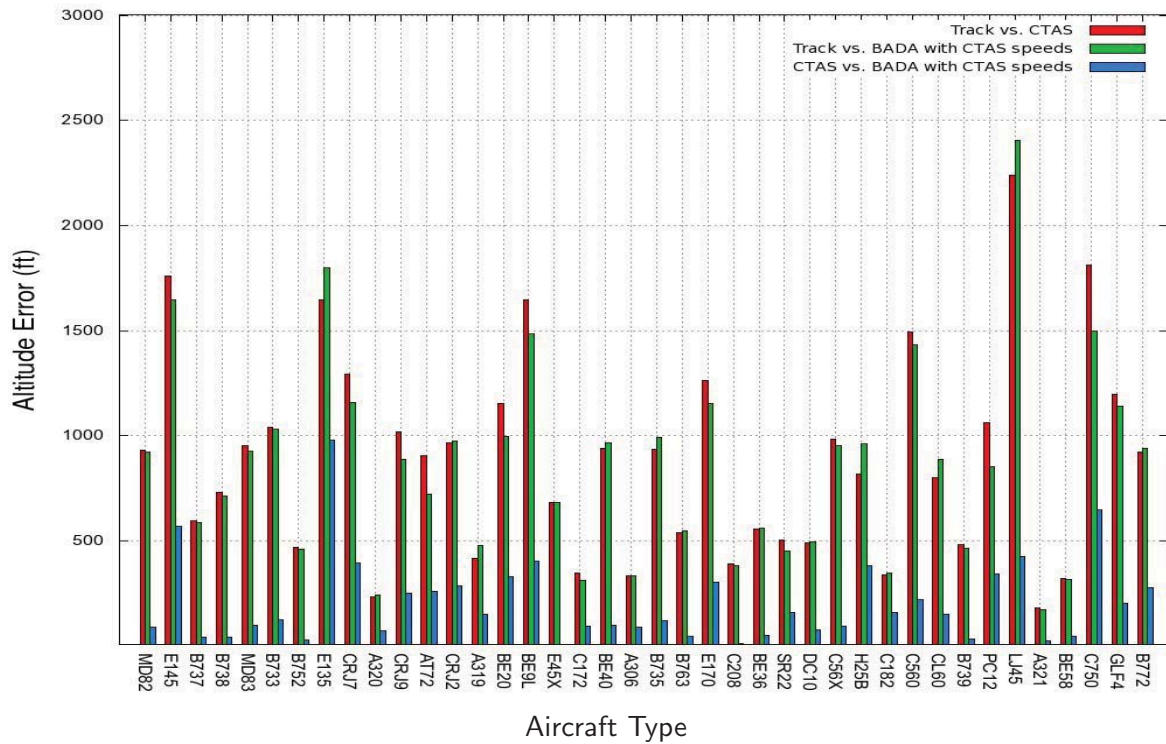
Figure 33. Mean of absolute mean altitude errors for BADA with CTAS speeds
