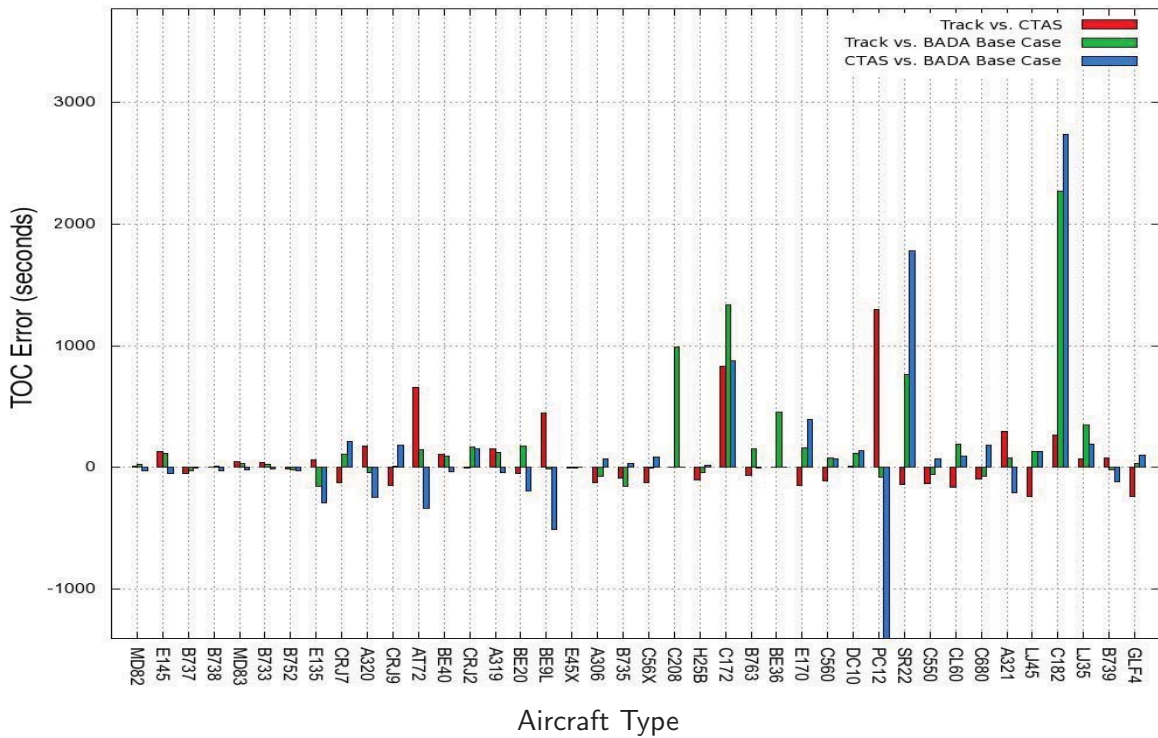
Figure 9. Events, Mean of mean TOC time errors
