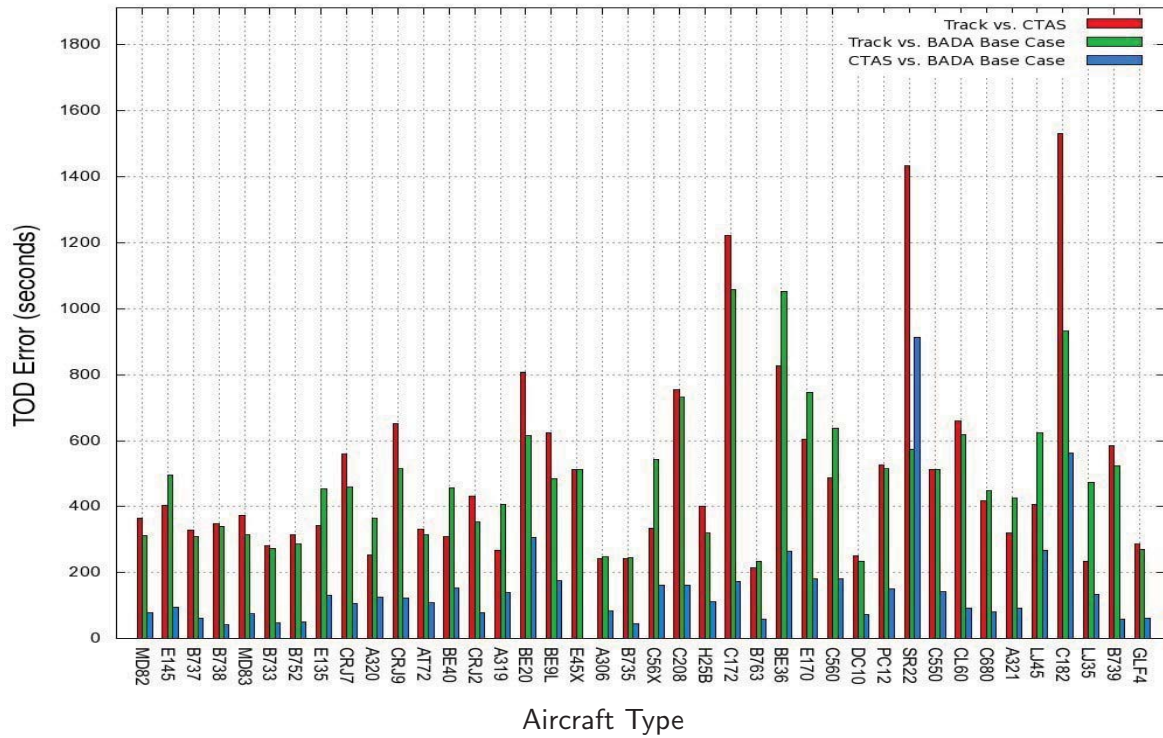
Figure 12. Events, Mean of absolute mean TOD time errors
