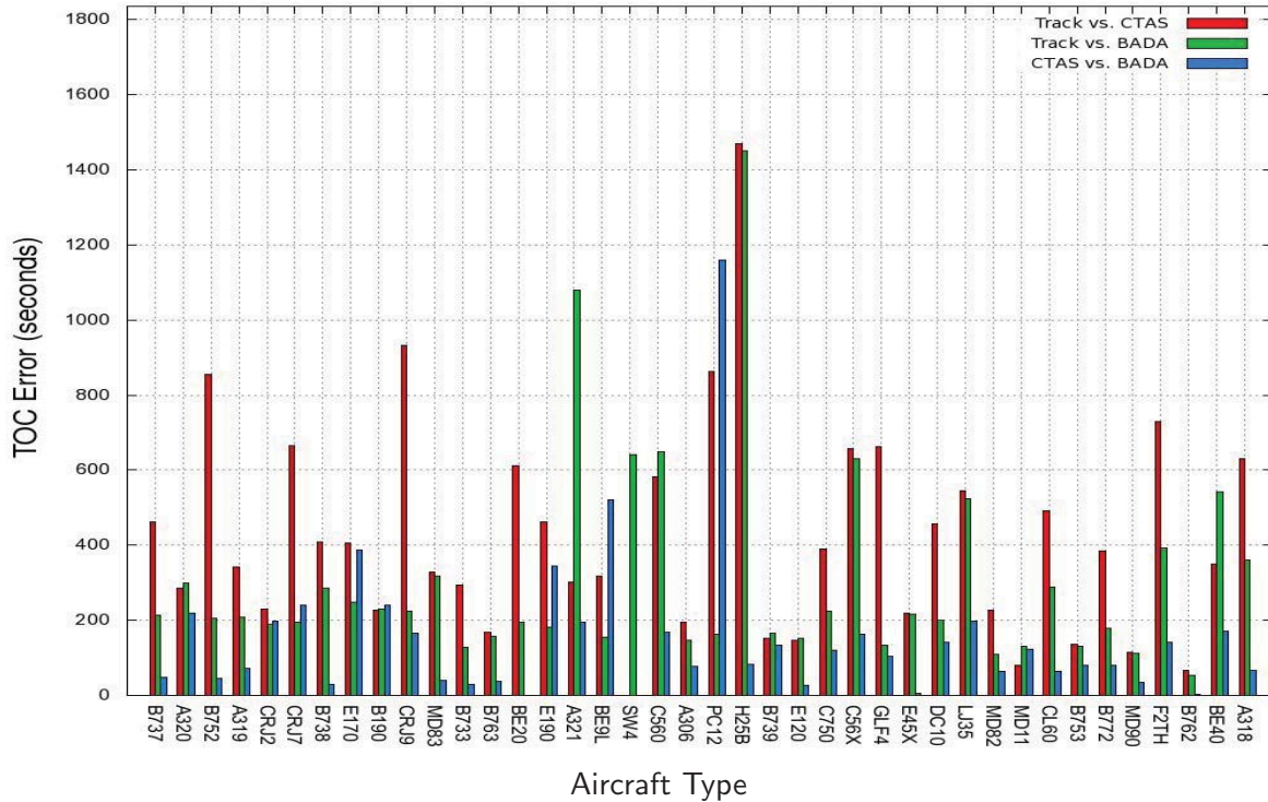
Figure 42. Mean of absolute mean TOC time errors in Denver center
