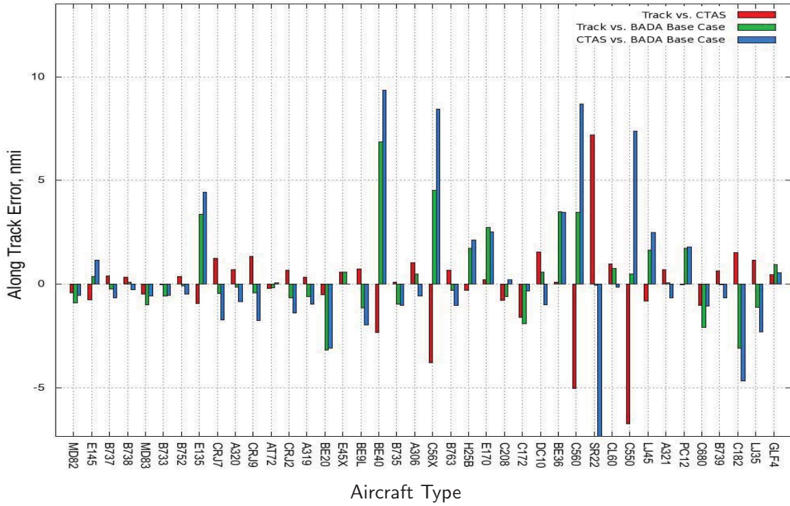
Figure 8. Mean of mean along-track errors
