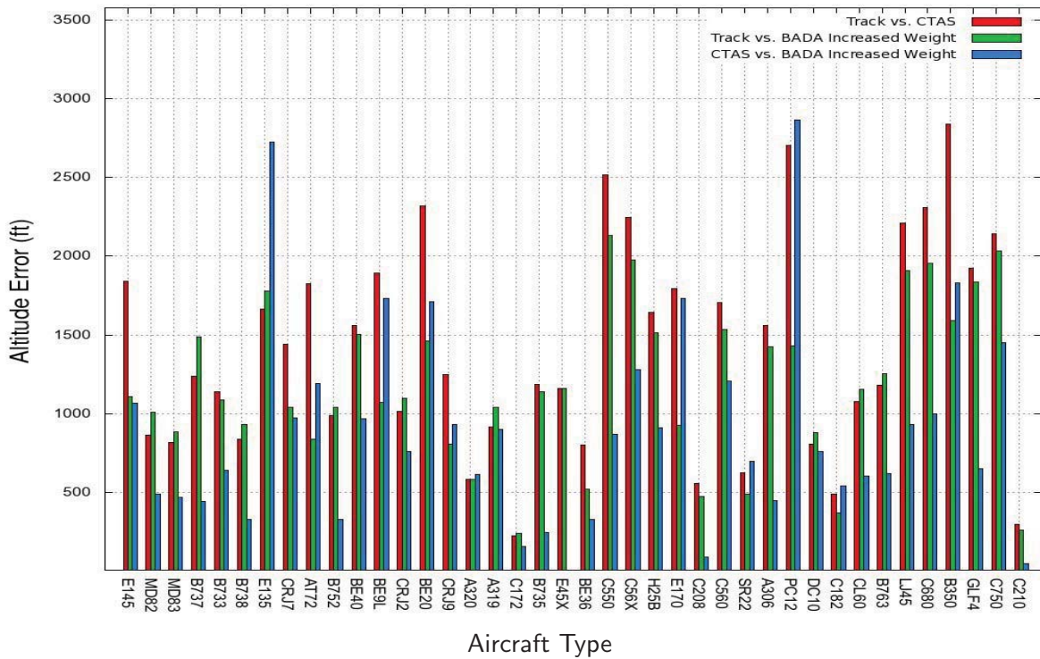
Figure 31. Mean of absolute mean altitude errors in climb, BADA Increased Weight
