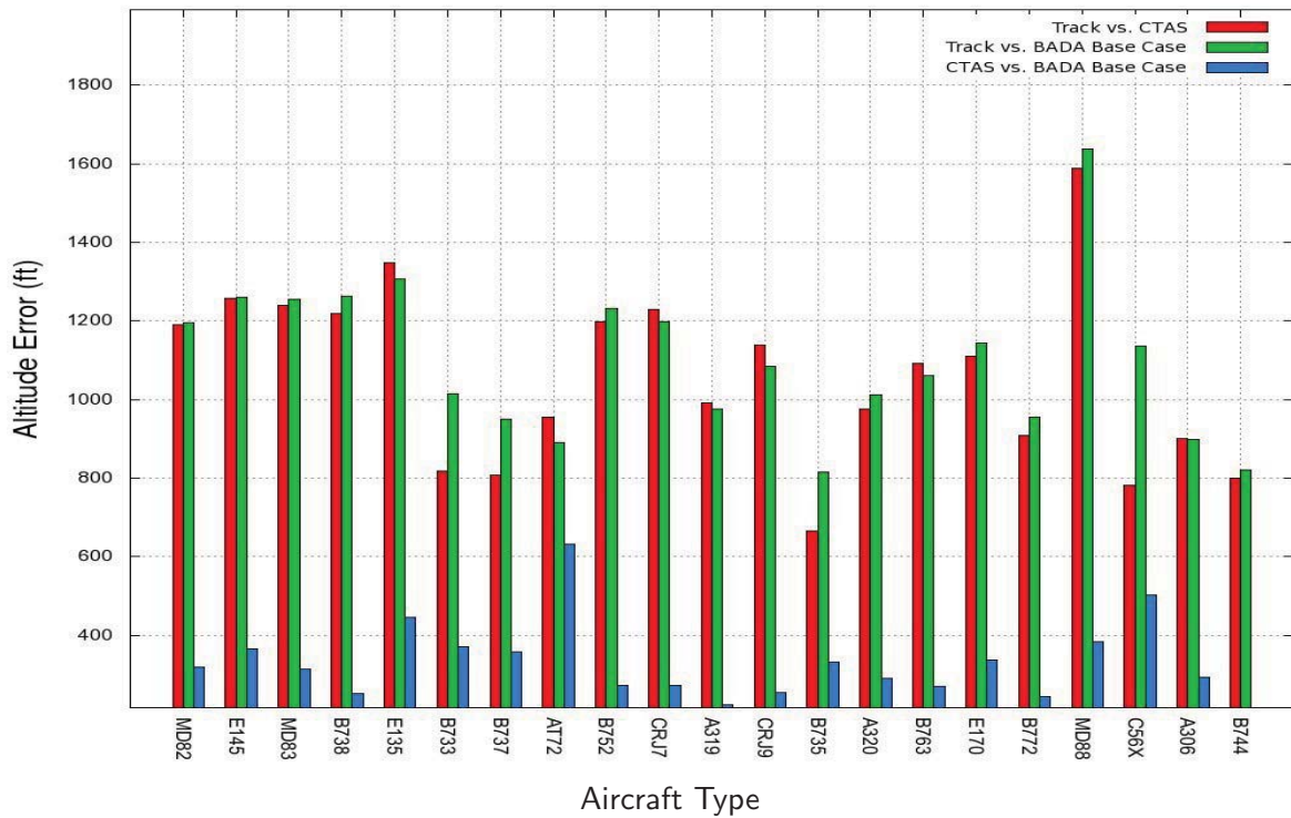
Figure 23. Mean of absolute mean altitude errors, TRACON only
