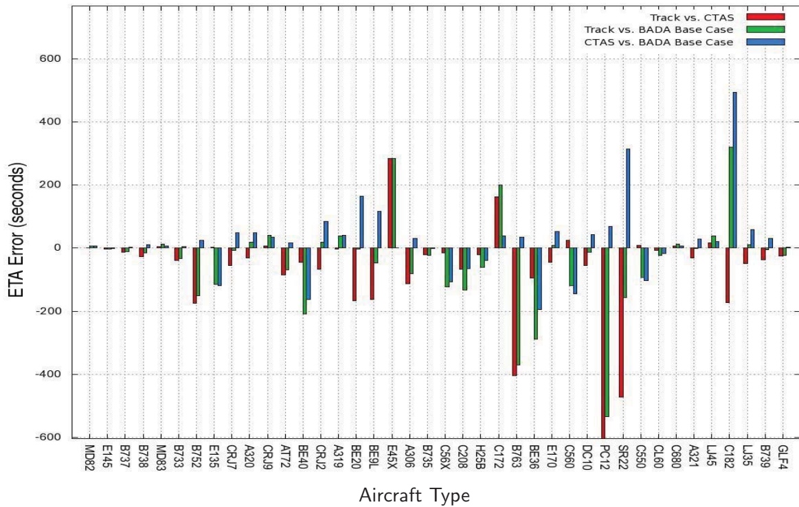
Figure 13. Events, Mean of mean ETA time errors
