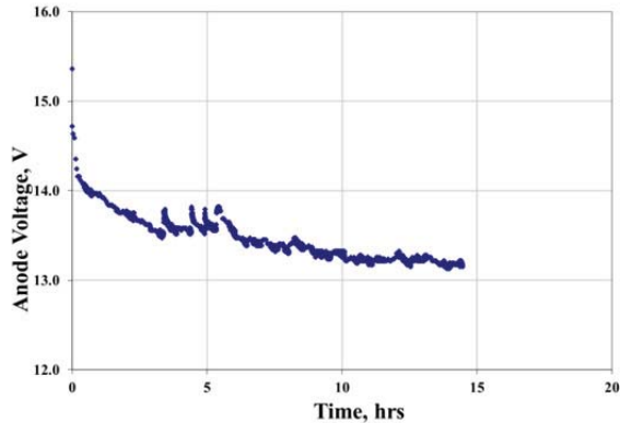
Figure 17.—HCA.001-F anode voltage profile during segment 112.
