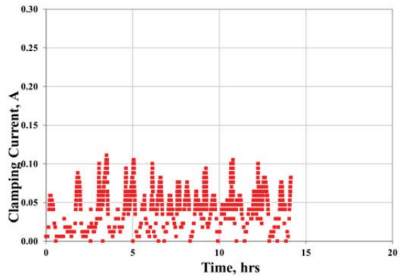
Figure 12.—HCA.001-F clamping current profile during segment 123.
