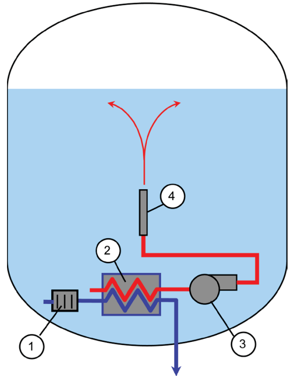
Figure 1.—Simplified schematic of thermodynamic vent system (TVS) hardware: 1—Joule-Thomson device, 2—Heat exchanger, 3—Liquid recirculation pump, 4—Axial jet (or alternatively, a spray bar).
