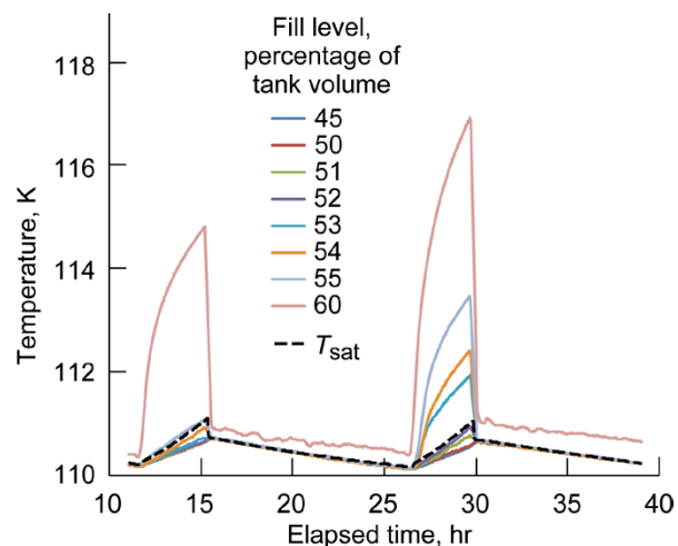
Figure 23.—Liquid-ullage interface temperatures during Test 50A thermodynamic vent system (TVS) cycles; T_{sat} , temperature of saturated vapor.
