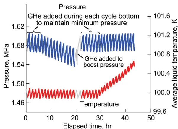
Figure 43.—Tank pressure and average liquid temperature for Test 50E; GHe, gaseous helium.
