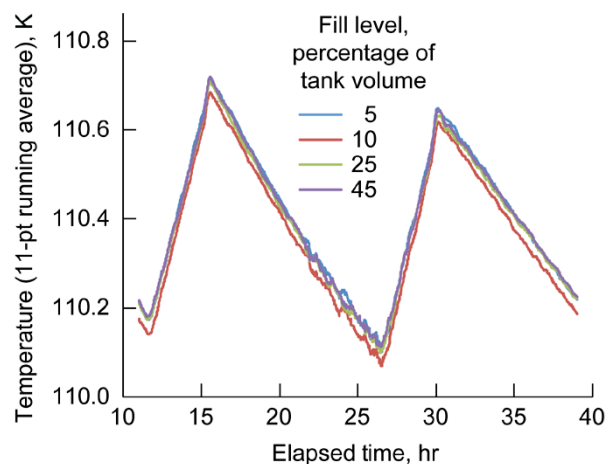
Figure 22.—Liquid temperatures during Test 50A thermodynamic vent system (TVS) cycles.
