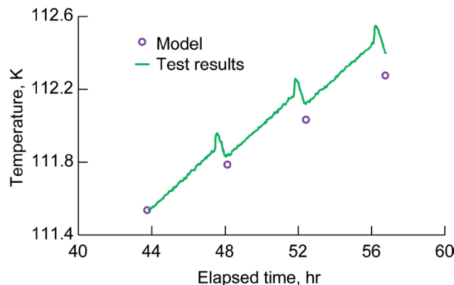
Figure 51.—Comparison of model predictions with data at 90-percent fill with pressure control.
