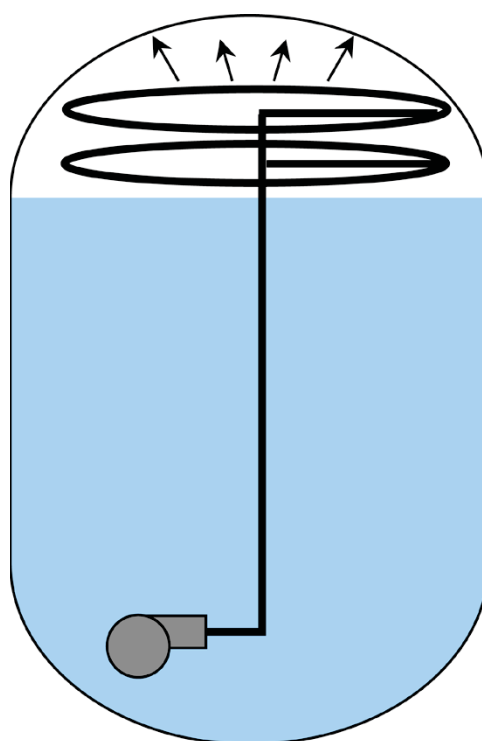
Figure 8.—Spray hoops.
