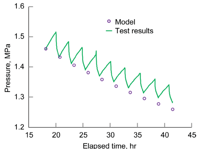
Figure 50.—Comparison of model predictions with data at 90-percent fill with temperature control.
