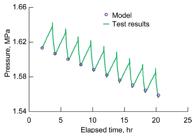
Figure 52.—Comparison of model predictions with data at 50-percent fill with temperature control.
