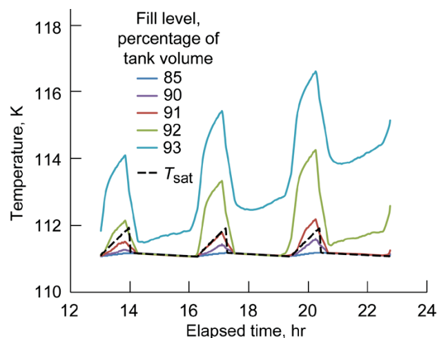
Figure 20.—Liquid-ullage interface temperatures during Test 90A thermodynamic vent system (TVS) cycles; T_{sat} , temperature of saturated vapor.
