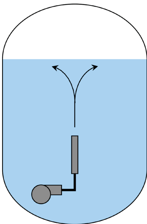
Figure 7.—Axial jet.
