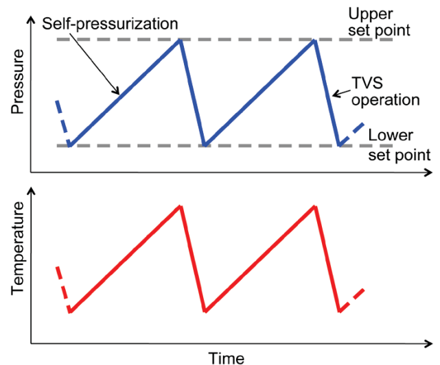
Figure 2.—Idealized thermodynamic vent system (TVS) operational control for a system of pure liquid propellant and its vapor.
