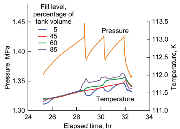
Figure 40.—Pressure and liquid temperatures for pressure-controlled operation in Test 90D.
