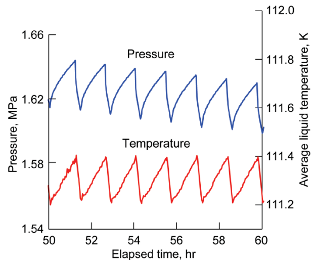
Figure 28.—Closeup of seven temperature-controlled pressure and temperature cycles for Test 50B.
