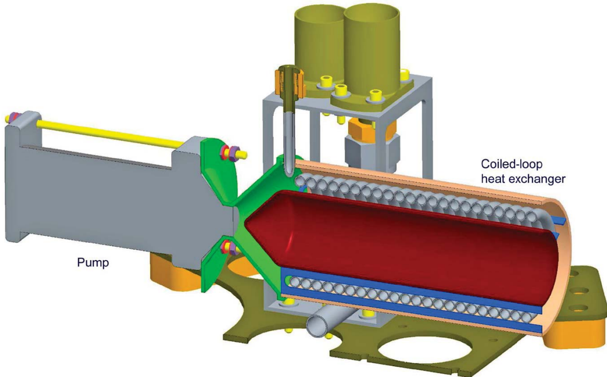
Figure 12.—Thermodynamic vent system (TVS) heat exchanger and pump assembly.
