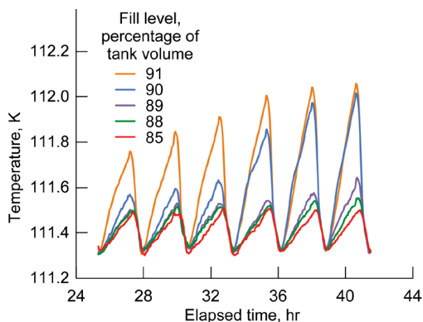
Figure 32.—Liquid-ullage interface temperatures during Test 90C thermodynamic vent system (TVS) cycles.
