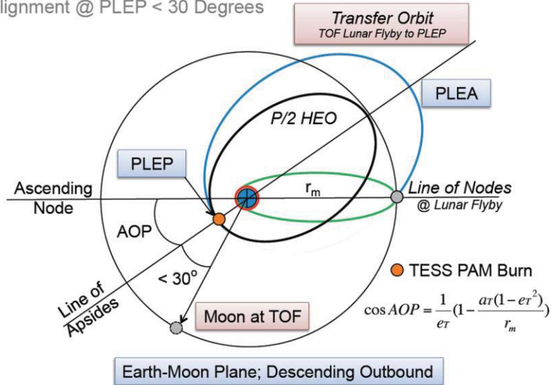
Figure 2. Diagram of the trajectory events [1]. The Translunar Injection (TLI) segment (green) sends the spacecraft to lunar flyby. Following flyby, TESS travels on the Transfer orbit (blue) that delivers it to the Science orbit (black).
