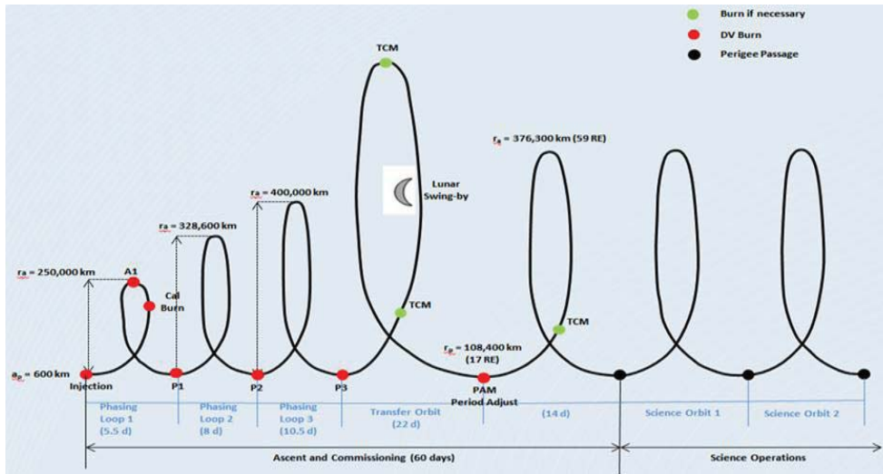
Figure 1. TESS mission timeline. There are three phasing loops, followed by a Translunar Injection maneuver that sends the spacecraft to a lunar flyby. The flyby raises perigee to mission altitude. At the next perigee, a Period Adjust Maneuver (PAM) is performed to place TESS in a 2:1 resonant orbit with the Moon.
