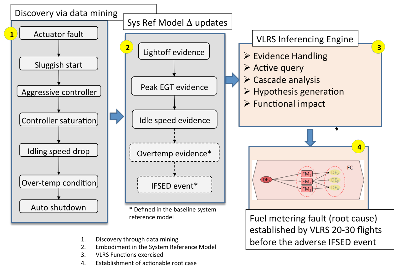
Figure 5. Impact of VLRS on detecting events that led to an in-flight engine shutdown
