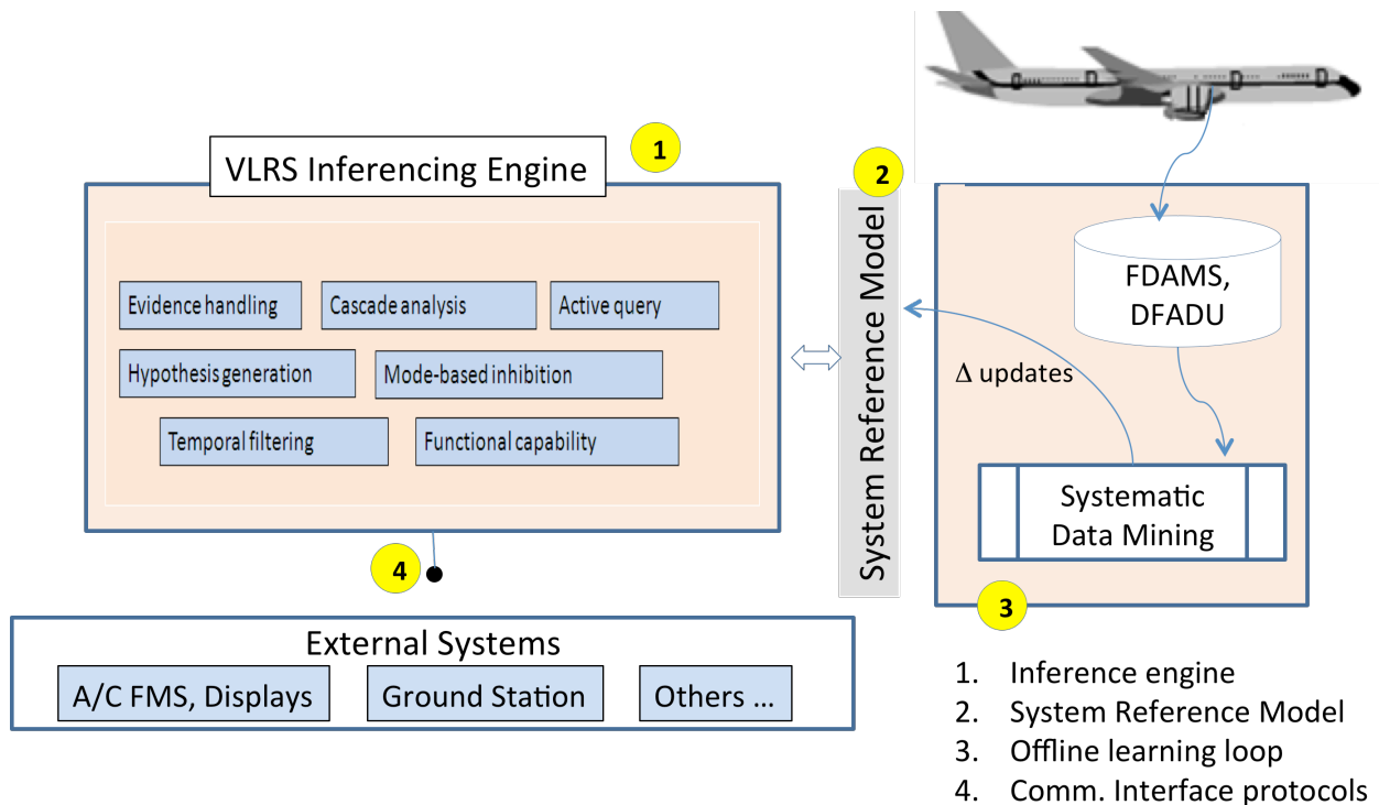
Figure 2. Functional modules in a Vehicle-Level Reasoning System.
