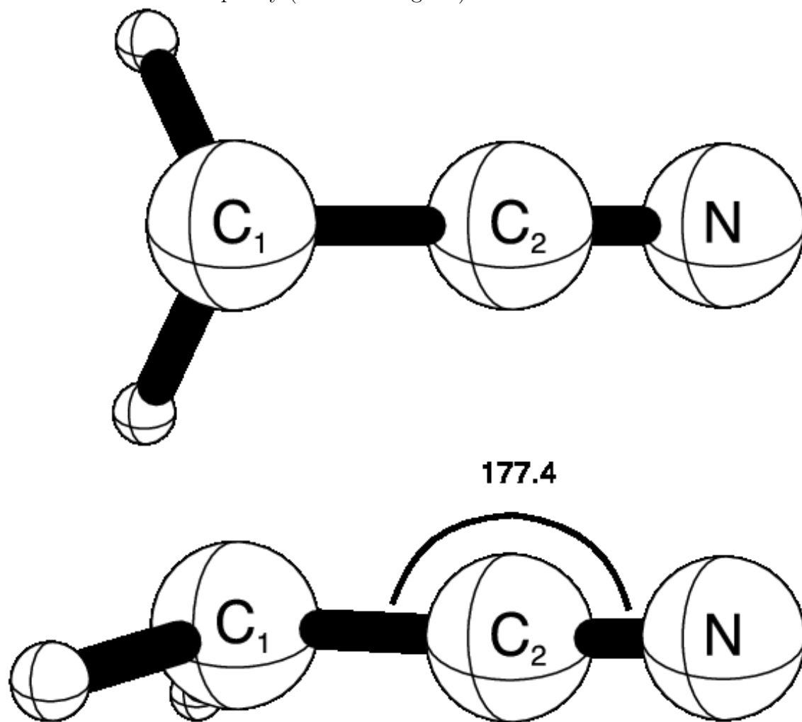
Fig. 1.— Top-down and side-on views for the CcCR equilibrium geometry of \tilde{X}^1A' \text{CH}_2\text{CN}^- . \angle\text{C}-\text{C}-\text{N} is shown explicitly (units are degrees) in the lower side-on view.
