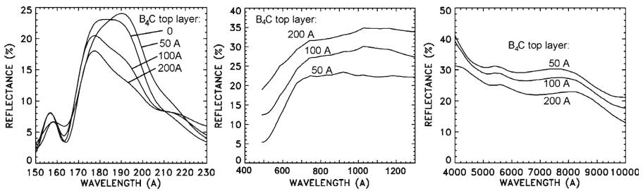
Fig. 11 LEMUR broadband Mo/Si multilayer mirror coating with B 4 C top layer with thicknesses of 50, 100 and 200 Å. The reflectance is shown for the SW band ( left ), LW band ( middle ), and the Vis-NIR range ( right )
