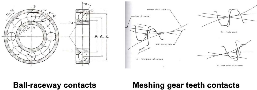
Figure 1-Hertz concentrated contacts in bearings and gears.
