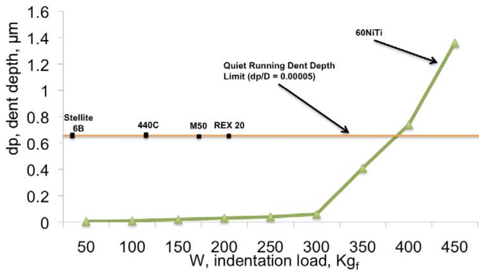
Figure 4 -Indent depths for 60NiTi plate as a function of load when contacted by a 12.7mm diameter Si 3 N 4 indenter ball. Data for Stellite 6B, 440C, M50 and REX20 from References 4, 5.
