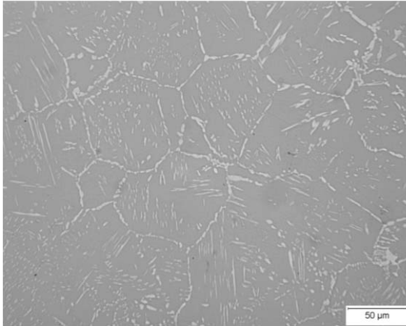
As-received 60NiTi (lighter phase is Ni 3 Ti).
