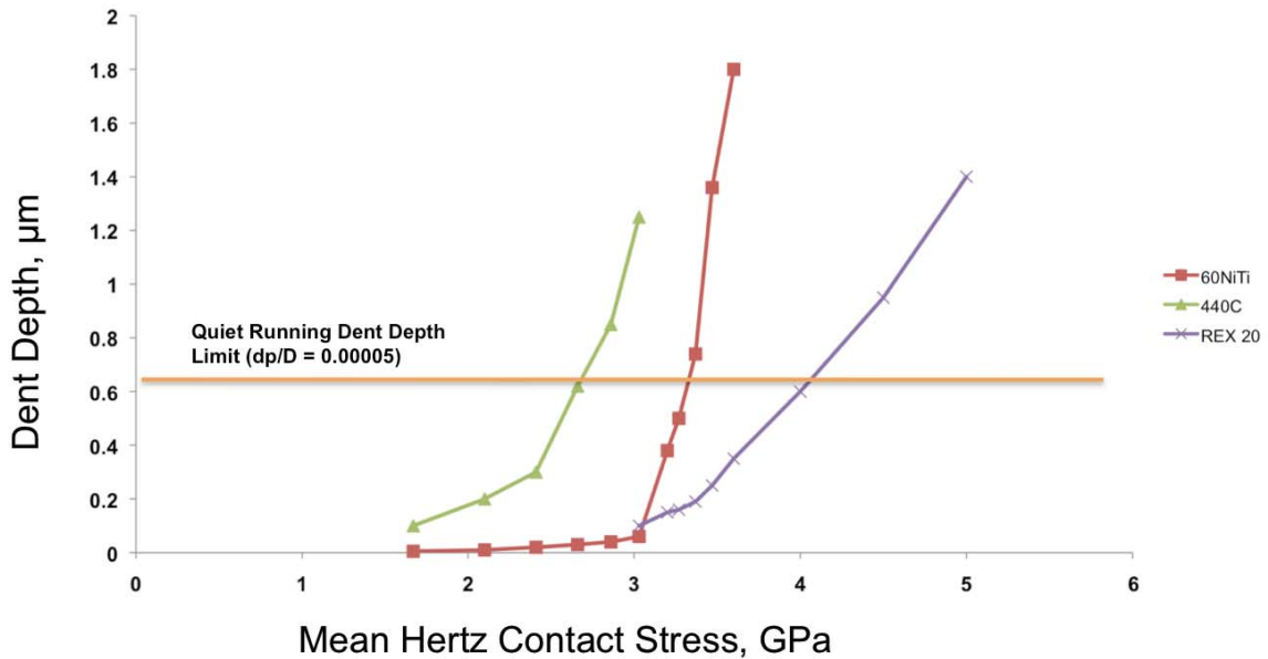
Figure 3 -Indent depths as a function of contact stress for 60NiTi, 440C and REX20 plates loaded
