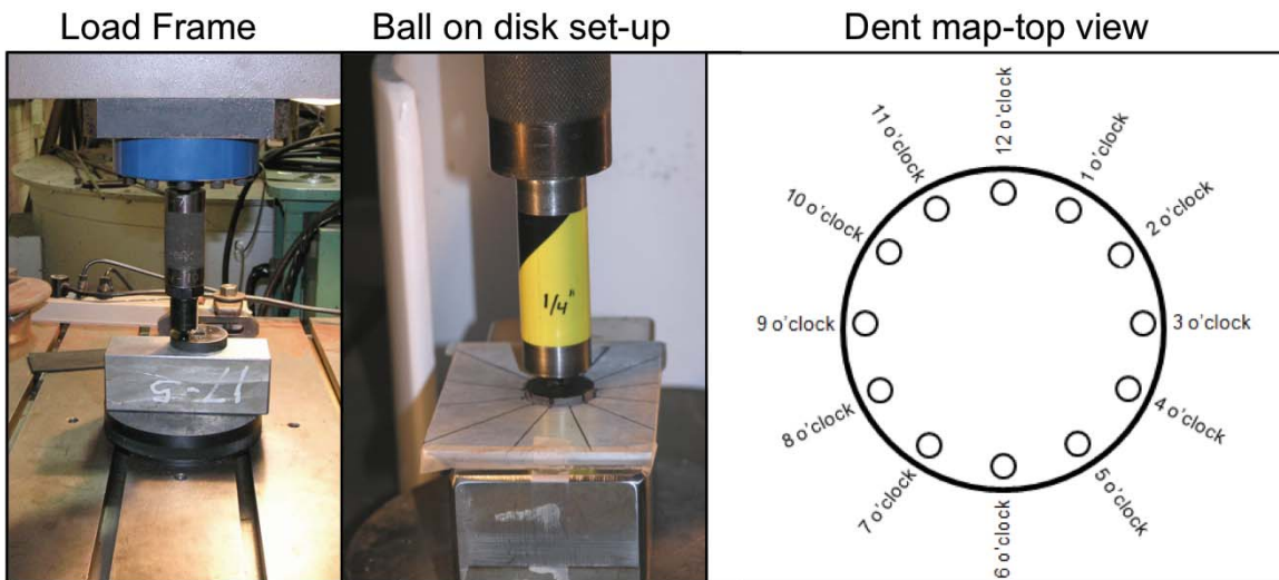
Figure 7- Brinell test configuration used for indentation experiments to measure static load capacity.
