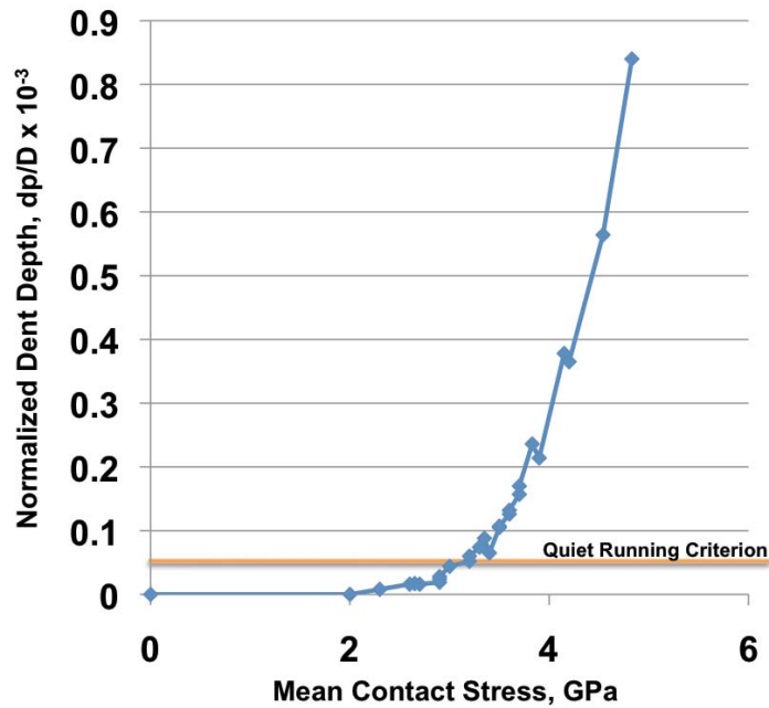
Figure 9- Normalized dent depth (dp/D) versus mean contact stress for polished 60NiTi plate indented with Si 3 N 4 balls ranging in size from 6.35 to 12.7mm diameter.
