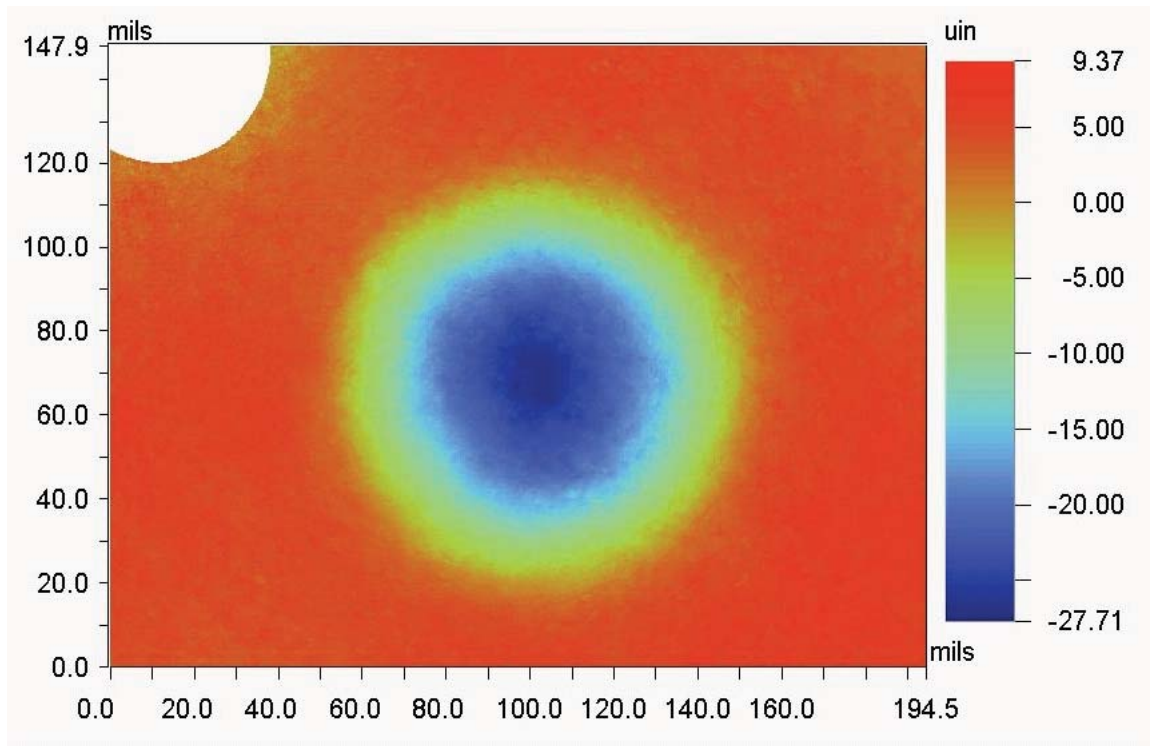
Figure 8- Topographical contour plot of dented 60NiTi surface as measured by optical (non-contact) surface profilometry.
