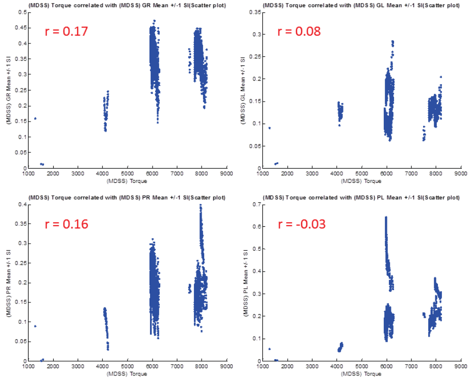
Figure 24. Correlation Between \pm 1 Average Sideband (SI1) and Torques.
