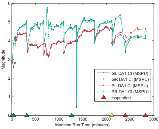
Figure 14: MDSS and MSPU DA1.
