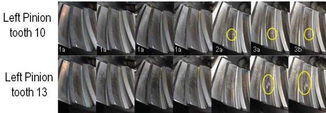
Figure 5: Left Pinion Tooth Damage.
