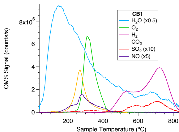
Figure 1. Major volatiles evolved during Cumberland EGA analysis. O 2 from soil oxidants evolves <550°C and is used as the O 2 source for step 1 of the combustion experiment. CO 2 and H 2 O captured <550°C are sent to the TLS for isotopic analysis. In step 3, H 2 from clay dehydroxylation >550°C is combusted to H 2 O to get a total high temperature water δD value. SO 2 is also evolved >550°C from sulfate decomposition.
