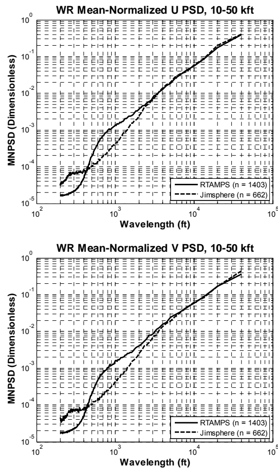
Figure 2: Mean-normalized power spectral density (PSD) for the WR Jimsphere and RTAMPS rawinsonde systems.
