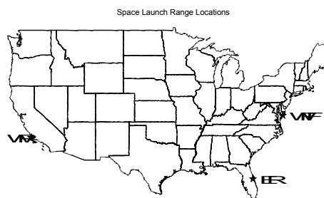
Figure 1: Location of space launch ranges where temporal wind pair databases were developed.
