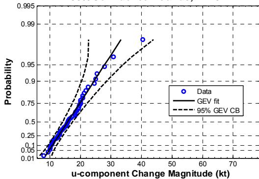
WFF Maximum 1.5-hr u-component Change Magnitudes with Generalized Extreme Value Fit and 95% Confidence Bounds, n = 54
