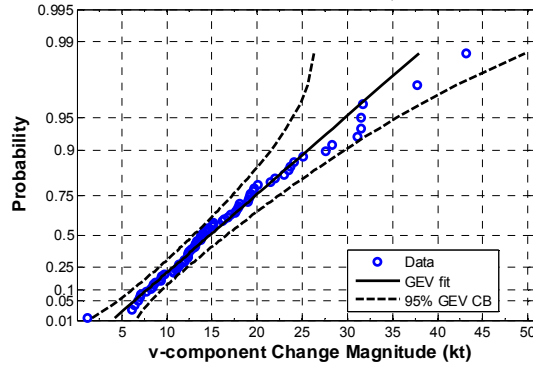
Figure 4: Illustration of a large spread in the 95% CB associated with a small sample population. Maximum wind change from the 1.5-hr wind pairs at WFF with 95% CB for the u-(top) and v-component (bottom) wind changes. The magnitude of the wind component change is on the x-axis and probability is on the y-axis. The number of pairs (n) in the analysis is 54.
