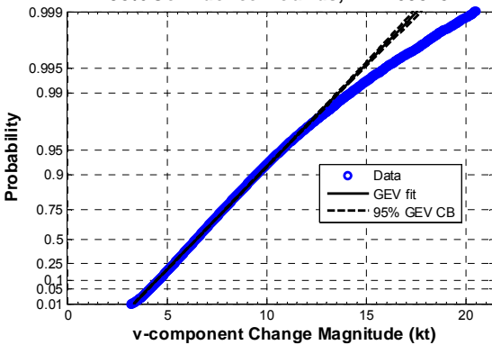
Figure 3: Illustration of a narrow spread in the 95% CB associated with a large sample population. Maximum wind change from the 1.5-hour wind pairs at the ER with 95% CB for the u-(top) and v-component (bottom) wind changes. The magnitude of the wind component change is on the x-axis and probability is on the y-axis. The number of pairs (n) in the analysis is 260,878.
