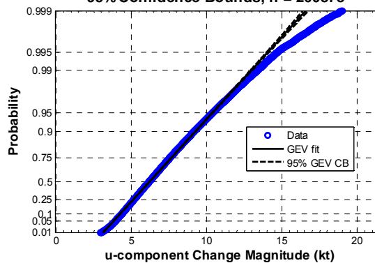
ER Maximum 1.5-hr u-component Change Magnitudes with Generalized Extreme Value Fit and 95% Confidence Bounds, n = 260878
