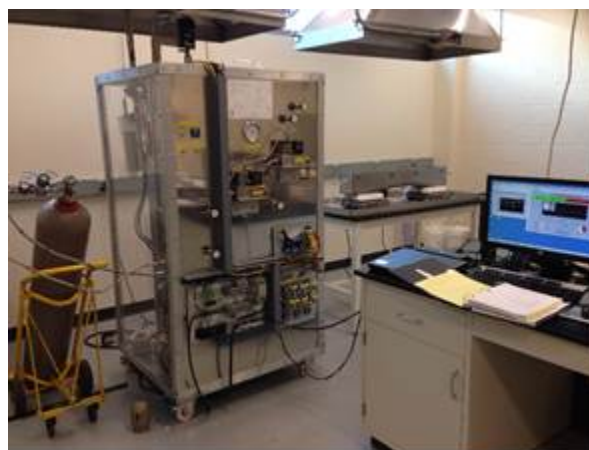
Figure 1. CVD system.
