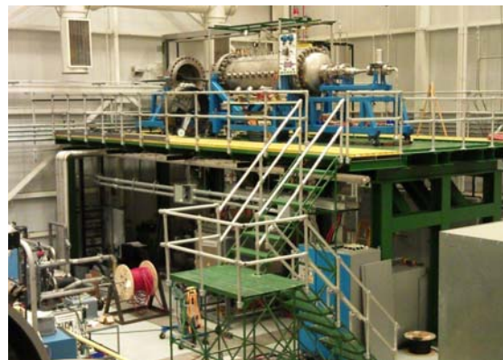
Figure 1. Current NTREES Configuration
