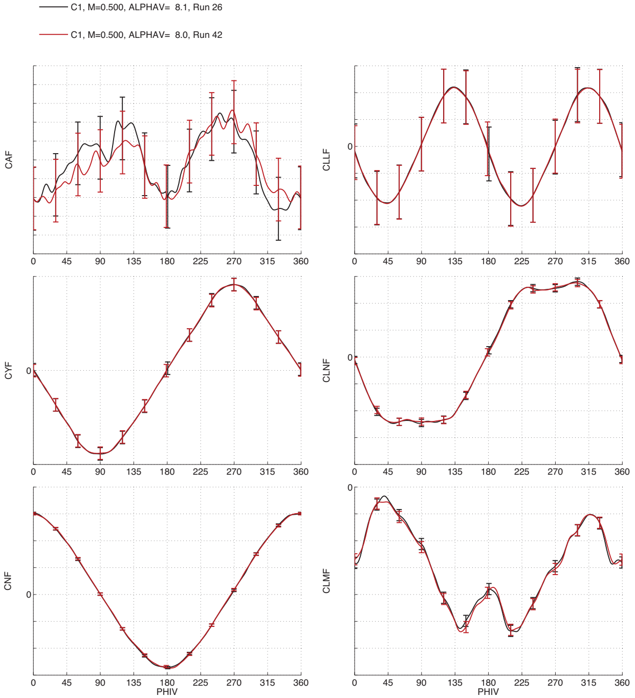
Figure 9. SLS-10003 forebody force and moment coefficients for 2 repeat continuous roll sweeps at M=0.5 , \text{ALPHAV}=8^\circ , moment reference at the balance moment center, error bars represent uncertainty due to balance calibration
