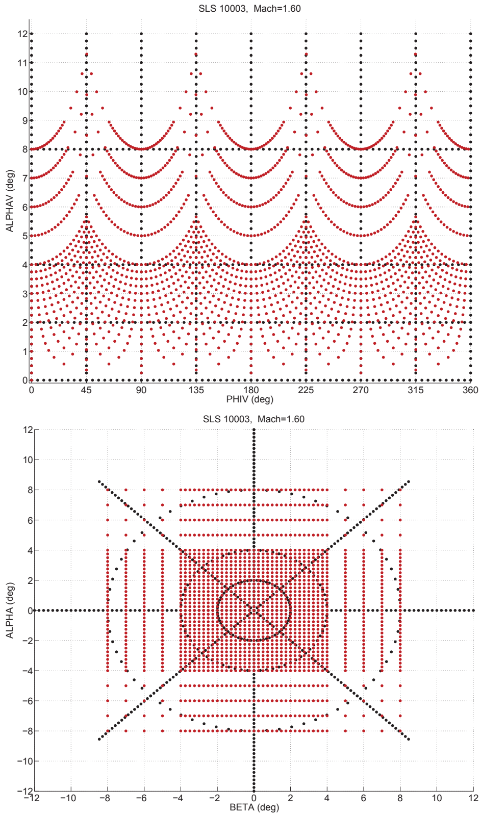
Figure 16. Wind tunnel post-processed data breakpoints (black circles), and database breakpoints (red circles), in the ALPHAV/PHIV space (top) and in the ALPHA/BETA space (bottom)
