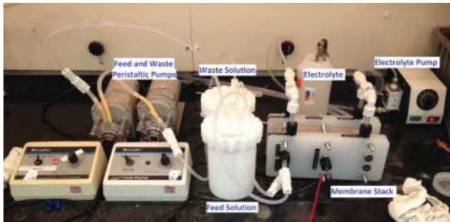
Image of the experimental apparatus used to test the chloride and fluoride removal capabilities of the electro dialysis stack
