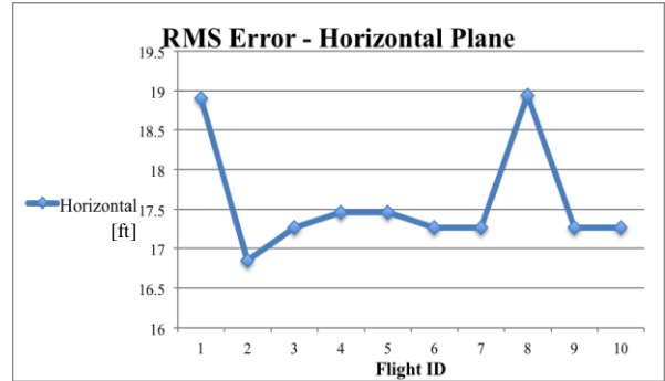
Fig. 3 RMS Error on the Horizontal plane
