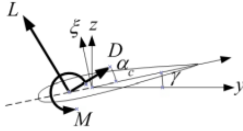
Fig. 10 - Airfoil Forces and Moment
