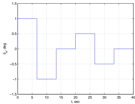
Fig. 21 - Elevator Doublet
