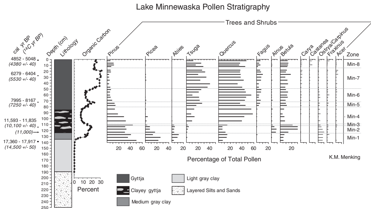
Fig. 2. Lithology and pollen stratigraphy of the Lake Minnewaska core. Sediments below 140 cm are nearly devoid of organic matter and yielded insufficient pollen grains for analysis. Depths of AMS radiocarbon dates and organic carbon content are also shown. Bold italicized date in parentheses and denoted with an arrow marks the regional onset of the Younger Dryas cooling event.
