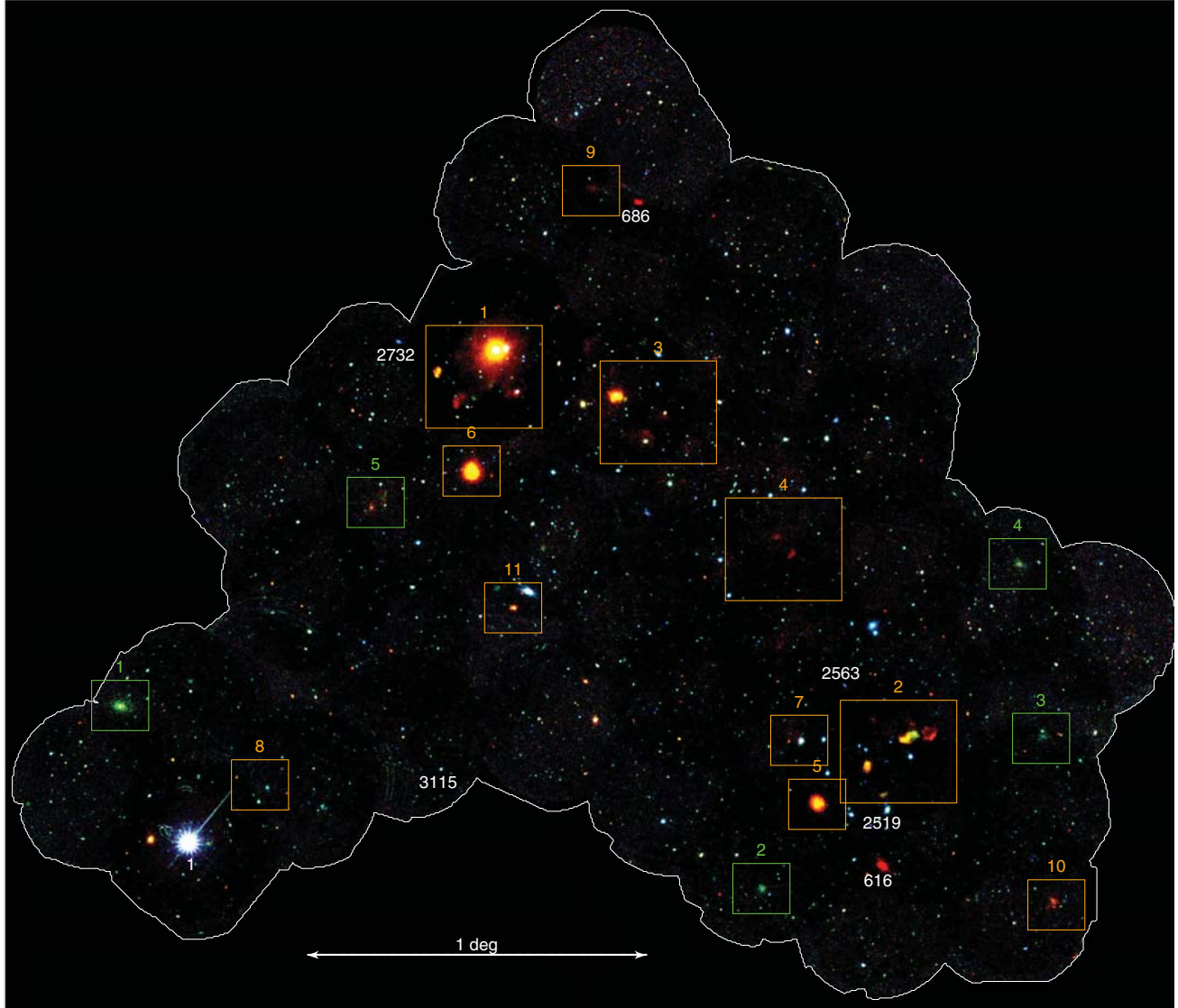
Fig. 5. Combined EPIC pn and MOS mosaic image of the SMC region centred at RA = 01:00:30, Dec = -72:28:00 (J2000). The RGB colour image is composed of the three energy bands 0.2–1.0 keV (red), 1.0–2.0 keV (green), and 2.0–4.5 keV (blue) (exposure-corrected and for EPIC pn out-of-time event subtracted, but not detector-background subtracted and not vignetting-corrected). The boxes mark fields with SNRs (orange) and galaxy clusters (green), which are shown in more detail in Figs. 6 and 9. Several X-ray sources, which are mentioned in the text, are marked in white with their catalogue number from Sturm et al. (2012b) : 686 the planetary nebula SMP SMC 22; 616 the symbiotic binary SMC 3; 1 the super-giant HMXB SMC X-1; 2519, 2563, 2732, and 3115 new Be/X-ray binaries.
