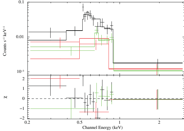
Fig. 7. EPIC pn (black) and MOS (red and green) spectra of the candidate SNR XMMU J0056.5–7208 extracted from observation 0601210601 (with net exposures of 29.6 ks and 34.1 ks, respectively). Top : data with best-fit Sedov model as histogram, bottom : residuals in units of sigma.
