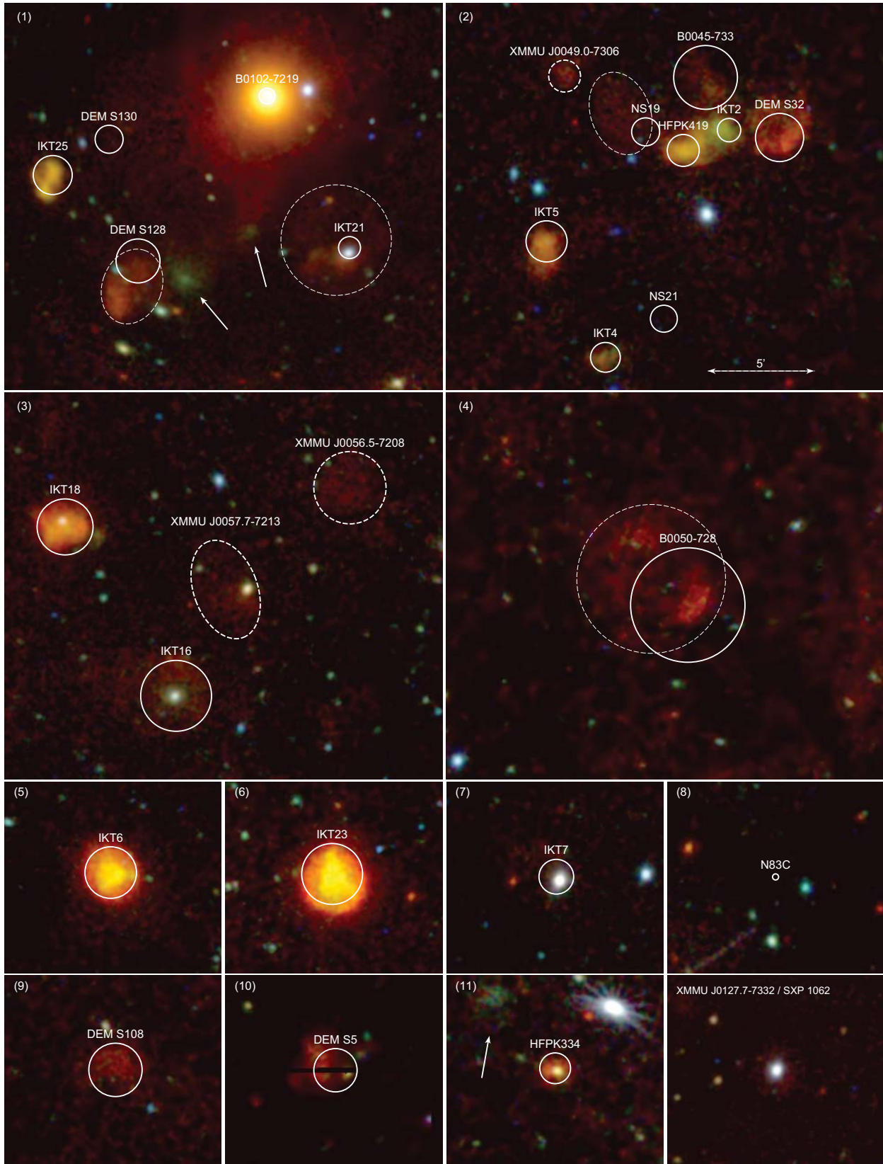
Fig. 6. Supernova remnants in the SMC as seen by EPIC. Colours represent the same energy bands as in Fig. 5 and the panels are numbered according to Fig. 5. To more clearly reveal faint diffuse emission, all images were detector background-subtracted and both exposure- and vignetting-corrected and are shown with the scale indicated in the upper right . For a description of the markings see Sects. 2.1 (SNRs) and 2.2 (galaxy clusters). The bottom right panel shows the only known SMC SNR (Haberl et al. 2012) not covered by our survey.
