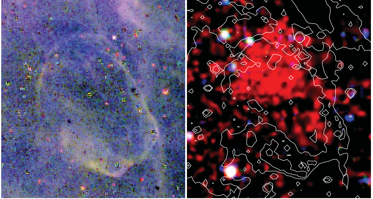
Fig. 8. The region around XMMU J0056.5–7208. Left: zoom-in of the MCELS image from Fig. 4. Right: zoom-in of the X-ray image from Fig. 6, panel 3 with enhanced contrast. The contours mark the summed H\alpha , [S II] , and [O III] intensity at 100 and 150 \times 10^{-17} \text{ erg cm}^{-2} \text{ s}^{-1} .
