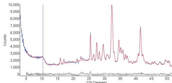
Figure 2: 1D XRD pattern of John Klein with observed (blue) versus calculated (red) patterns, and difference curve at the bottom (gray). Vertical line marks the smectite 001 diffraction maximum at \sim 10^\circ .
