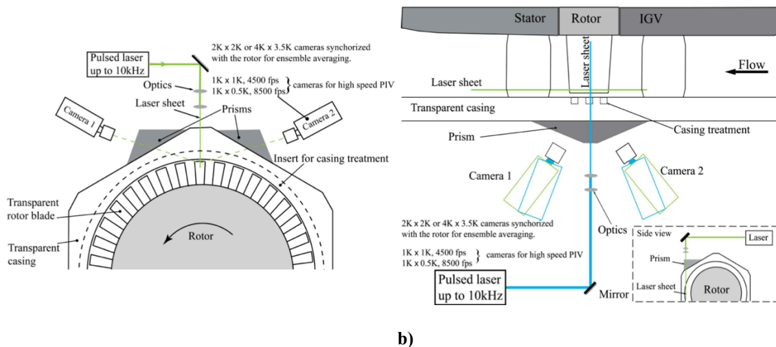
Figure 8. Stereo PIV setup for a) axial and b) blade-to-blade planes.
