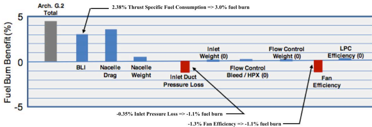
Figure 30. Results from a system study indicating potential fuel burn benefits of BLL propulsion 17 .
