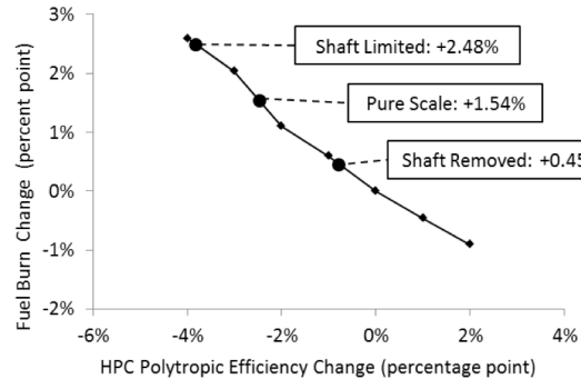
Figure 24. Fuel burn impact as a function of HPC polytropic efficiency and scaling options 10 .
