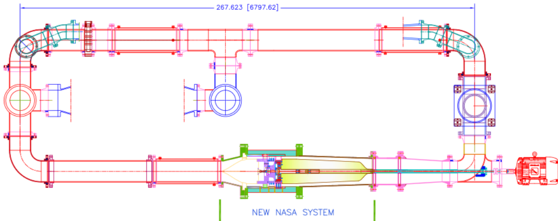
Figure 4. The JHU turbomachinery facility with the new NASA compressor setup installed.
