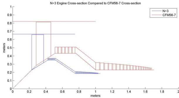
Figure 21. Scaling CFM56-7 to future (denoted N+3) engine size 10 .
