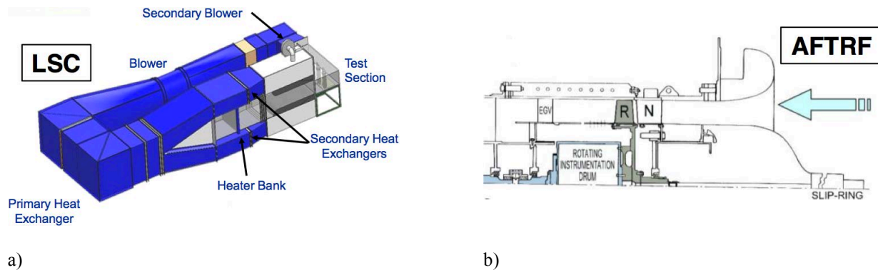
Figure 16. (a) PSU low speed cascade (LSC), and (b) axial flow turbine research facility (AFTRF).
