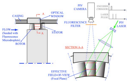
Figure 12. Volumetric illuminating PIV.
