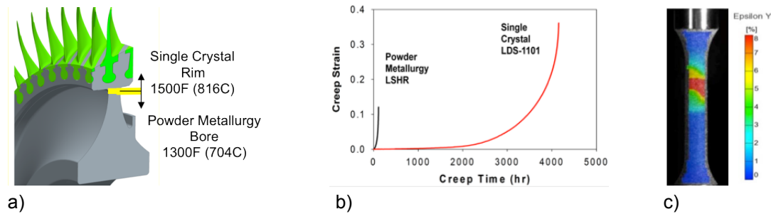
Figure 25. (a) Schematic of a hybrid disk , (b) Creep resistance of LDS alloys required for 816 °C (1500 °F) disk rim temperatures and (c) 3D strain mapping of PM/SX joint indicating most deformation occurs in the single crystal region 11 .
