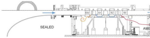
Figure 10. Meridional view of the Purdue 3-1/2 stage research compressor.
