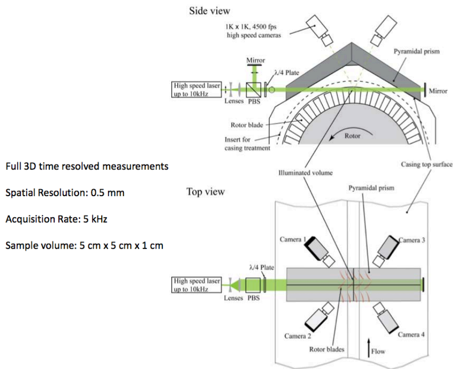
Figure 9. Setup of Tomographic PIV system.
