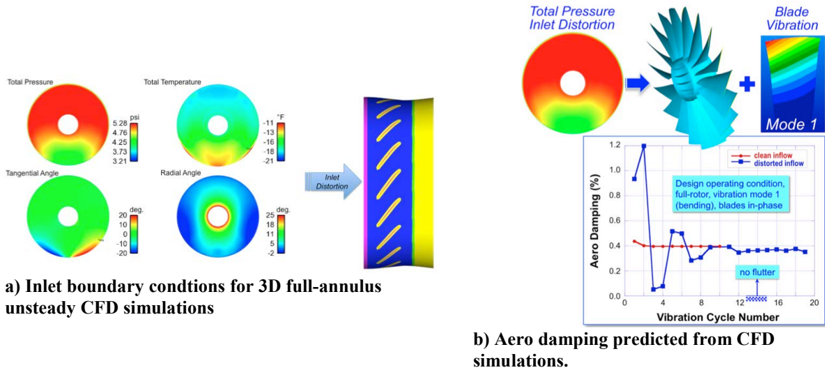
Figure 33. NASA high fidelity CFD for eromechanical analysis of UTRC designed distortion tolerant fan.
