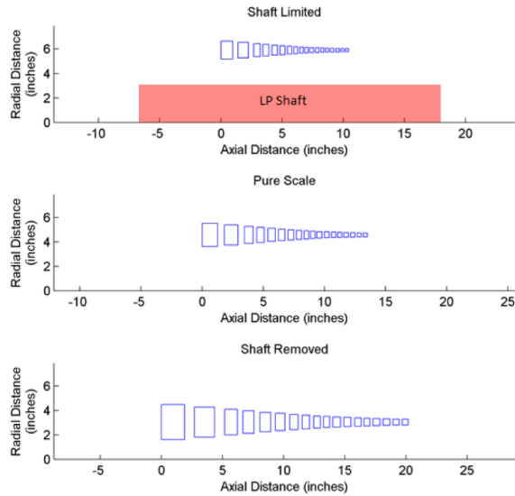
Figure 23. Impact of different scaling dependent on shaft constraint 10 .
