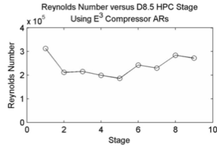
Figure 22. Reynolds number in D8.5 HPC stages 10 .
