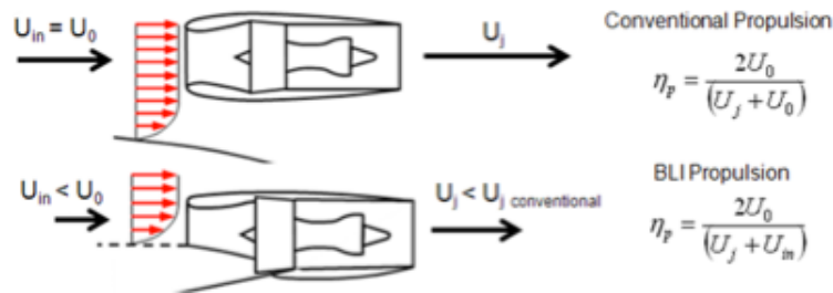
Figure 29. Propulsive efficiency benefit from BLI v.s. conventional propulsion 6 .
