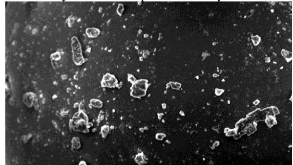
Figure 3. Sulfate weathering products produced during olivine weathering experiments at -40^{\circ} C. Experimental duration was 2 weeks. All particles in field of view are sulfate minerals.
