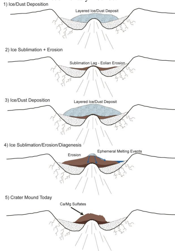
Figure 2. Sketch model for the formation and evolution of martian sedimentary mounds.
