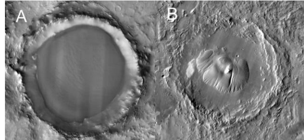
Figure 1. THEMIS Daytime Infrared Image of (A) Korolev Crater and (B) Nicholson Crater on Mars. Image credit: ASU/NASA/JPL.
