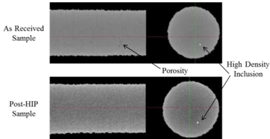
GRC computed tomography of an as-received Ti-6Al-4V tensile sample and following hot isostatic pressing (HIP) confirming closure of porosity by HIP post-processing (GRC)
