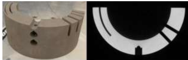
Photography (left) and computed tomography (right) of a direct metal laser sintered POGO-Z aluminum gauge black (MSFC).
