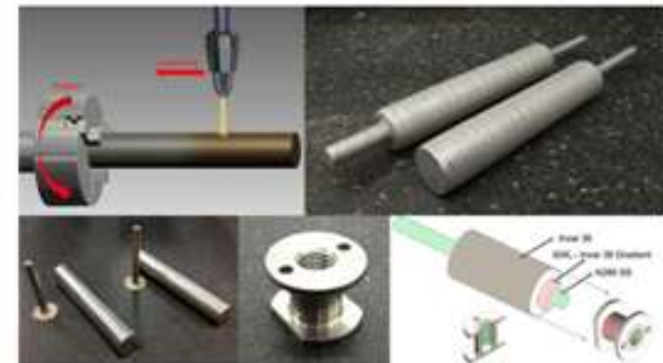
Stainless steel-Invar radial gradient alloys
