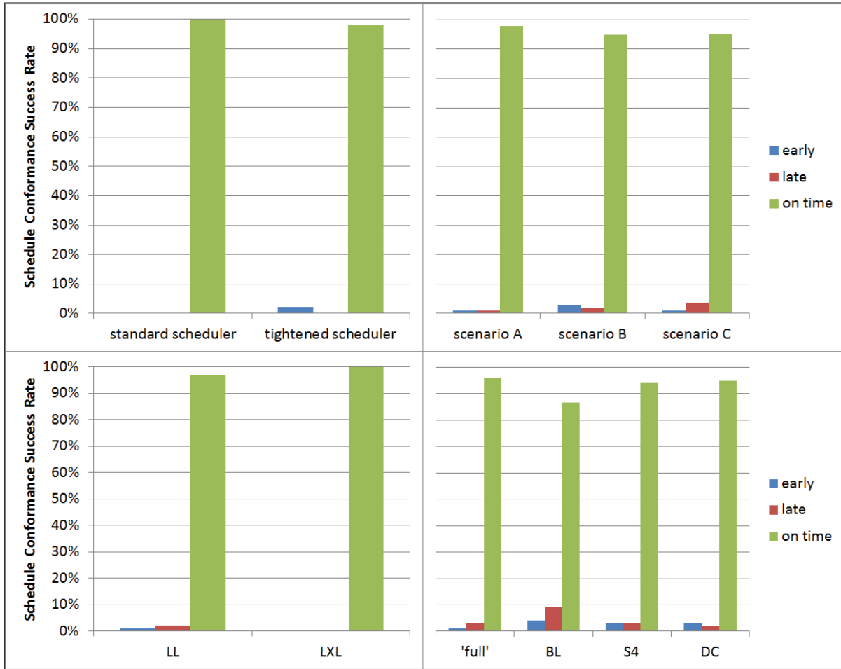
Figure 14. Percentage of aircraft delivered to the meter-fix either early, late, or on time, as reported in the exploratory analyses.
