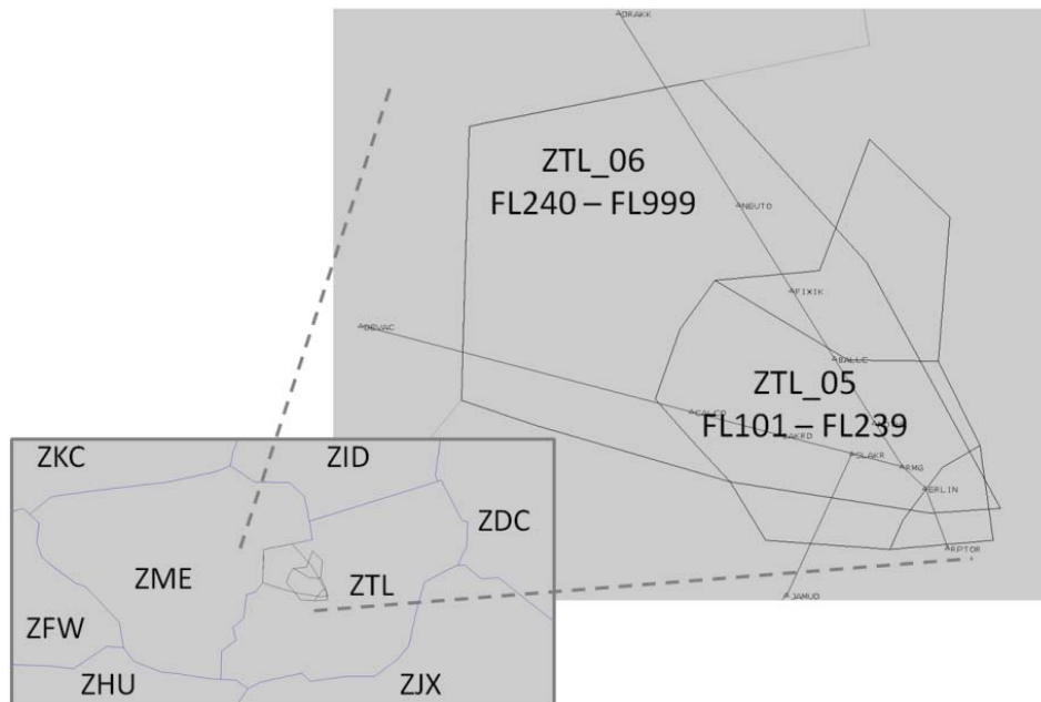
Figure 2. The two test sectors in the northwest portion of the Atlanta en route airspace.
