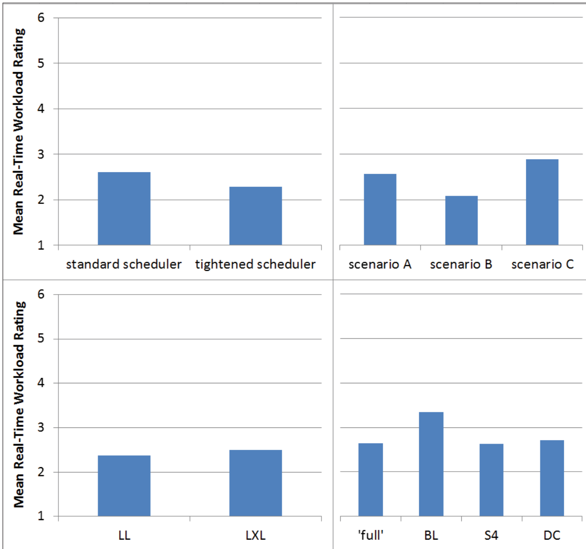
Figure 16. Controllers' average real-time workload rating, as reported in the exploratory analyses. A rating of 1 represents low workload, while a rating of 6 signifies high workload.
