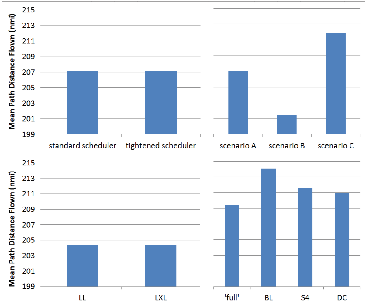
Figure 15. Average path distance flown, as reported in the exploratory analyses.
