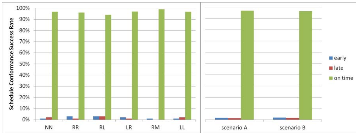
Figure 11. Percentage of aircraft delivered to the meter-fix either early, late, or on time, when compared across error conditions and traffic scenarios.
