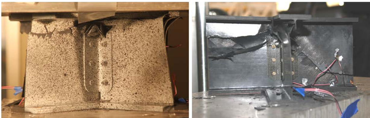
Figure 13. Post-test images of cruciform specimen following the 8-ft drop test.
