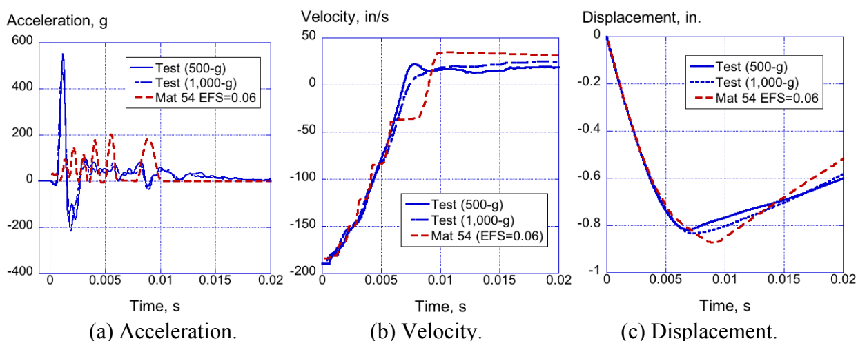
Figure 33. Experimental and Mat 54 analytical results for the I-beam 4-ft drop (velocity=189.6-in/s) with EFS=0.06.
