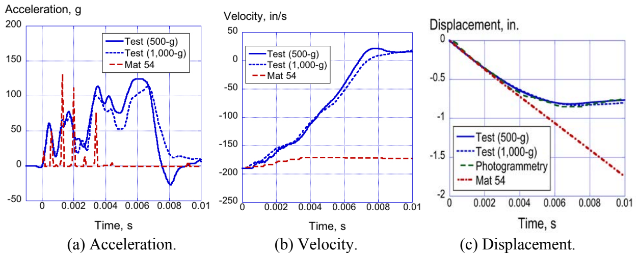
Figure 15. Experimental and Mat 54 analytical results for the I-beam crush test at 189.6-in/s.
