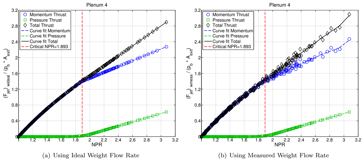
Figure 16. Comparison of the calculated non-dimensional momentum thrust, non-dimensional pressure thrust, and non-dimensional total thrust using (a) the ideal weight flow rate and (b) the measured weight flow rate.
