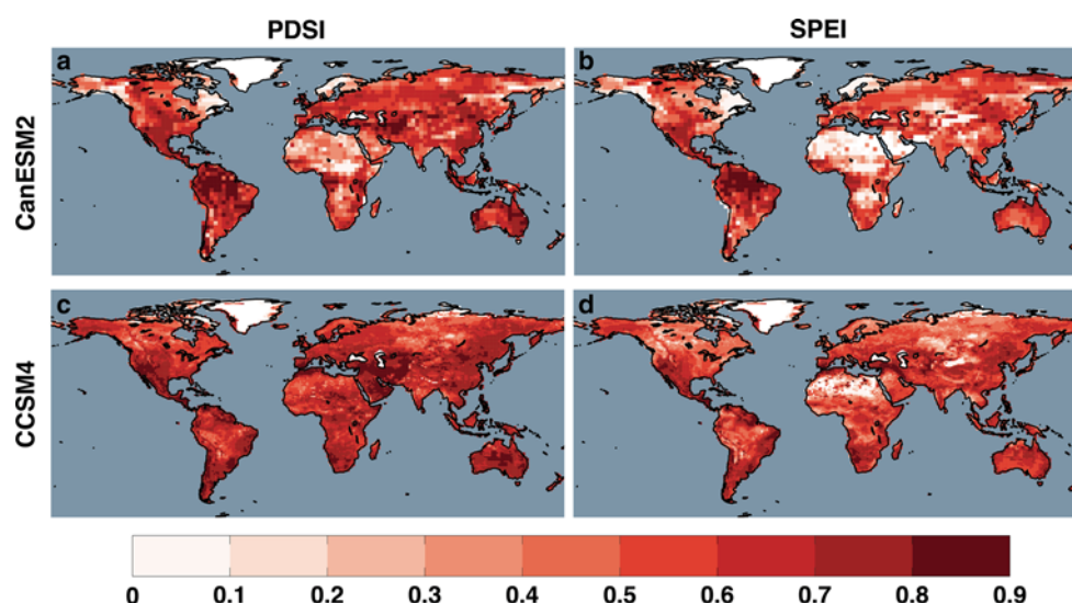
Fig. 1 Pearson's correlation coefficients calculated between PDSI (a,c) and SPEI (b,d) and annual average model soil moisture from the approximate top 30 cm of the soil column: CanESM2 (a,b) and CCSM4 (c,d). Maps represent average correlations across a five member ensemble for each model; the comparison interval is 1901–2009
