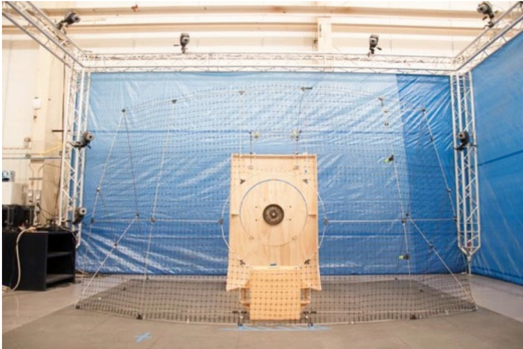
B-5. Phase 2 Mockup of Launch Vehicle Stage Adapter Wall Section with Hatch Opening, Connectors Requiring Tool Manipulation (right side) and Simulated LRU Equipment Shelf Attached to Plywood Structure
