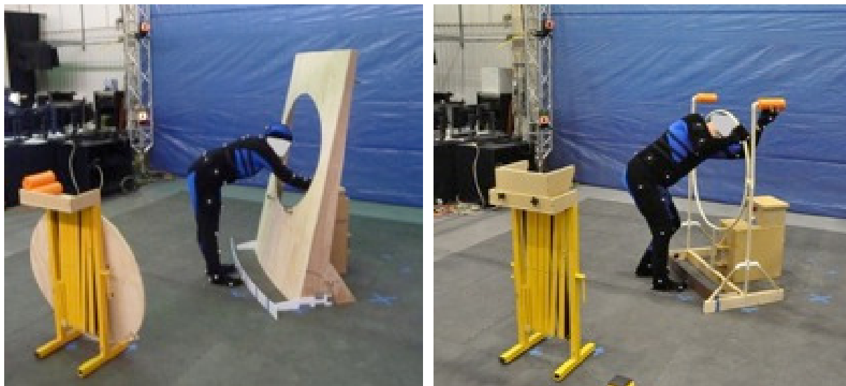
Figure 6.6-5. Sample Mockup Configurations with Participants Performing Subtasks during Phase 1
