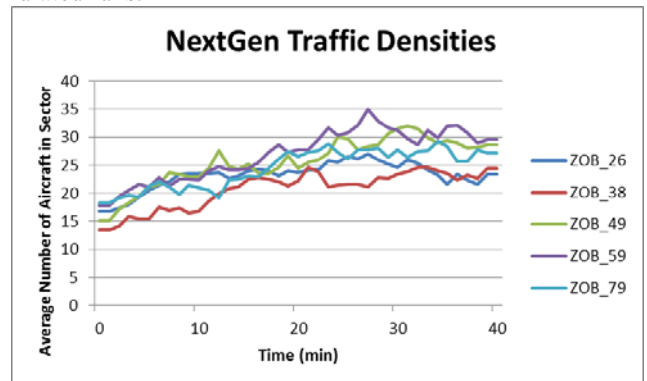
Figure 7. Average aircraft counts across all 6 runs per sector.
