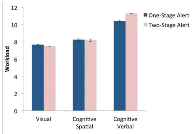
Figure 15. Predicted PF workload with one-stage and two-stage wake threat alerts (+/- 1 SE)
