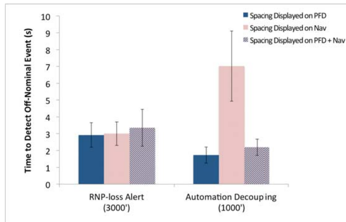
Figure 20. Predicted PF response time to detect RNP-loss alert and automation decoupling as a function of spacing information location (+/- 1 SE)
