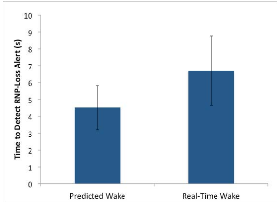
Figure 10. Predicted PF response times to RNP-loss alerts with static versus real-time wake displays (+/- 1 SE)
