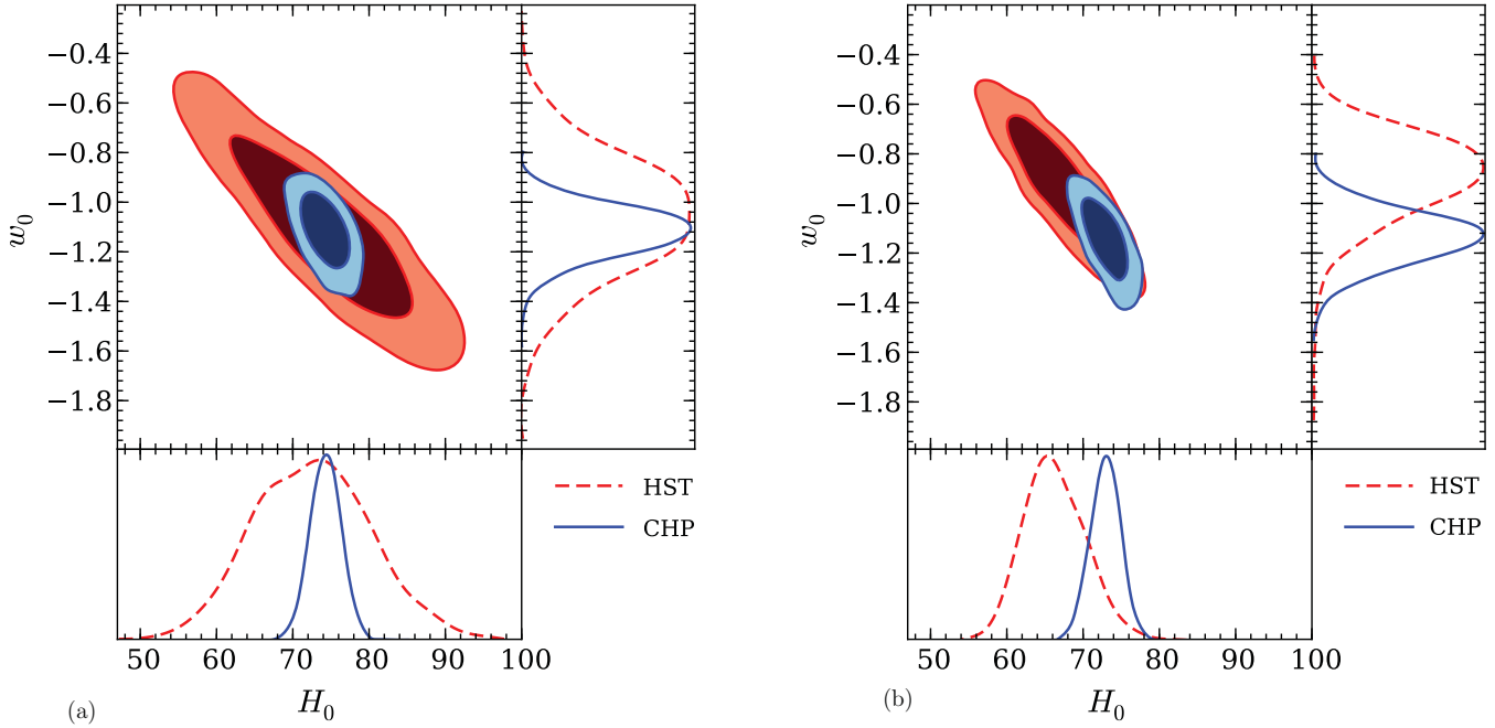
Figure 4. Two-dimensional confidence plots of the equation-of-state parameter w_0 and the Hubble constant H_0 using (a) the WMAP7 data alone and (b) WMAP7 and BAO data combined, and assuming \Omega_k = 0 , w_a = 0 , and N_{\text{eff}} = 3.046 . The red contours show the results using the prior from F01, while the blue contours show the results using the prior from this paper (labeled CHP). The right and bottom panels show the one-dimensional marginalized posterior probability distributions (PPDs) for w_0 and H_0 , respectively. The F01 PPD is plotted as red dashed lines, the CHP PPD is plotted as blue solid lines.
