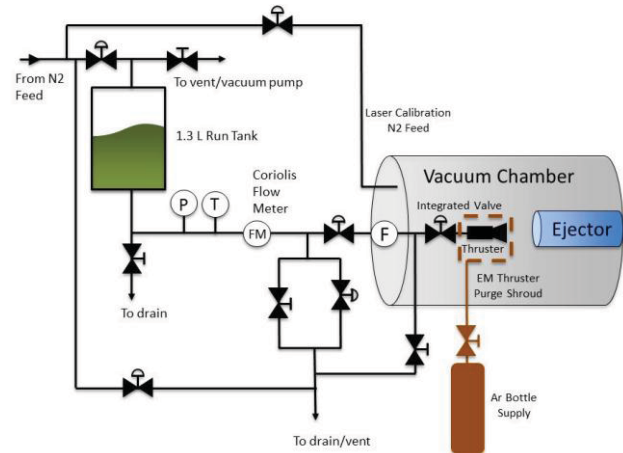
Figure 14: Green Propellant Flow System Diagram
