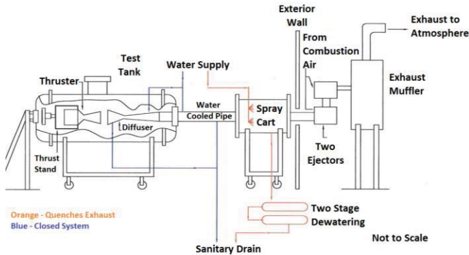
Figure 11: RCL-11 Schematic
