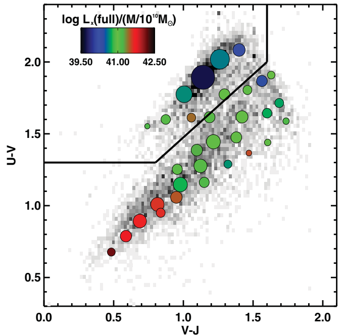
Figure 6. Rest-frame U - V vs. V - J color for each SED type, color-coded by full band (0.5–7 keV) normalized X-ray luminosity \text{erg s}^{-1} , corrected to the average redshift of the sample ( z = 0.95 ) using the best fit L_x - z relation, and scaled by bin size. The full NMBS sample with K -band S/N > 25 is shown in gray. Passive red galaxies (top left: bounded by the Williams et al. (2009) division separating quiescent and star-forming galaxies) have an average luminosity per stellar mass almost a dex lower than that of blue galaxies. (A color version of this figure is available in the online journal.)
