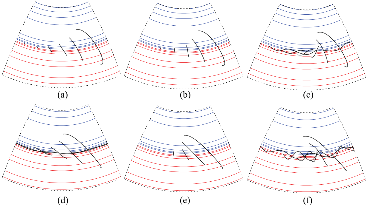
Fig. 8.— Competing effects of differential rotation and supergranular helicity injection with surface diffusion included. The plots show the results for differential rotation and surface diffusion only (left column); with helicity injected at a rate of \bar{\omega}_l = 1 \times 10^{-6} \text{ s}^{-1} (middle column); and with helicity injected at a rate of \bar{\omega}_l = 5 \times 10^{-6} \text{ s}^{-1} (right column). Elapsed times are 10 days (top row) and 20 days (bottom row). Line styles are the same as in Figure 6.
