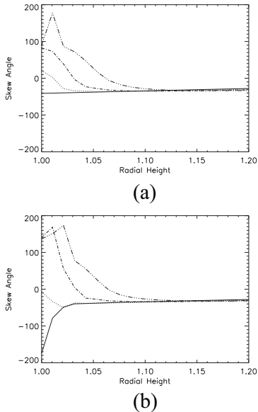
Fig. 7.— Skew angle \gamma versus radial height after 20 days for the cases of differential rotation and supergranular helicity injection (a) only and (b) in combination with surface diffusion. The various line styles denote different rates of helicity injection: \overline{\omega}_l = 0 \text{ s}^{-1} (solid), \overline{\omega}_l = 1 \times 10^{-6} \text{ s}^{-1} (dot), \overline{\omega}_l = 2.5 \times 10^{-6} \text{ s}^{-1} (dash-dot), and \overline{\omega}_l = 5 \times 10^{-6} \text{ s}^{-1} (dash-dot-dot-dot). Positive values indicate a dextral skew; negative values, sinistral skew.
