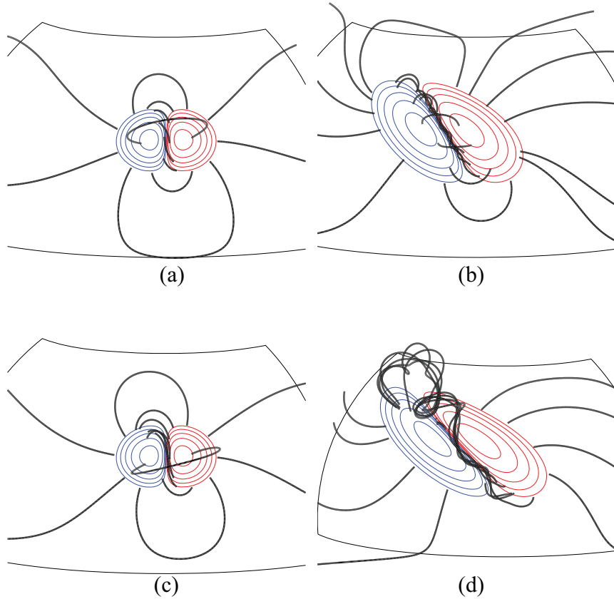
Fig. 3.— Evolution of an isolated bipole when (left column) helicity injection with vorticity \overline{\omega}_l = 1 \times 10^{-6} \text{ s}^{-1} is applied with no other surface flux transport processes, and (right column) surface flux transport processes are applied with no helicity injection. Elapsed times are 27 days (top row) and 54 days (bottom row). Line styles are the same as in Figure 2.
