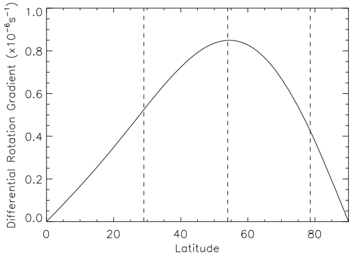
Fig. 1.— Differential rotation gradient, \omega_{dr} \equiv d\Omega/d\theta , versus latitude. Vertical dashed lines indicate the latitudes of the polarity inversion line in the axisymmetric cases described in §4.
