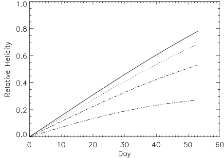
Fig. 9.— Relative magnetic helicity H_r for simulations with an east/west PIL at 54^\circ latitude when differential rotation and helicity injection only are applied (no surface diffusion). The various line styles denote different rates of helicity injection: \bar{\omega}_l = 0 \text{ s}^{-1} (solid), \bar{\omega}_l = 1 \times 10^{-6} \text{ s}^{-1} (dot), \bar{\omega}_l = 2.5 \times 10^{-6} \text{ s}^{-1} (dash-dot), and \bar{\omega}_l = 5 \times 10^{-6} \text{ s}^{-1} (dash-dot-dot-dot).
