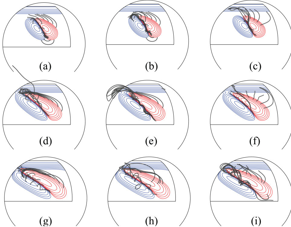
Fig. 12.— Interaction of a single magnetic bipole at 20^\circ latitude with the polar field in the declining phase of the solar cycle. Results are shown for full surface flux transport alone (left column) and in combination with supergranular helicity injection at rates of \bar{\omega}_l = 1 \times 10^{-6} \text{ s}^{-1} (middle column) and \bar{\omega}_l = 5 \times 10^{-6} \text{ s}^{-1} (right column). Elapsed times are 30 days (top row), 60 days (middle row), and 90 days (bottom row). Line styles are the same as in Figure 2.
