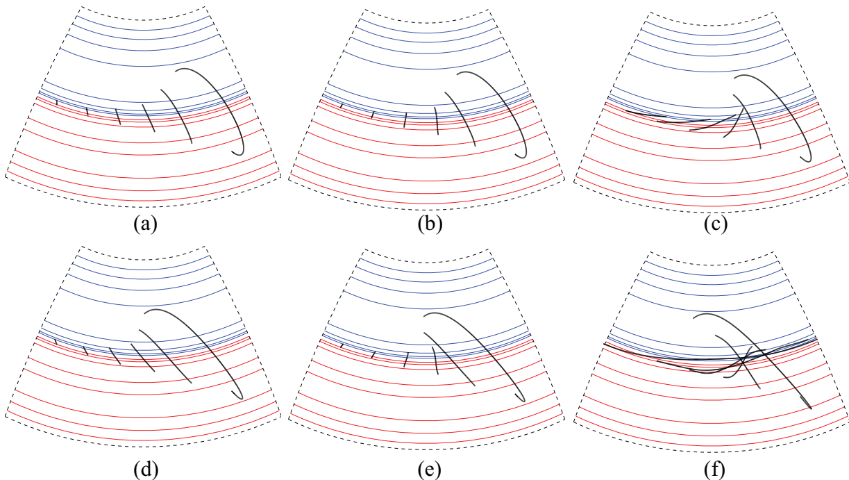
Fig. 6.— Competing effects of differential rotation and helicity injection (no surface diffusion). Results are shown for differential rotation alone (left column) and for differential rotation plus helicity injection at rates of \bar{\omega}_l = 1 \times 10^{-6} \text{ s}^{-1} (middle column) and \bar{\omega}_l = 5 \times 10^{-6} \text{ s}^{-1} (right column). Elapsed times are 10 days (top row) and 20 days (bottom row). Dashed lines indicate where the computational domain is truncated in the images; other line styles are the same as in Figure 2.
