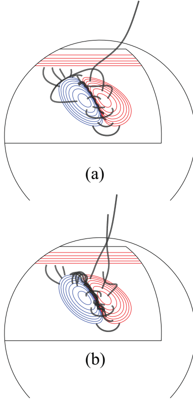
Fig. 11.— Interaction of a single magnetic bipole at 20^\circ latitude with the polar field in the rising phase of the solar cycle for full surface flux transport (a) alone and (b) with helicity injection at a rate of \bar{\omega}_l = 1 \times 10^{-6} \text{ s}^{-1} . Elapsed time is 27 days. Line styles are the same as in Figure 2.
