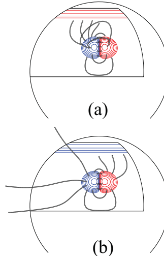
Fig. 10.— Initial conditions for a single bipole at 20^\circ latitude in the (a) rising and (b) declining phases of the solar cycle. Line styles are the same as in Figure 2.
