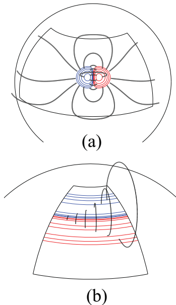
Fig. 2.— Initial conditions for (a) an isolated bipole at 25^\circ latitude and (b) an east/west PIL at 54^\circ latitude. Red/blue represents positive/negative flux; thick black lines are field lines; thin black lines demarcate the boundaries of the computational domain and the limb of the Sun.
