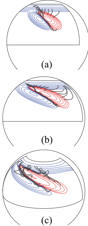
Fig. 13.— Interaction of a single magnetic bipole at 30^\circ latitude with the polar field in the declining phase of the solar cycle. Results are shown for full surface flux transport with supergranular helicity injection at a rate of \overline{\omega_l} = 5 \times 10^{-6} \text{ s}^{-1} . Elapsed times are (a) 30 days, (b) 60 days, and (c) 90 days. Line styles are the same as in Figure 2.
