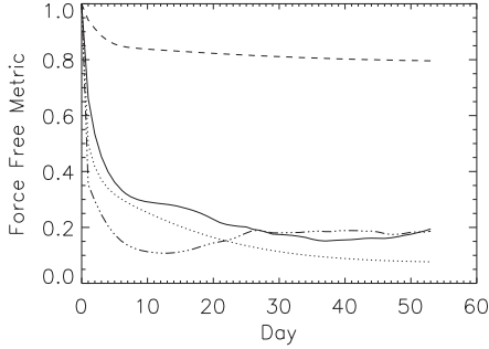
Fig. 5.— Force-free metric \sigma_j (Eq. 8) versus day of simulation for an isolated bipole. In all simulations, a radial outflow is applied at the upper boundary. Line styles are the same as in Figure 4.
