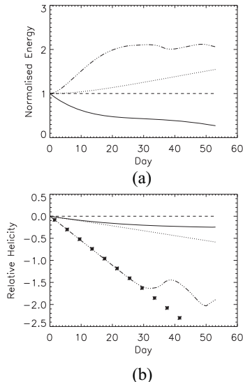
Fig. 4.— Normalised (a) magnetic energy E_m (Eq. 6) and (b) relative magnetic helicity H_r (Eq. 7) versus day of simulation for an isolated bipole. In all simulations a radial outflow is applied at the upper boundary. The various line styles denote: no photospheric boundary transport (dash); helicity injection at a rate of \bar{\omega}_l = 1 \times 10^{-6} \text{ s}^{-1} (dot) or \bar{\omega}_l = 5 \times 10^{-6} \text{ s}^{-1} (dash-dot-dot-dot); and standard surface flux transport without helicity injection (solid). In (b), the stars denote the results for a helicity injection rate of \bar{\omega}_l = 1 \times 10^{-6} \text{ s}^{-1} , scaled up by a factor of 5.
