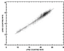
Figure 3. The correlation between LEND thermal neutron Doppler detectors counting rate ( y axis, counts per second) and LPNS counting rate from thermal neutron detector ( x axis, counts per second) using a 2^\circ \times 2^\circ regular mapping grid. The linear best fit is shown by dashed line.
