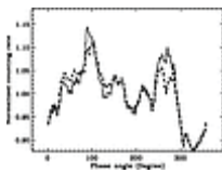
Figure 4. Orbital phase curves (see section 3 ) showing regional latitude variations of thermal neutron flux across the lunar surface. The x axis is the phase angle measured in degrees of arc from 0^\circ up 360^\circ , where 90^\circ corresponds to south pole and 270^\circ to the north pole. The y axis is the normalized counting rate of fast neutrons measured by different instruments. LEND data are shown by solid curve and LPNS data by dashed curve.
