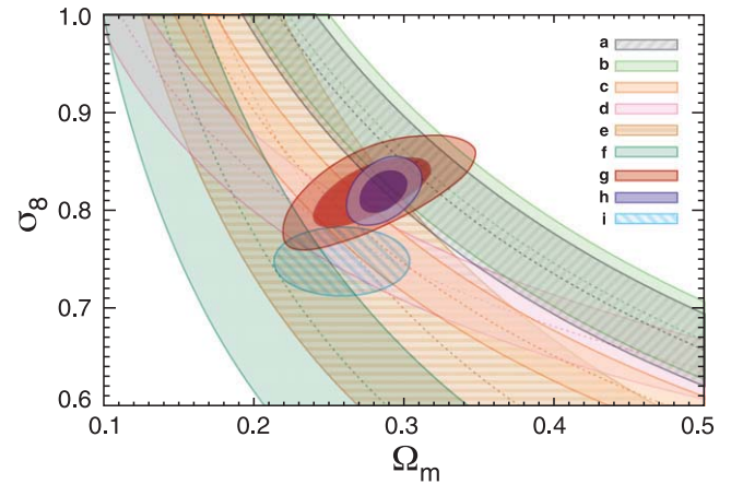
Figure 11. Compilation of the (\Omega_m, \sigma_8) constraints from large scale structure observations, discussed in Section 5, compared to the constraints obtained from CMB, BAO, and H_0 data. The various large scale structure probes do not separately constrain the two parameters, and have somewhat different degeneracy slopes among them, but these independent measurements are quite consistent. The following 1\sigma regions are plotted: (a) \sigma_8 \Omega_m^{0.5} = 0.465 \pm 0.026 from Tinker et al. (2012); (b) \sigma_8 (\Omega_m / 0.325)^{0.501} = 0.828 \pm 0.049 from Zu et al. (2012); (c) \sigma_8 (\Omega_m / 0.25)^{0.47} = 0.813 \pm 0.032 from Vikhlinin et al. (2009b); (d) \sigma_8 (\Omega_m / 0.25)^{0.3} = 0.785 \pm 0.037 from Benson et al. (2013); (e) \sigma_8 (\Omega_m / 0.3)^{0.67} = 0.70^{+0.11}_{-0.14} from Semboloni et al. (2011); (f) \sigma_8 \Omega_m^{0.7} = 0.252^{+0.032}_{-0.052} from Lin et al. (2012); (g) WMAP only; (h) WMAP+eCMB+BAO+H_0 ; (i) ellipse whose major and minor axes are given by \Omega_m = 0.259 \pm 0.045 and \sigma_8 = 0.748 \pm 0.035 from Hudson & Turnbull (2012).
