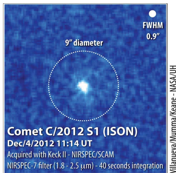
Figure 2: Image acquired for comet C/2012 S1 (ISON) on December 4, 2012 from the Keck II observatory. The GBT beam size at 89 GHz ( \sim 9'' ) is shown for comparison. Molecular emission for comet ISON will be monitored from a number of facilities through perihelion.
