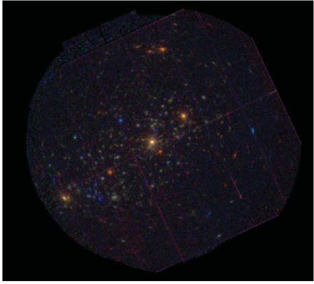
Fig. 7. Same as Fig. 1, but for IC 2944/2948. The yellow source at the field's center is HD 101205. The color version of this figure is available online.
