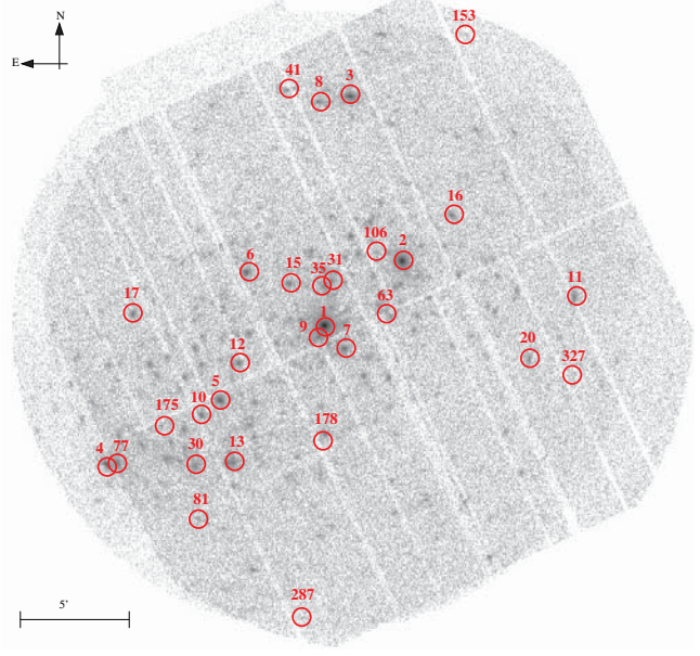
Fig. 7. Same as Fig. 1, but for IC 2944/2948. The yellow source at the field's center is HD 101205. The color version of this figure is available online.
