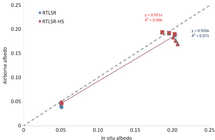
Figure 4. Results of the albedo test carried out in the corn ( circles ), wheat ( squares ), and barley ( triangles ) fields.
