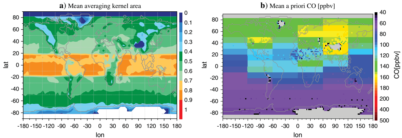
Figure 5. (a) 2005–2008 annual mean averaging kernel area ( ka ) and (b) mean a priori for TES CO retrievals at about 800 hPa.
