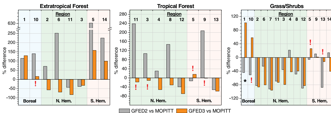
Figure 12. GFED2 and GFED3 versus MOPITT 2005–2008 annual mean CO emissions per MODIS fire count for the 14 GFED regions and the three basic vegetation types. GFED3 vs MOPITT differences are statistically significant within 5% ( p=0.05 ), except for those indicated with (*) = low significance (10%) and (!) = statistically insignificant.
