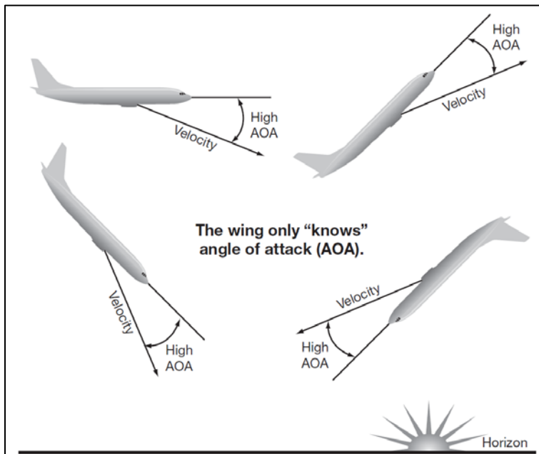
Figure 4: Different Pitch Attitudes and Stall AoA (Upset Recovery Industry Team, 2008)
