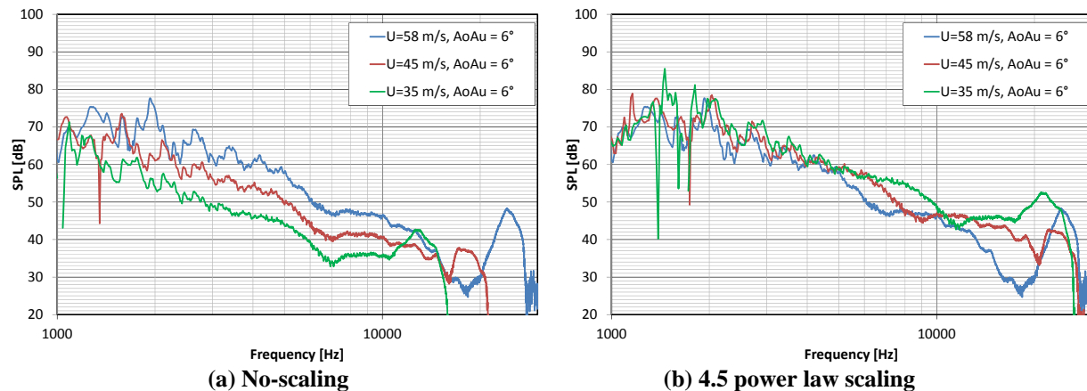
Figure 30. Comparison of microphone phased-array based acoustic spectra obtained by integration of noise source maps within SD3 at different free-stream velocities ( \alpha_{ti} = 6^\circ , spectral bin width = 10 Hz).
