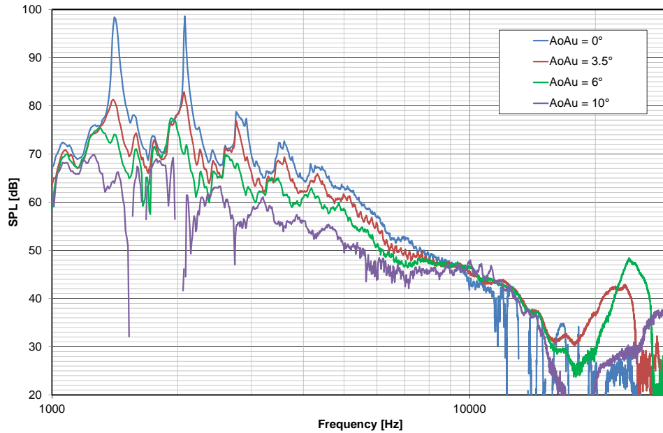
Figure 22. Acoustic spectra obtained by integrating noise source maps within SD3 at selected angles of attack (spectral bin width = 10 Hz).
