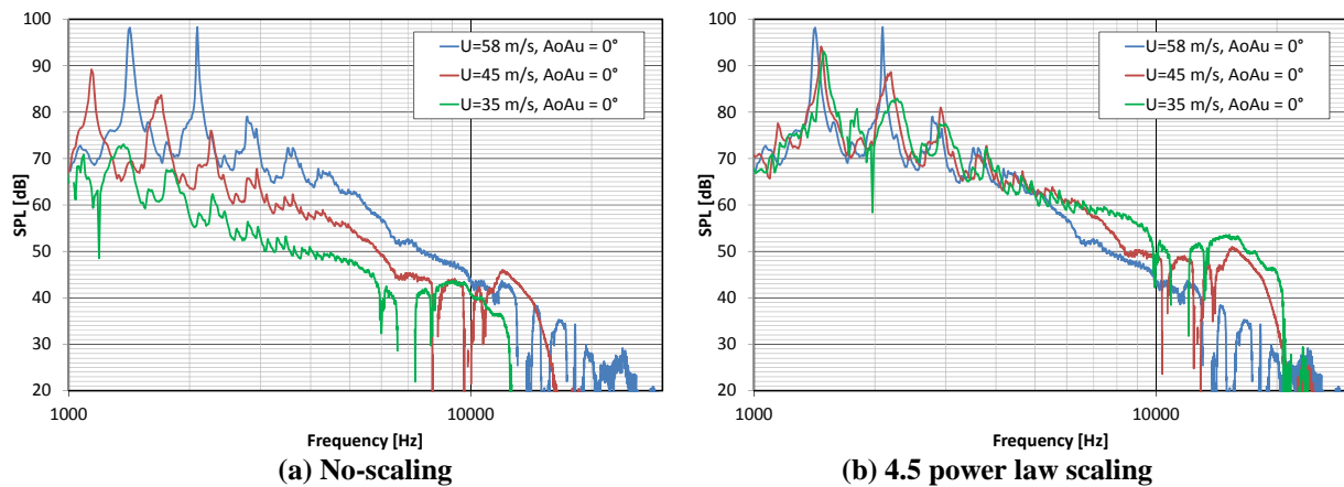
Figure 29. Comparison of microphone phased-array based acoustic spectra obtained by integration of noise source maps within SD3 at different free-stream velocities at \alpha_{ti} = 0^\circ (spectral bin width = 10 Hz).
