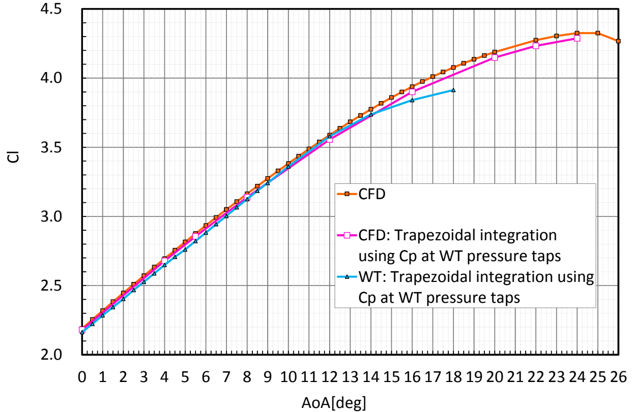
Figure 17. Comparisons of C_l - \alpha curves based on two-dimensional steady-state RANS CFD and wind tunnel measurement.
