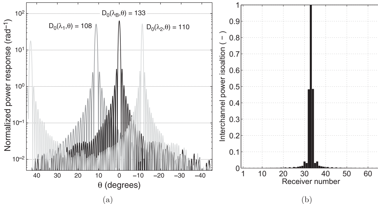
Fig. 6: Design B angular response. (a) The emitter antenna array’s angular power response is normalized by the total radiated power and plotted for the three stigmatic wavelengths. The directivity D_0(\lambda, \theta) is the peak angular response of the array and is indicated on the plot. (b) Power isolation between the receiver channels computed for \lambda_o \sim 560 \mu\text{m} , where the power in each channel is normalized to the power in the central channel.
