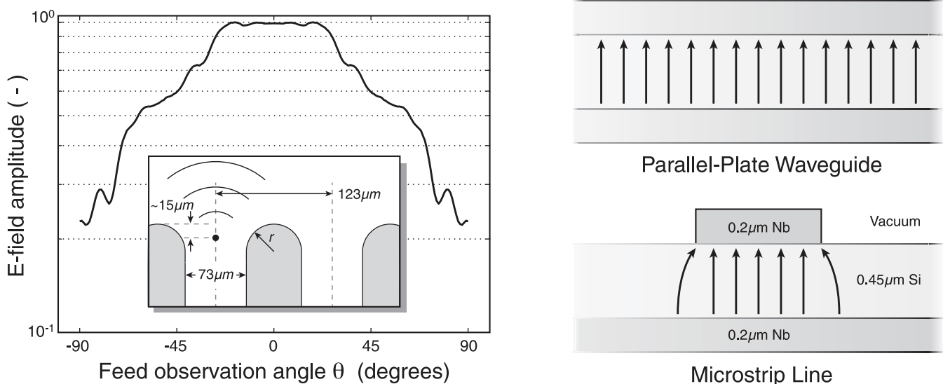
Fig. 4: (Left) The computed feed horn angular response at 430 GHz. The response of an emitting feed (aperture size 73 \mu\text{m} ) is evaluated in the far field ( \|\mathbf{r}\| \sim 6\lambda = 438 \mu\text{m} ) and normalized to the magnitude of the E field at zero degrees. The feed array geometry is provided in the figure insert. The feeds phase center is indicated by a black filled circle. (Right) Cross section of the parallel-plate waveguide (upper) and microstrip (lower) transmission line geometries. The electric field is depicted with arrows to indicate the dominant modal symmetry. An adiabatic transition serves as a mode converter between these modes and defines the feed’s angular response in the multimode power combined region.
