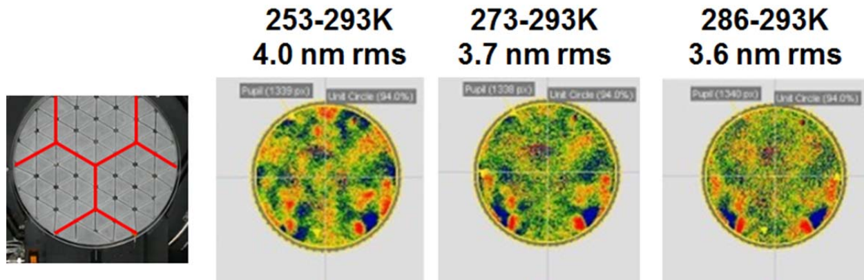
Figure 20 – The difference maps between ambient and temperatures down to 253K are shown. Very small changes were observed and were driven by the non-kinematic mount system.
